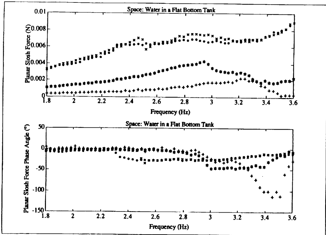
Uncoupled Test with Distilled Water as Test Fluid in a 3.1 cm Flat Bottom Cylindrical Tank . Planar Slosh Force.
