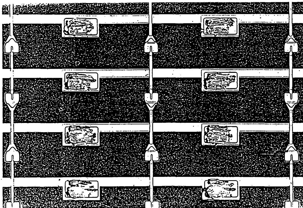
Figure 4: Photograph of a small section of the beam control array. Unit cell dimensions are 300 \mu\text{m} \times 120 \mu\text{m} . The vertical strips serve as the "antenna" elements, while the horizontal strips provide bias voltage to the diodes. The marks on the large rectangular test pads are from automated device probing.
