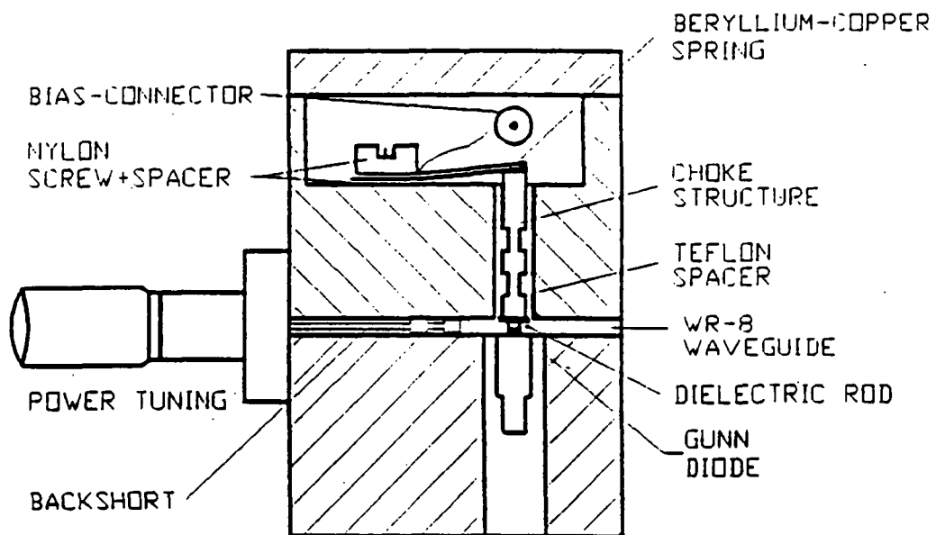
Fig. 5: GUNN-OSCILLATOR
