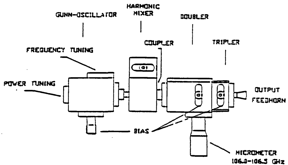
Fig. 4: LOCAL OSCILLATOR
