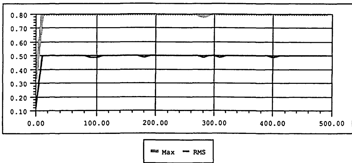
Figure 11b - Test Case 2, Max VS RMS Error
