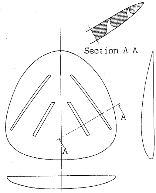
Figure 3.- Slotted low-aspect-ratio airfoil. b^2/S = 1.27
