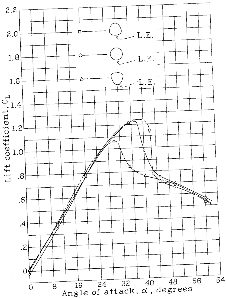
Figure 10.- Effect of plan form on lift coefficient. Flat plate airfoils.
