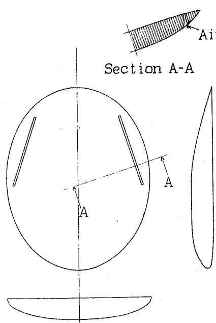
Figure 2.- Slotted low-aspect-ratio airfoil. b^2/S = 1
