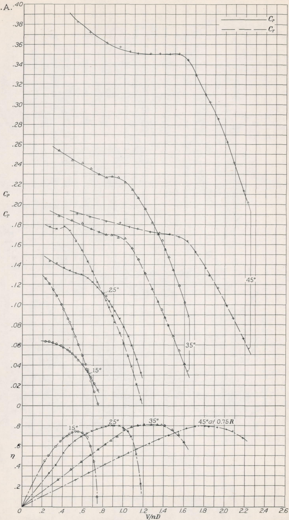
Figure 6.- Power, thrust, and efficiency. 4-blade right-hand propeller.
