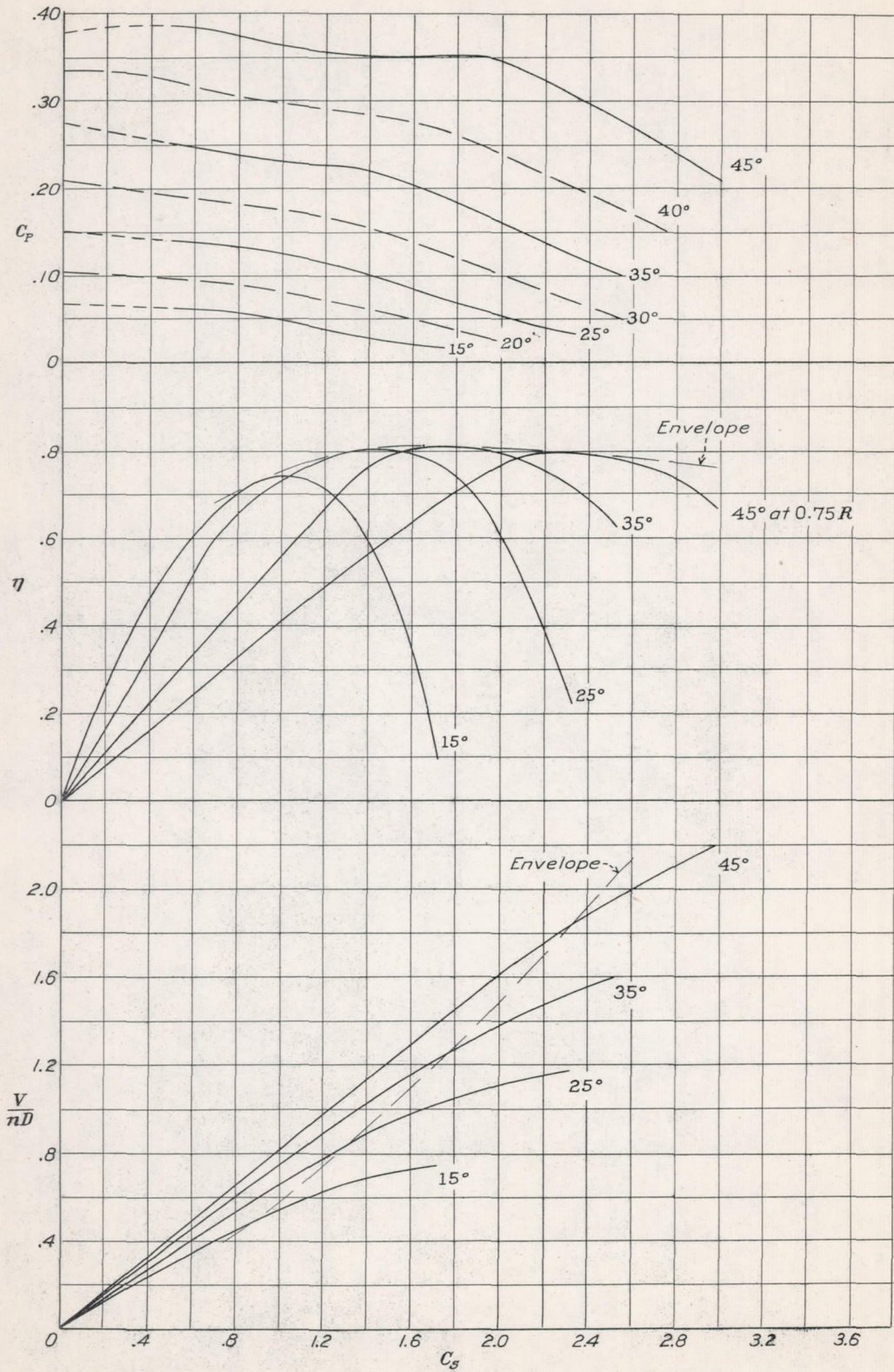
Figure 10.- Working chart. 4-blade right-hand propeller.
