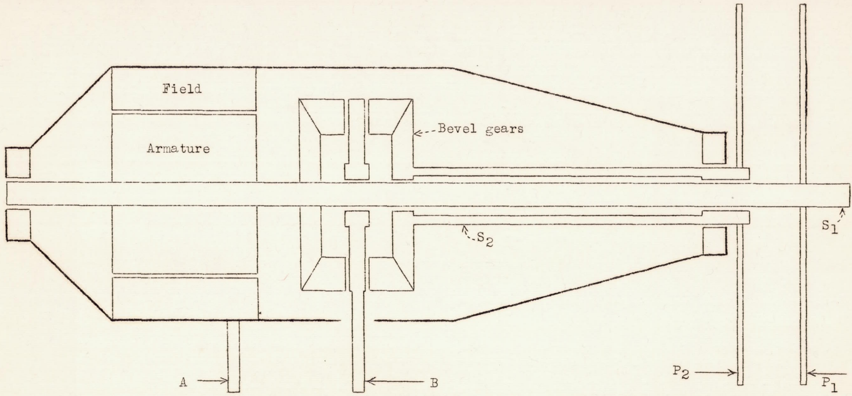
Figure 1.- Schematic section of propeller dynamometer.
