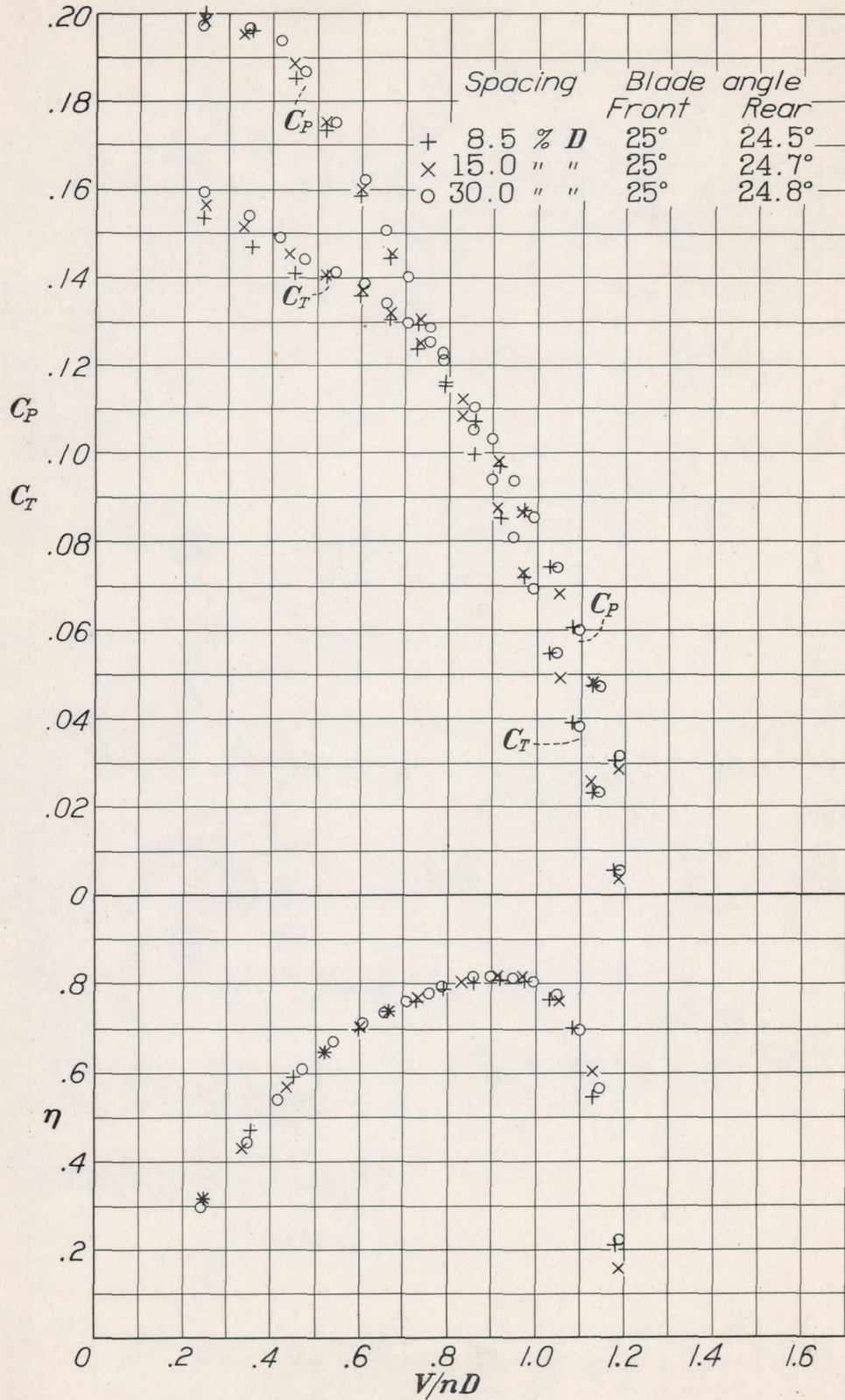
Figure 8.- Power, thrust, and efficiency. 2-blade tandem R.H. (front) and L.H. (rear) propellers with 25° blade angle and various axial spacings.
