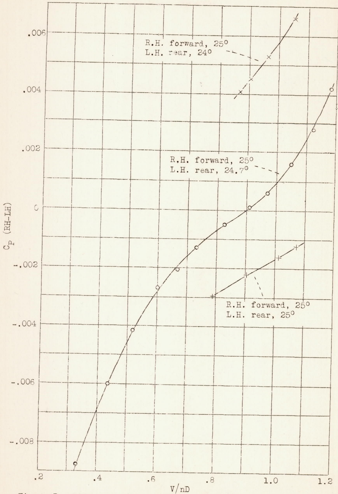
Figure 3.- Difference in power coefficients as affected by change in rear propeller blade-angle setting.
