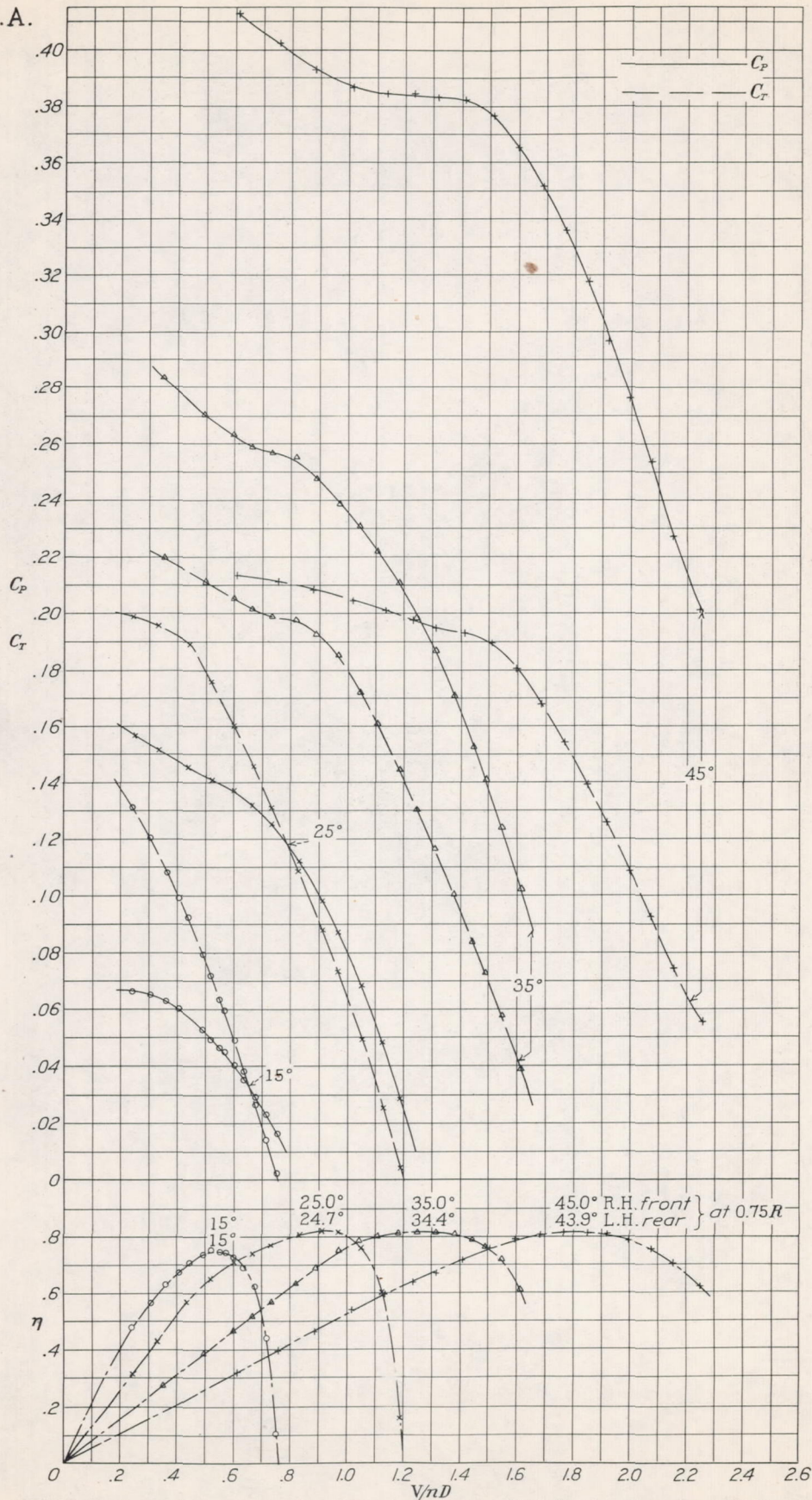
Figure 7.- Power, thrust, and efficiency. 2-blade tandem R.H. (forward) and L.H. (rear) propellers with 15% diameter spacing.
