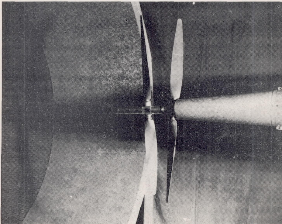
Figure 2.- Forward end of propeller dynamometer with tandem propellers at 15 percent diameter spacing.
