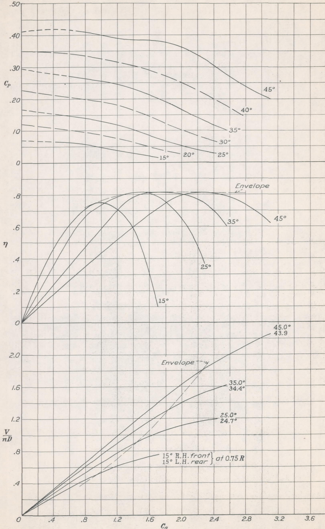
Figure 11.- Working chart. 2-blade R.H. (front) and L.H. (rear) propeller with 15 percent diameter spacing
