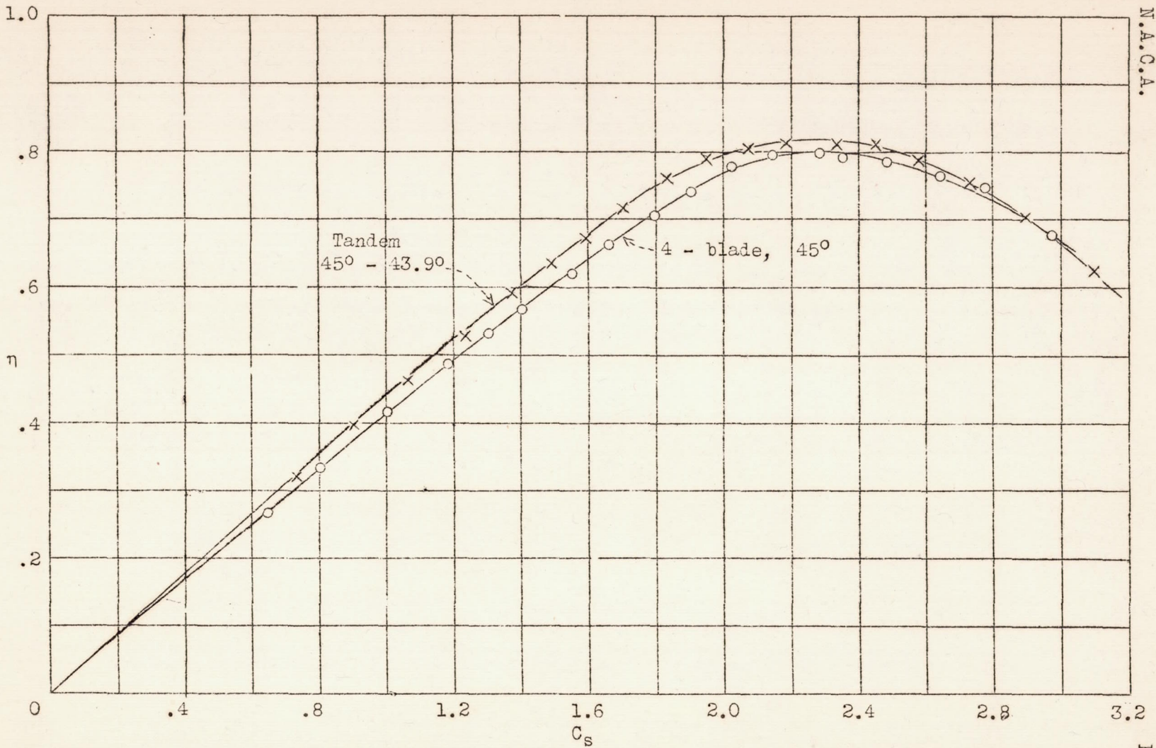
Figure 12.- Comparison of efficiency for 45° 4-blade propellers and 45° - 43.9° tandem propellers at same values of C_s .
