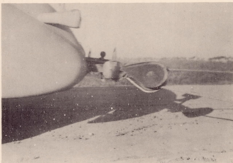
Figure 7.- Car pulley for pulley tow.
