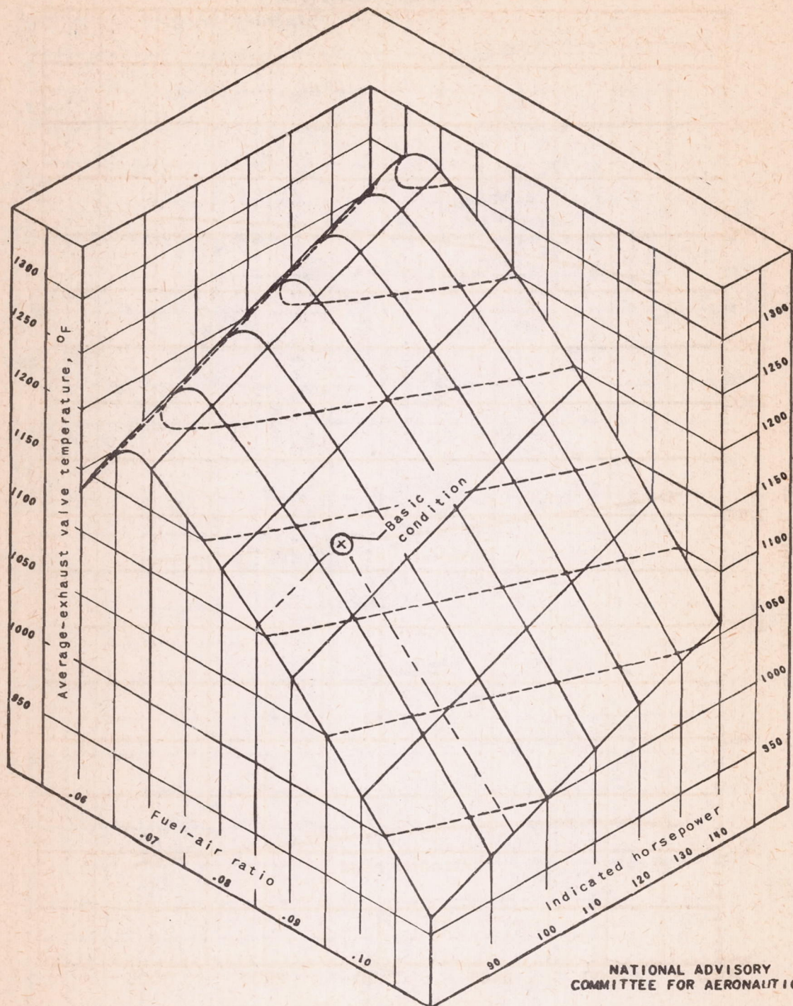
Figure 12. - Three-dimensional plot showing average valve temperature as function of indicated horsepower and fuel-air ratio. Spark advance; inlet, 28^{\circ} B.T.C.; exhaust, 34^{\circ} B.T.C.; mixture temperature, 200^{\circ} F; outlet coolant temperature, 250^{\circ} F; coolant flow, 105 gallons per minute; exhaust pressure, 30 inches mercury absolute; compression ratio, 6.65; fuel, 28-R.
