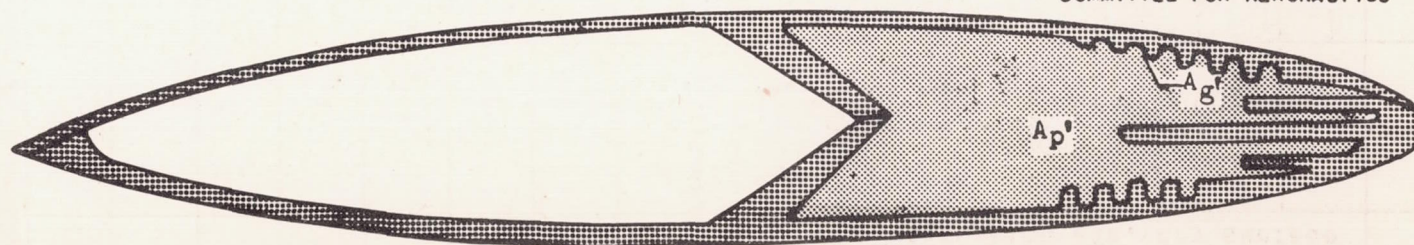
(c) Modification 2: Cross-sectional flow area ratio, A_p/A_p' = 1.5 ; internal heat-transfer area ratio, A_g'/A_g = 2.5 .
