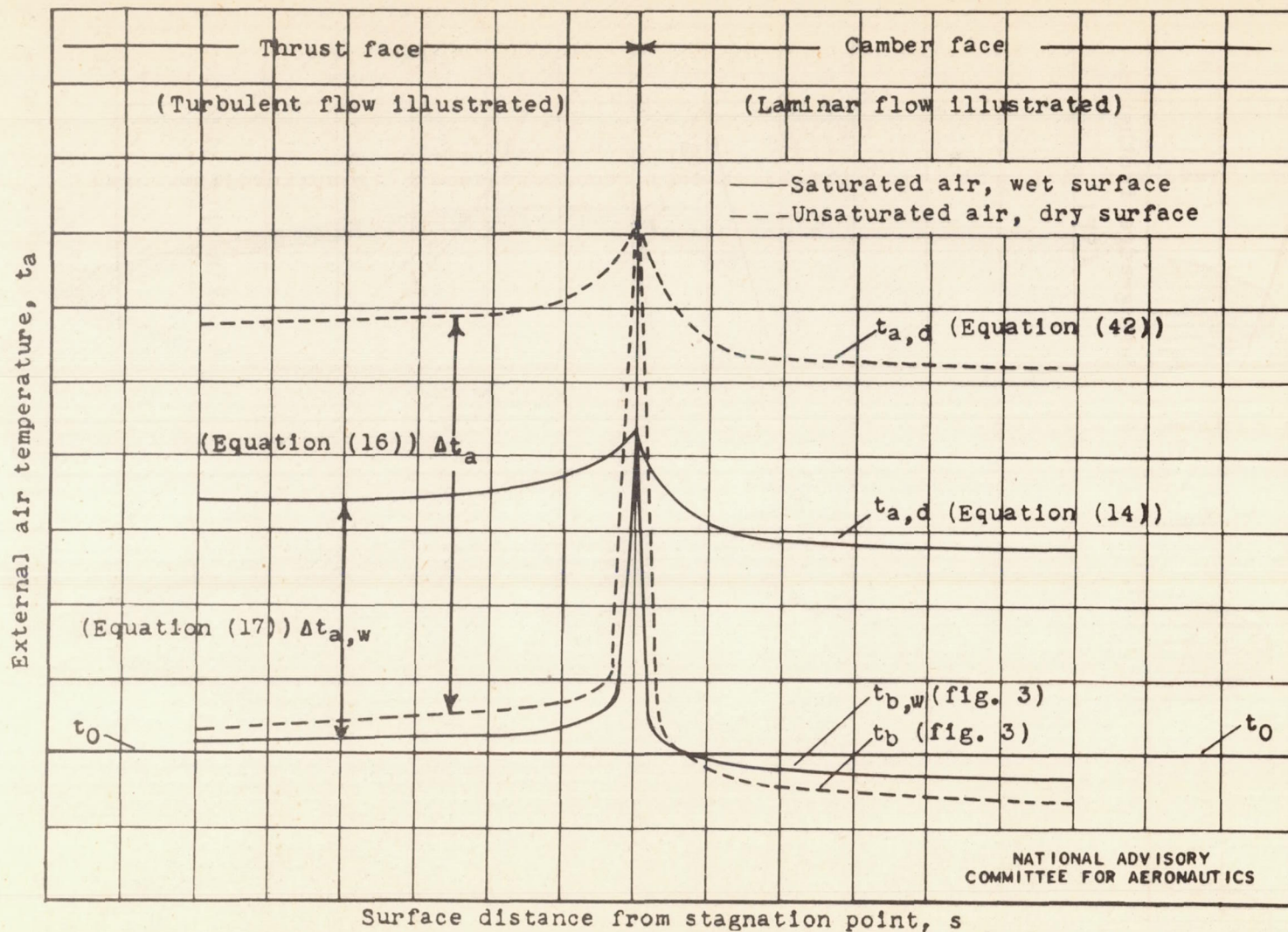
Figure 13. - Diagram of typical chordwise variation of heat-transfer datum temperature.
