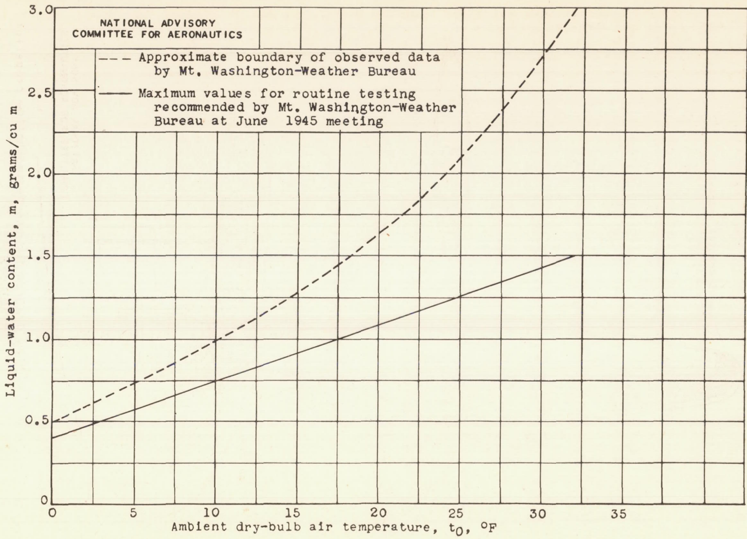
Figure 2. - Variation of liquid-water content with temperature.
