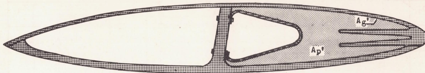
(b) Modification 1: Cross-sectional flow area ratio, A_p/A_p' = 2 ; internal heat-transfer area ratio, A_g'/A_g = 2 .
