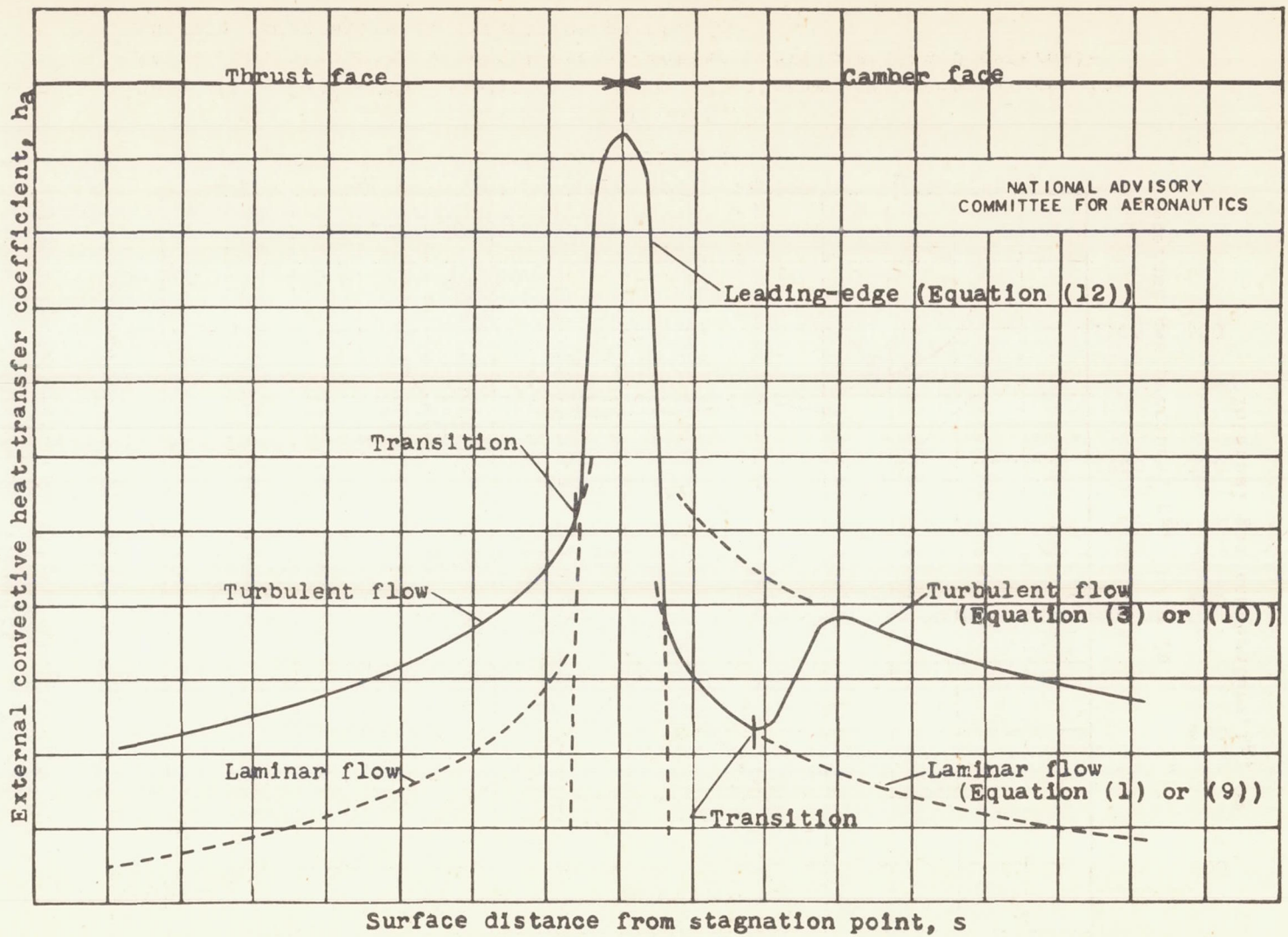
Figure 11. - Diagram of typical chordwise variation of external heat-transfer coefficient over propeller blade.
