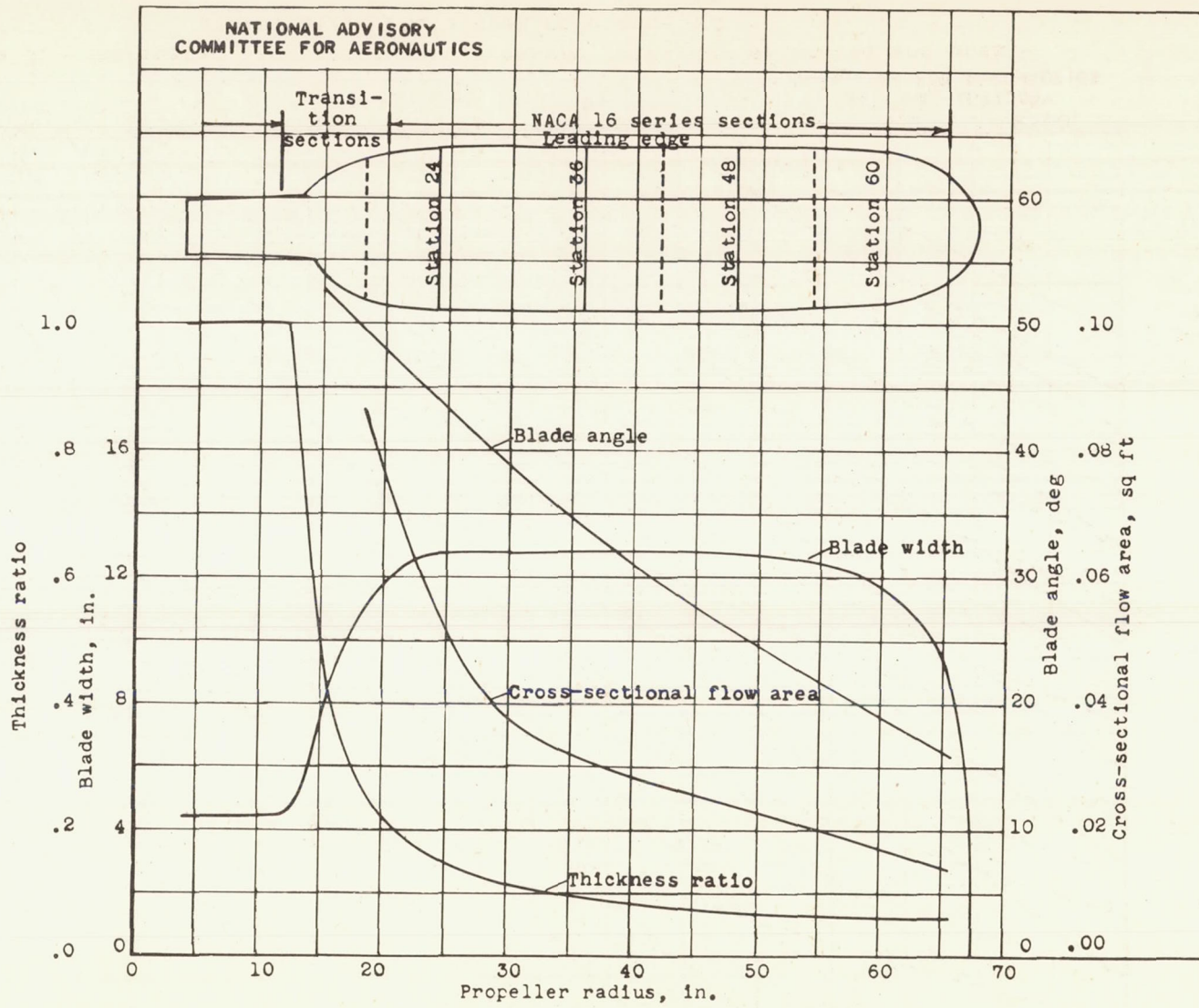
Figure 4. - Propeller-blade-form characteristics.
