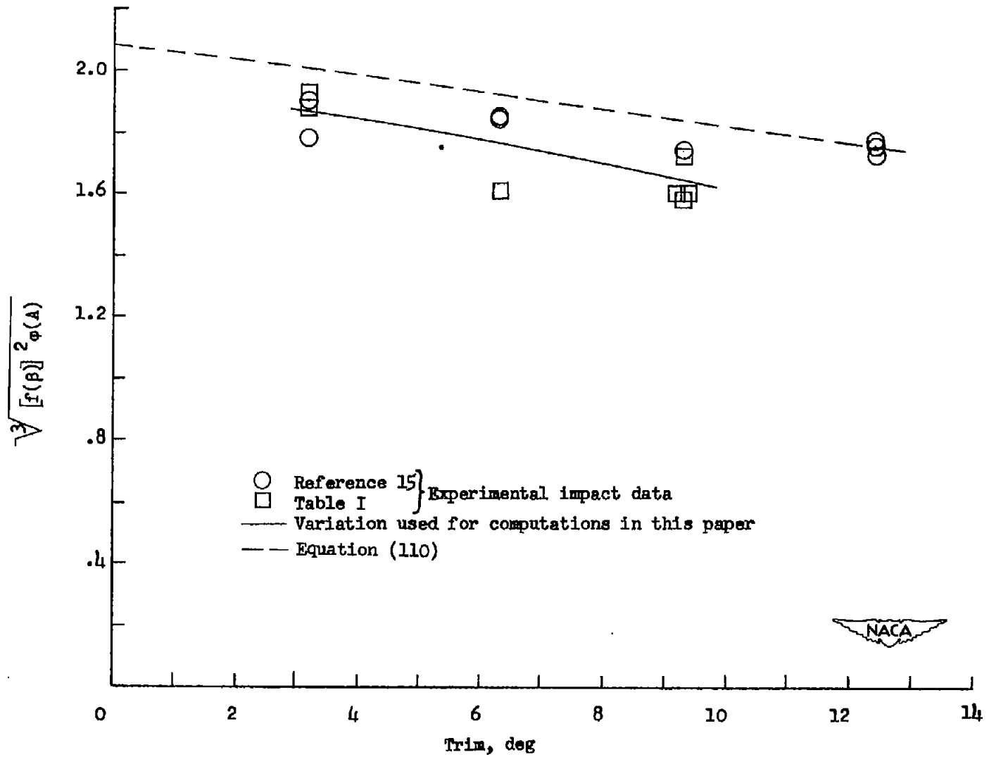
Figure 24.- Experimental variation of the dead-rise-aspect-ratio function with trim for an angle of dead rise of 22.5°.
