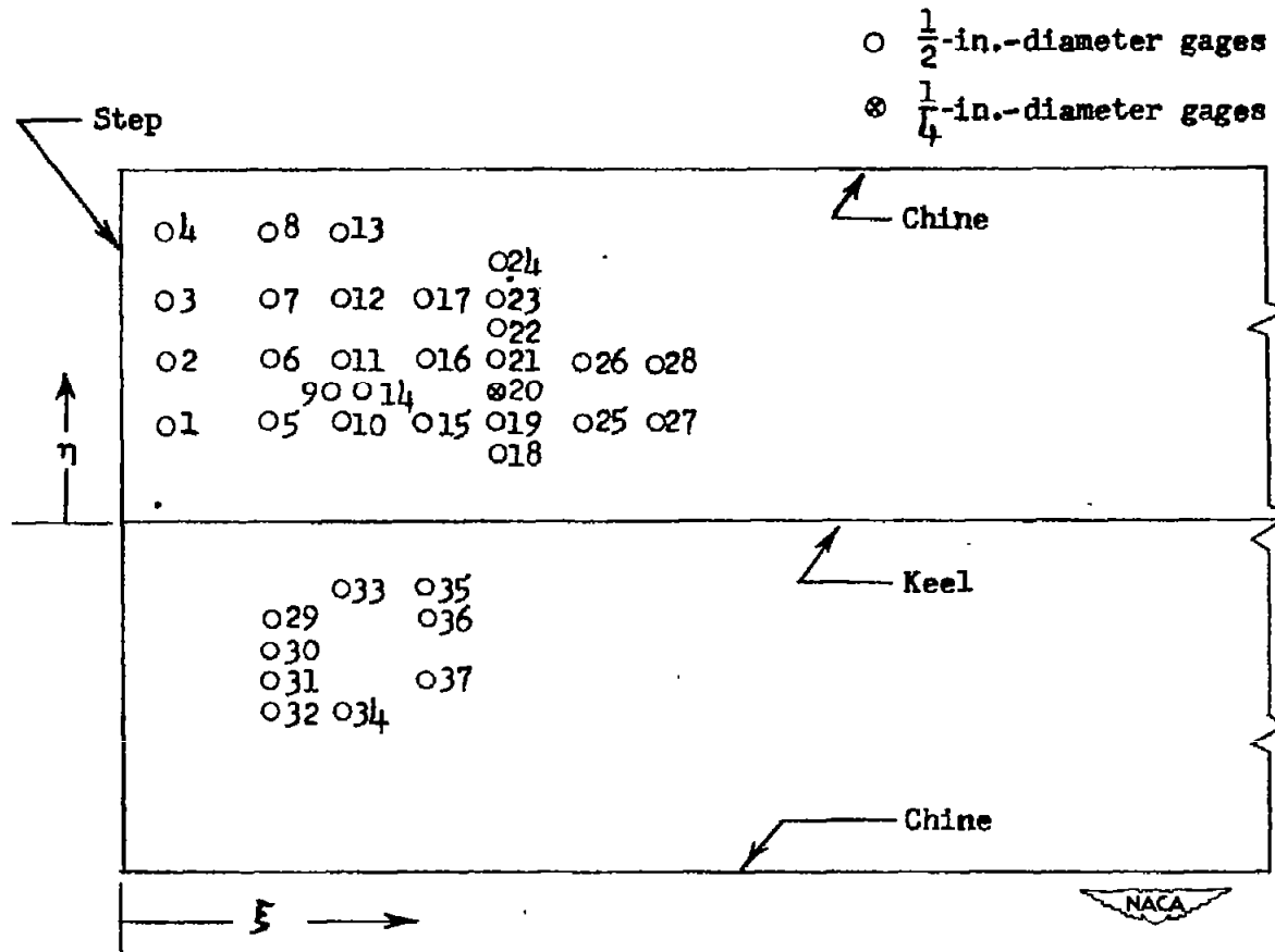
Figure 39.- Location of pressure gages in float bottom.
