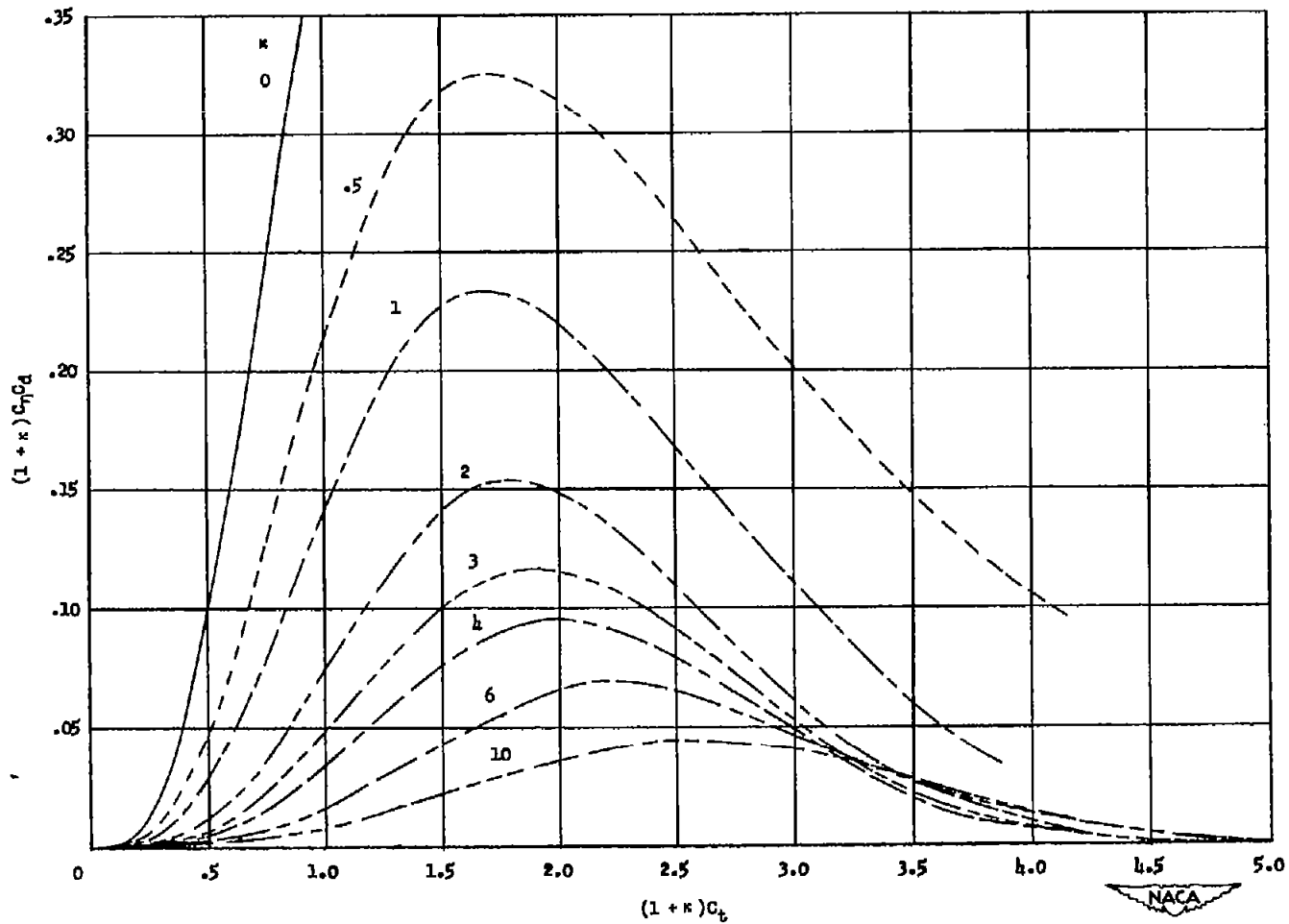
Figure 14.- Theoretical variation of the quantity C_{\eta}C_d with the time coefficient for various values of approach parameter for a non-chine-immersed wedge. (Ordinates and abscissas have been multiplied by the factor 1 + \kappa to facilitate interpolation.)
