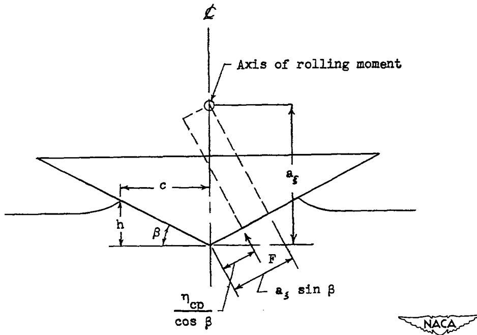
Figure 4.- Geometric relations for a straight-sided wedge.
