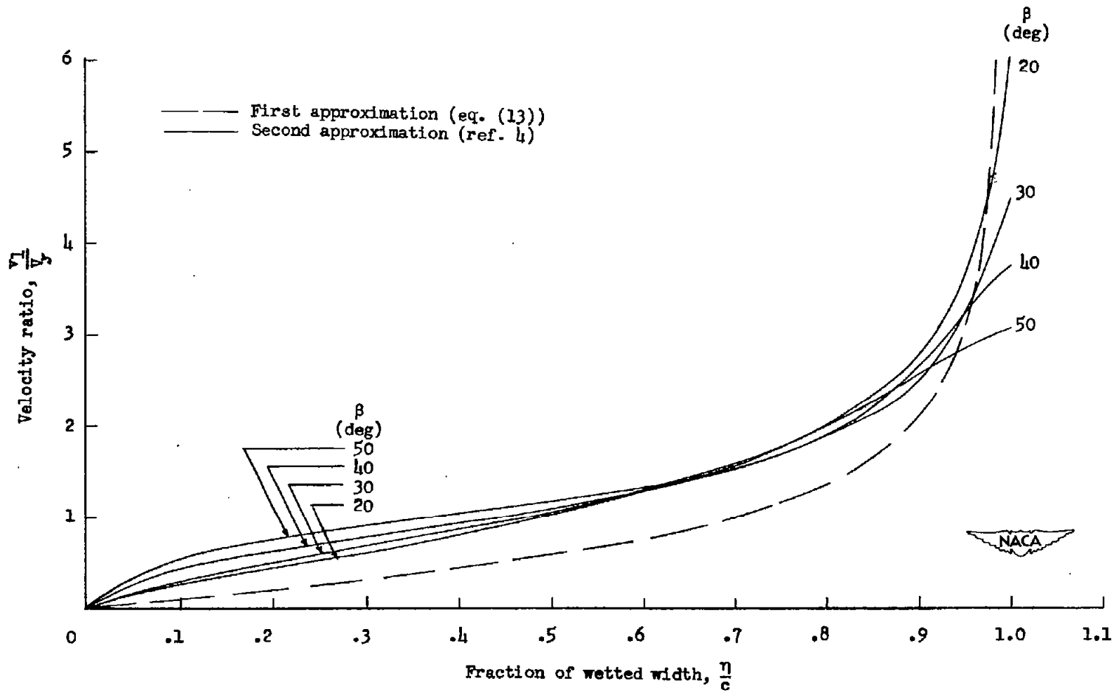
Figure 5.- Variation of the velocity ratio v_1/v_y on the side of a straight-sided two-dimensional wedge.
