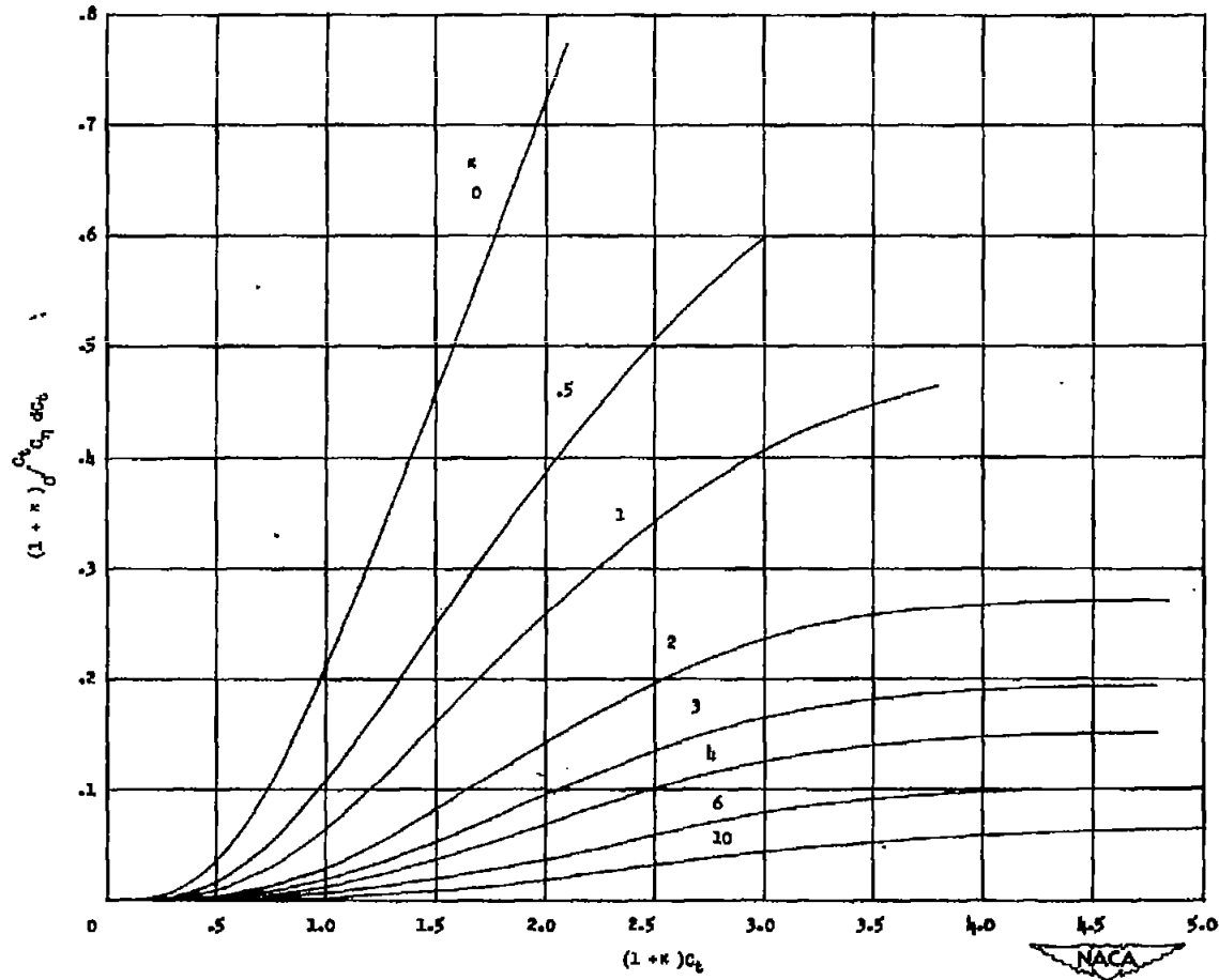
Figure 20.- Theoretical variation of the quantity (1 + \kappa) \int_0^{Ct} c_\eta dCt with the time coefficient for various values of approach parameter for a non-chine-immersed wedge. (The abscissa has been multiplied by 1 + \kappa to permit use of this curve with figs. 11 and 14.)
