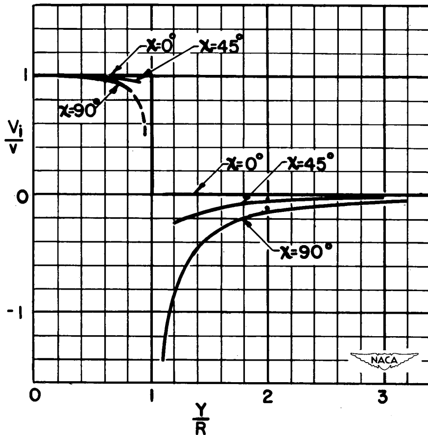
Figure 6.- Induced velocity distributions along Y-axis.
