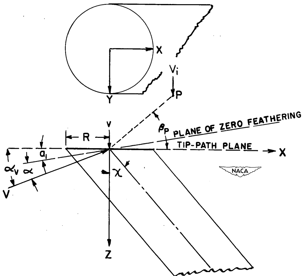
Figure 2.- Geometry of wake.
