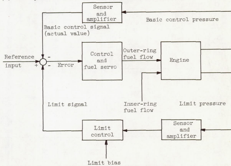
(b) Basic pressure-ratio control loop with limit loop.
