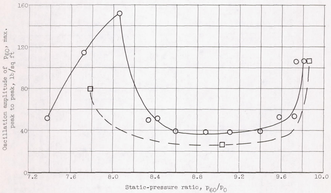
Figure 28. - Concluded. System stability at various pressure ratios.
