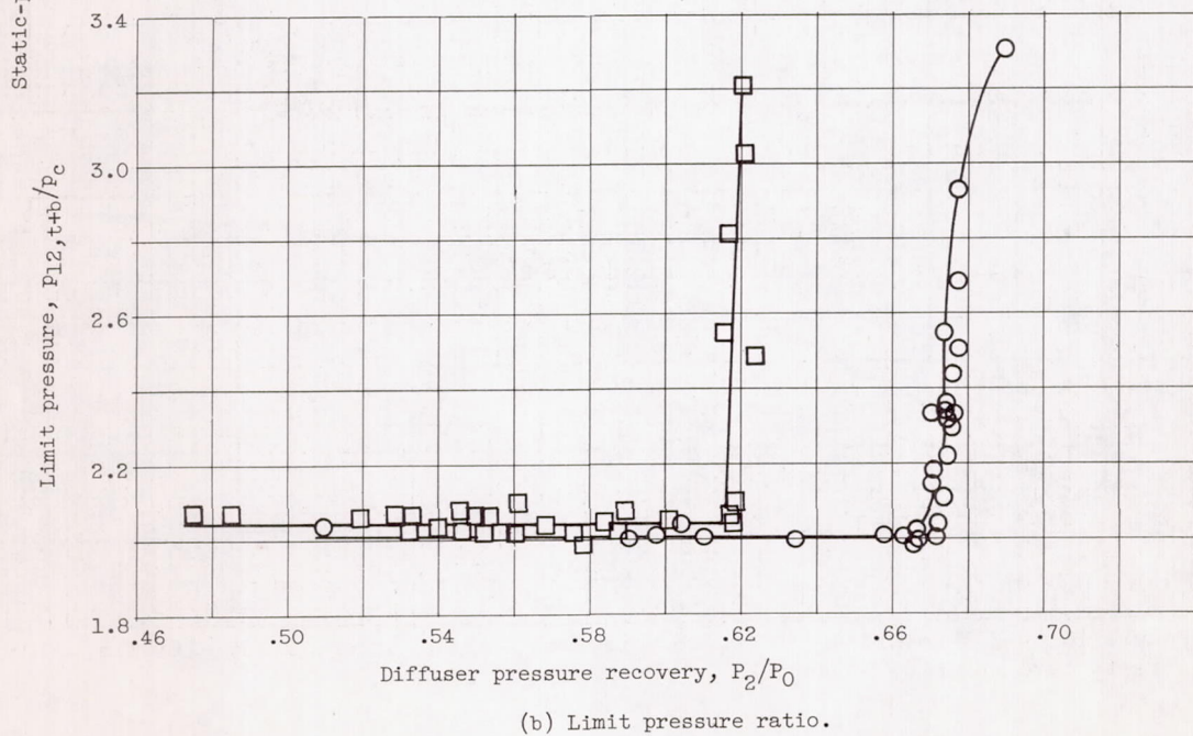
Figure 9. - Ratio of basic control and limit pressure to reference pressure as function of diffuser recovery at zero angle of attack.
