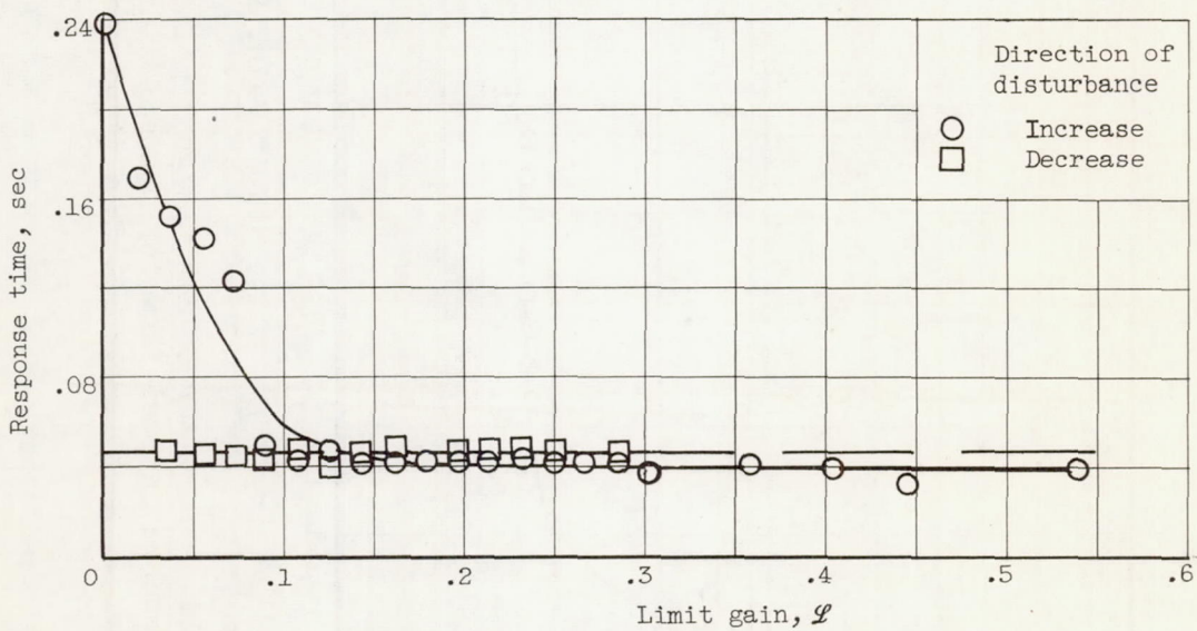
(a) Mach number, 2.35; loop gain, 0.503; fuel flow step size, \pm 0.26 pound per second; control pressure ratio p_{60}/p_0 , 8.21.
