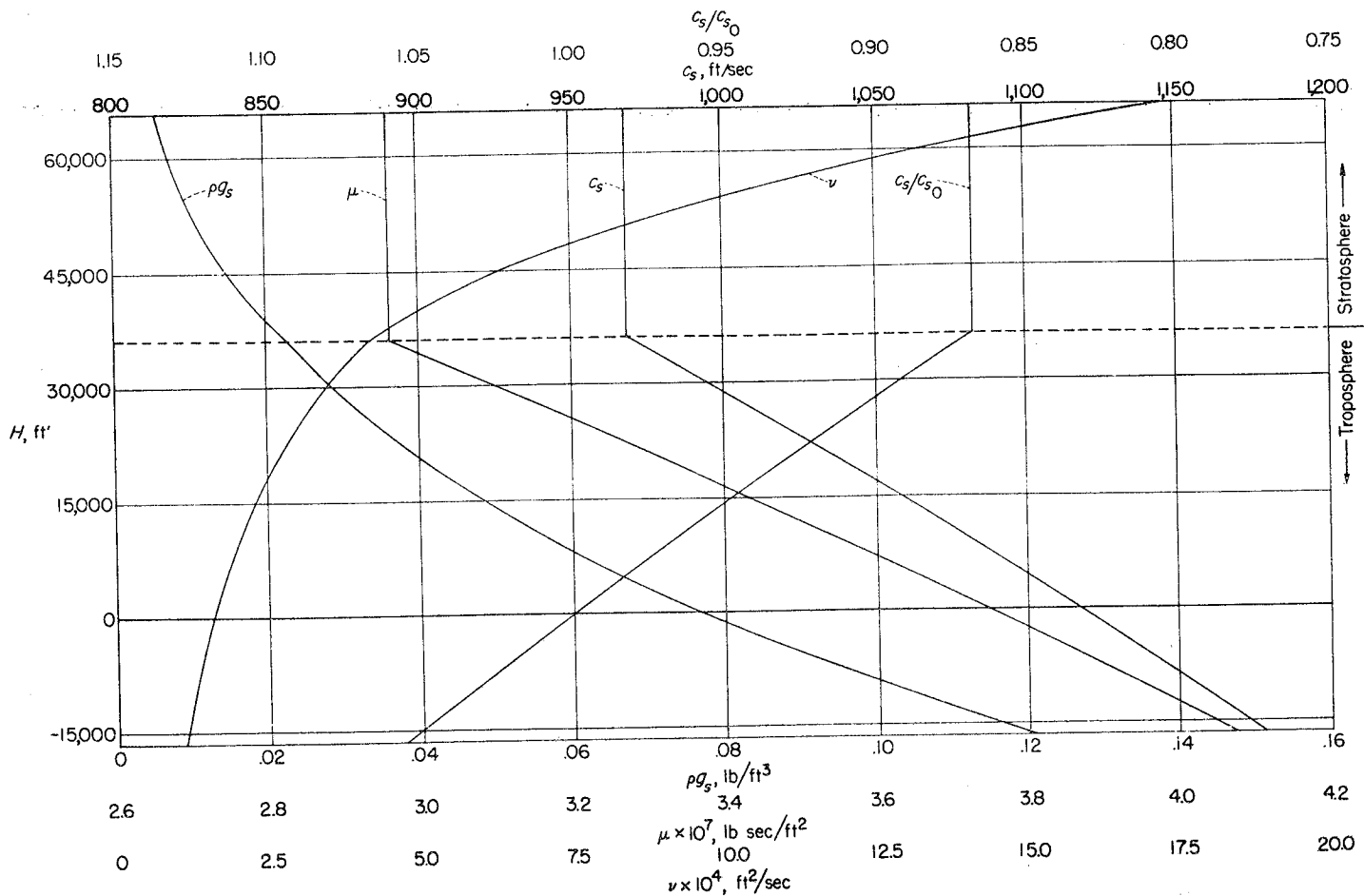
ENGLISH FIGURE II.—Specific weight \rho_g , viscosity \mu , kinematic viscosity \nu , sound speed c_s , and sound-speed ratio c_s/c_{s0} against geopotential H .
