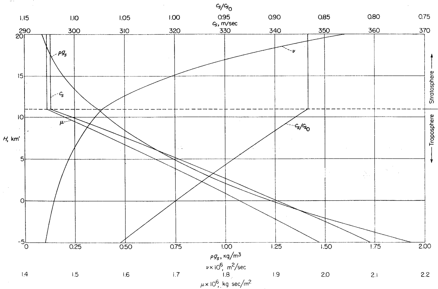
METRIC FIGURE II.—Specific weight \rho g_s , viscosity \mu , kinematic viscosity \nu , sound speed c_s , and sound-speed ratio c_s/c_{s0} against geopotential H .
