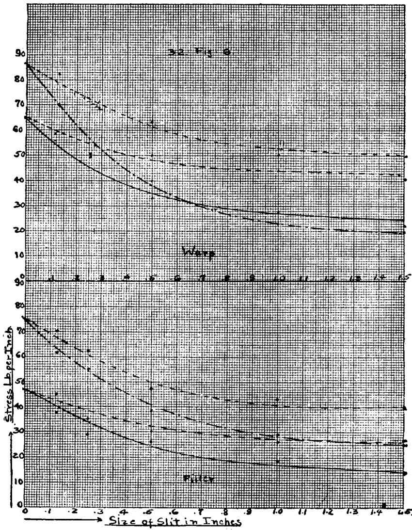
Tearing Tests on Linen #2 (Medium Grade) Curve I - Tearing Point - Undoped ——— Tearing Point - Undoped " II - " " Doped - - - - - " " Doped " III - Breaking Point - Undoped - - - - - Breaking Point " IV - " " Doped
