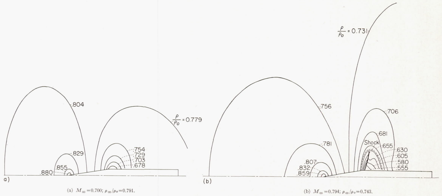
FIGURE 9.—Interferograms of flow past 10° semiangle wedge for various Mach numbers.
