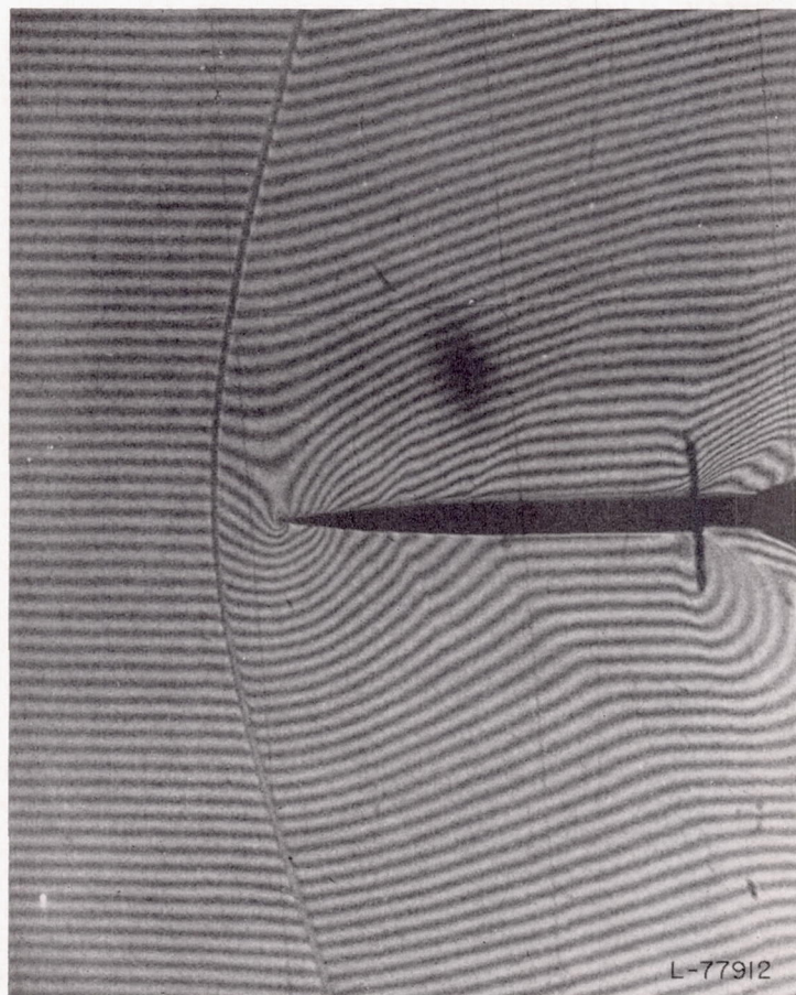
FIGURE 2.—Typical finite-fringe interferogram. 8.8-percent circular-arc section at M_\infty = 1.200 .
