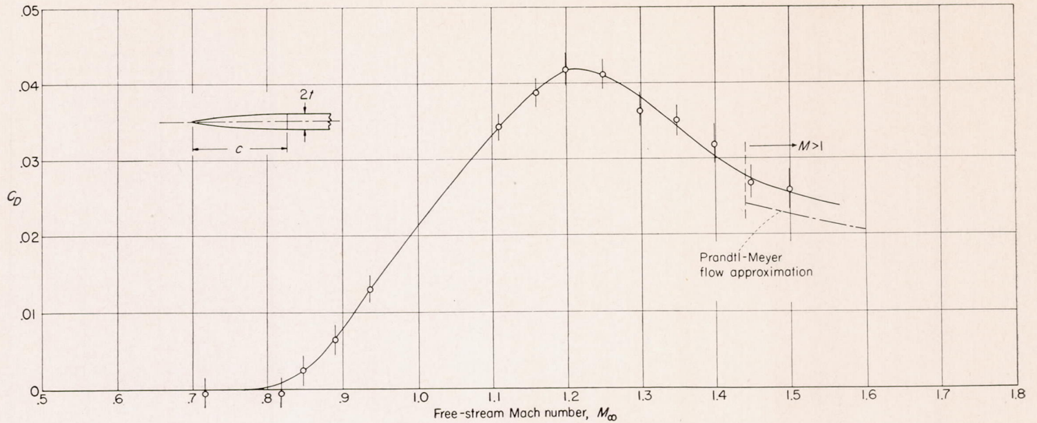
FIGURE 21.—Drag coefficient against Mach number for 8.8-percent circular-arc section.
