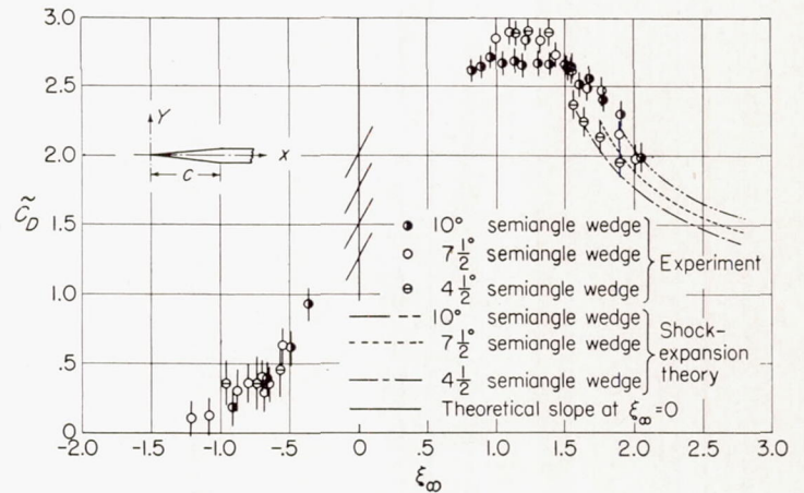
FIGURE 13.—Experimental reduced drag coefficient against reduced Mach number on a wedge.
