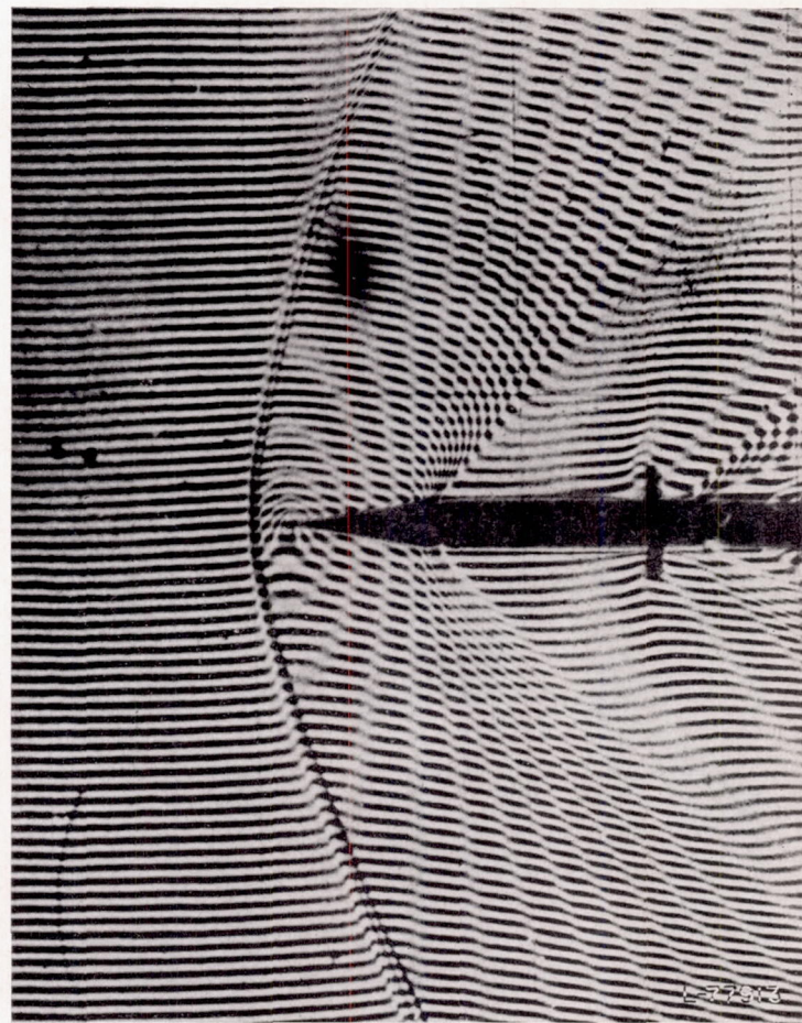
FIGURE 3.—Typical superimposed finite-fringe interferogram. 10^\circ semiangle wedge at M_\infty = 1.278 .
