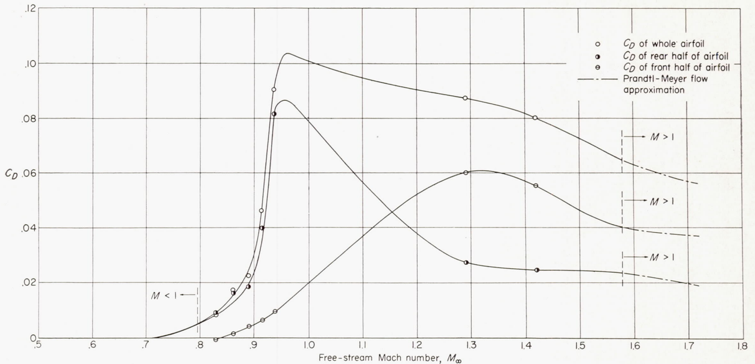
FIGURE 23.—Drag coefficient against Mach number for 12-percent biconvex circular-arc airfoil. (From data of fig. 22 on basis of constant Mach number distribution from M_\infty=0.96 to 1.20.)
