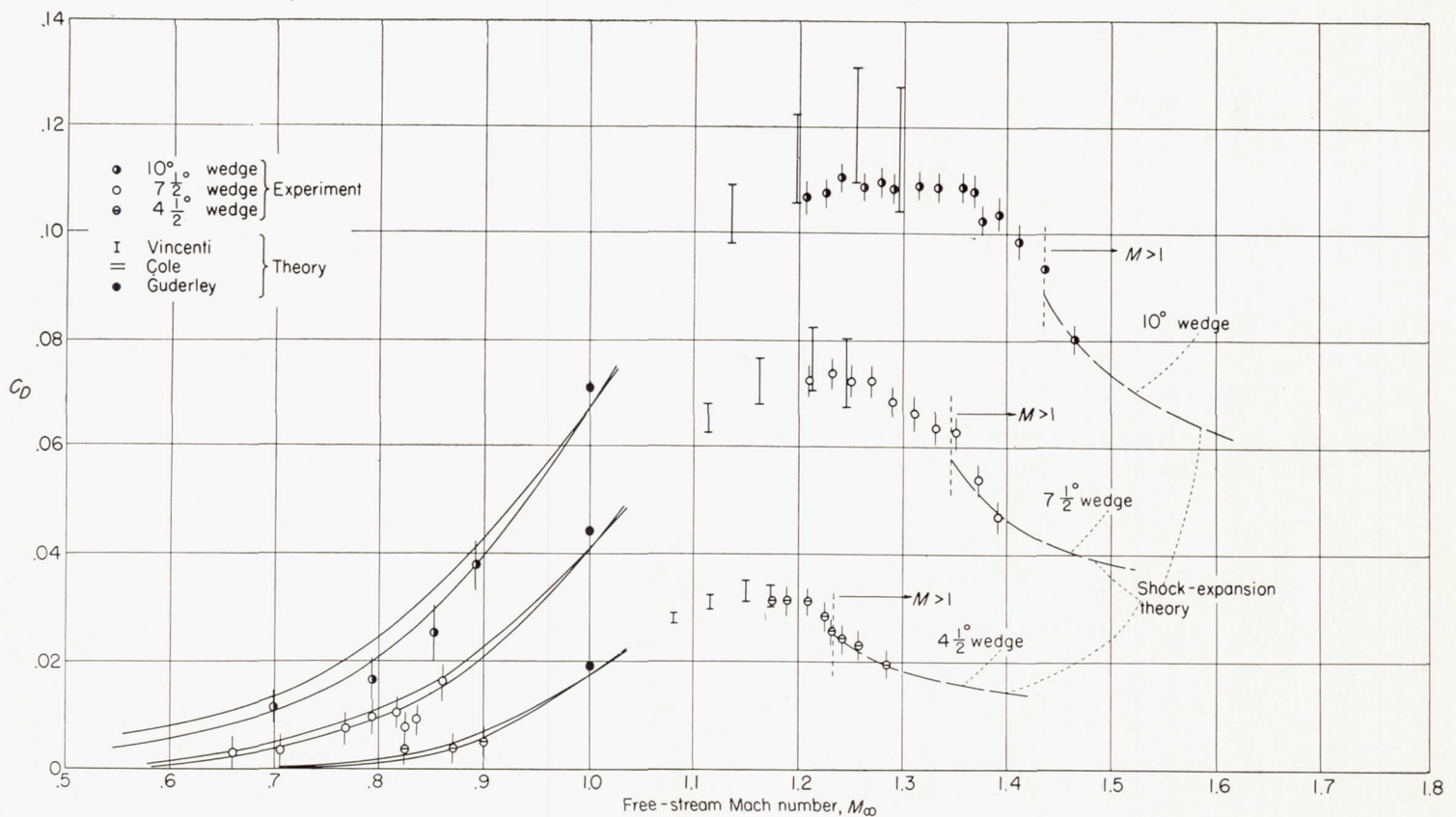
FIGURE 14.—Drag coefficient against Mach number for 4\frac{1}{2}^\circ , 7\frac{1}{2}^\circ , and 10^\circ semiangle wedges. Comparison of theory with experiment.
