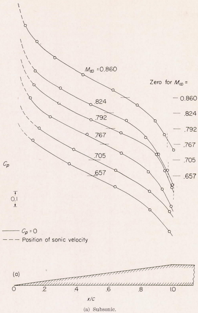
FIGURE 11.—Pressure distributions for 7\frac{1}{2}^\circ semiangle wedge.
