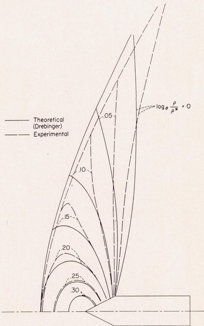
FIGURE 15.—Constant Mach number contours for 26.6^\circ semiangle wedge at M_\infty = 1.440 .
