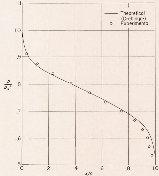
FIGURE 16.—Pressure distribution on a 26.6^\circ semiangle wedge at M_\infty = 1.440 .
