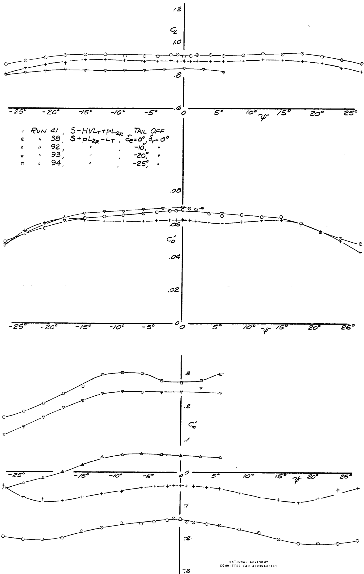
FIG. 25 - ELEVATOR EFFECTIVENESS OF THE MODEL IN YAW. FLOATS ON, FLAPS UP, \alpha_R=6^\circ , RUDDER NEUTRAL
