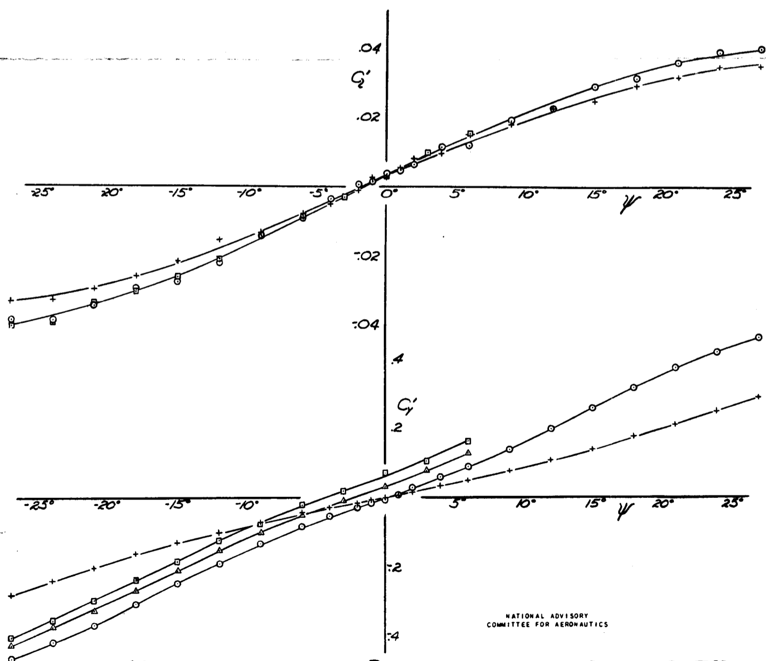
FIG 4-B- LATERAL STABILITY AND RUDDER EFFECTIVENESS CHARACTERISTICS OF THE MODEL WITH A LEADING EDGE FIN EXTENSION ( V_L ) \alpha_u = 6^\circ , FLOATS ON, FLAPS UP, ELEVATOR NEUTRAL, C_L \approx 0.9 .
