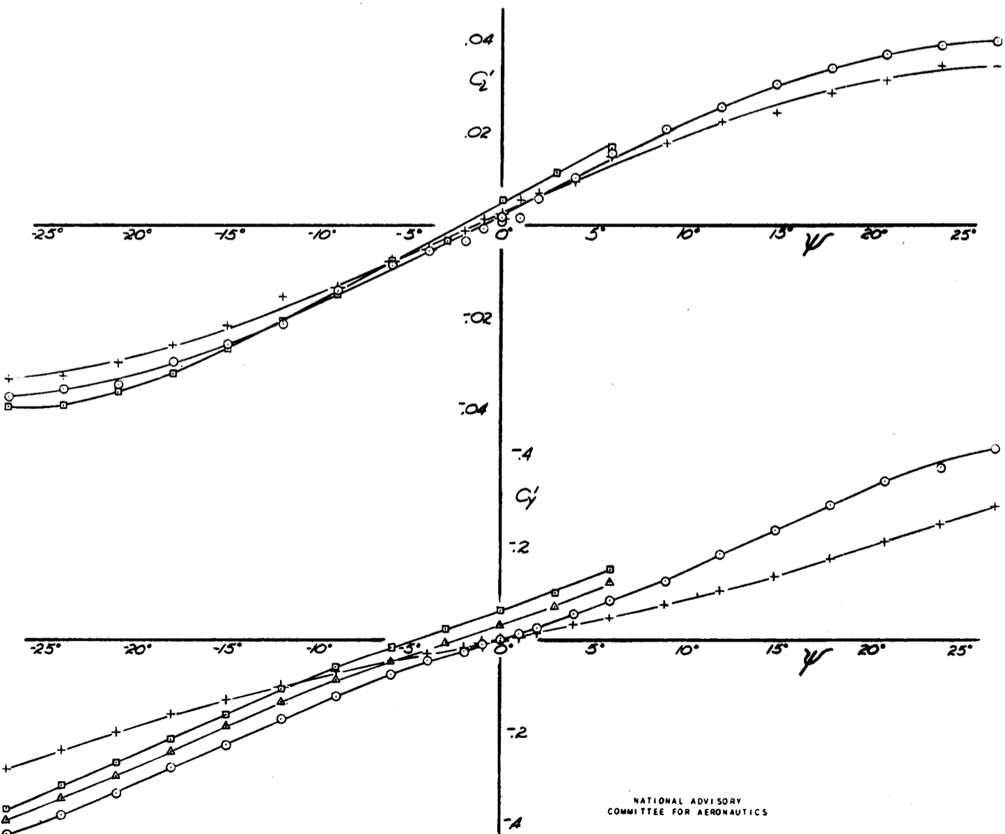
FIG 40 - RUDDER EFFECTIVENESS IN YAW, MODEL WITH FLOATS ON, FLAPS UP, \alpha_u=6^\circ , C_L \approx .9 , ELEVATOR NEUTRAL
