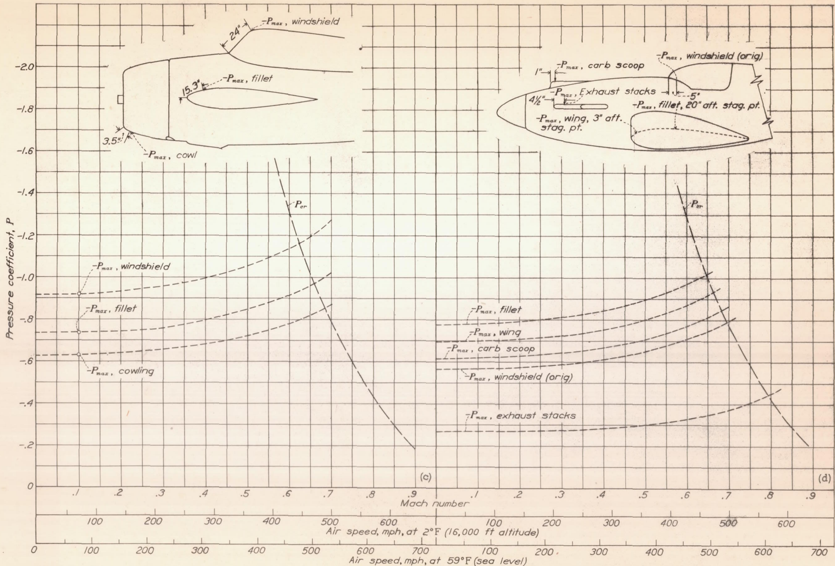
Figure 37d.- Critical speed for various components of airplane 11.
