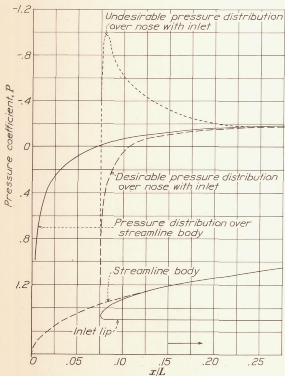
Figure 20.- Pressure distributions over air inlets.
