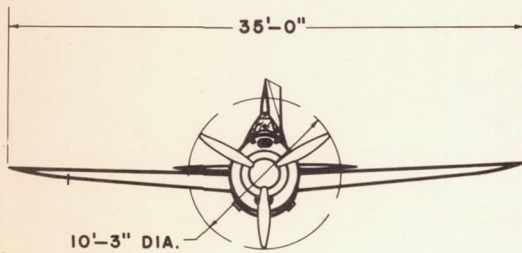
AIRPLANE 1
