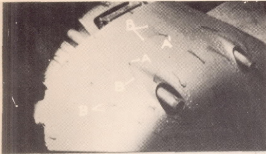
Original installation. Tubes faired & cowling gaps sealed. (a) Gun blast tube installation on airplane 3. (Note: A indicates fixed ends of tufts & B their free ends for original condition)
