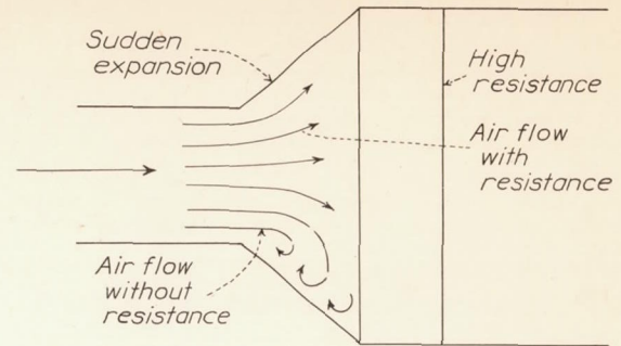
Figure 6.- Effect of high resistance in increasing allowable duct expansion.
