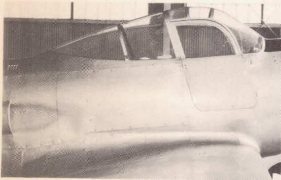
Original enclosure
