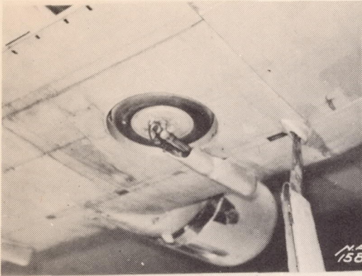
Original condition.
