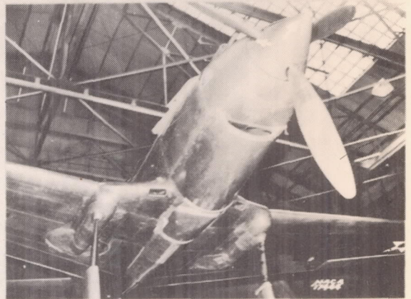
Original installation. Tubes faired & cowling gaps sealed. (a) Gun blast tube installation on airplane 3. (Note: A indicates fixed ends of tufts & B their free ends for original condition)
