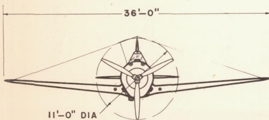
AIRPLANE 8
