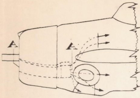
(a) Intercooler on airplane 10.
