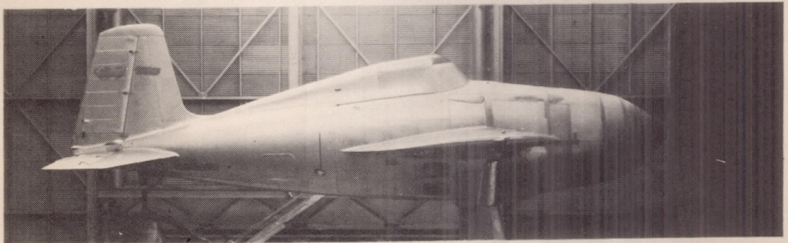
(j) Airplane 10 in smooth condition except for modified cockpit canopy.
