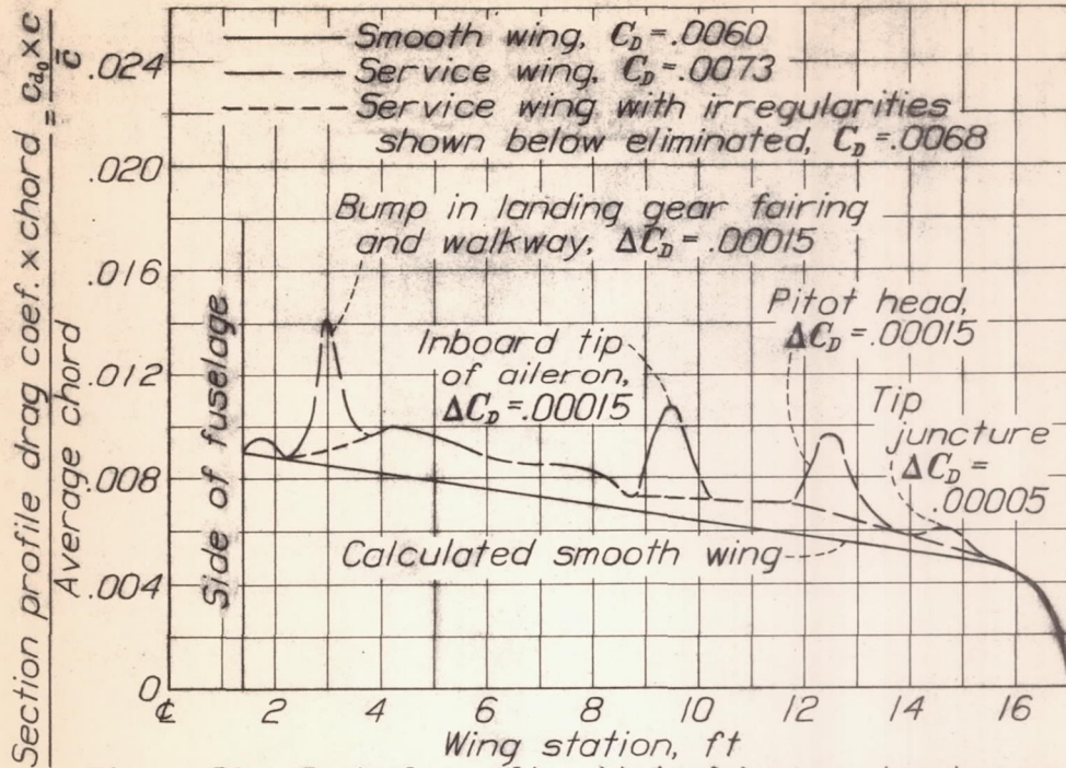
Figure 30.- Typical results obtained by momentum traverse along wing span and calculated smooth wing drag. Airplane 9.
