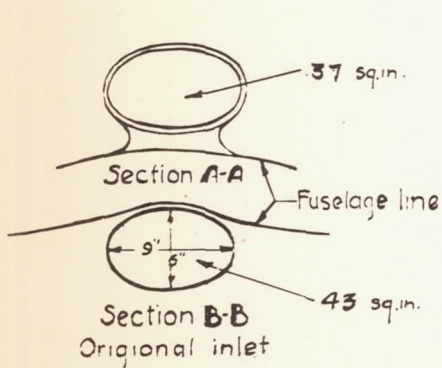
Figure 21.- continued. Carburetor air-intakes.
