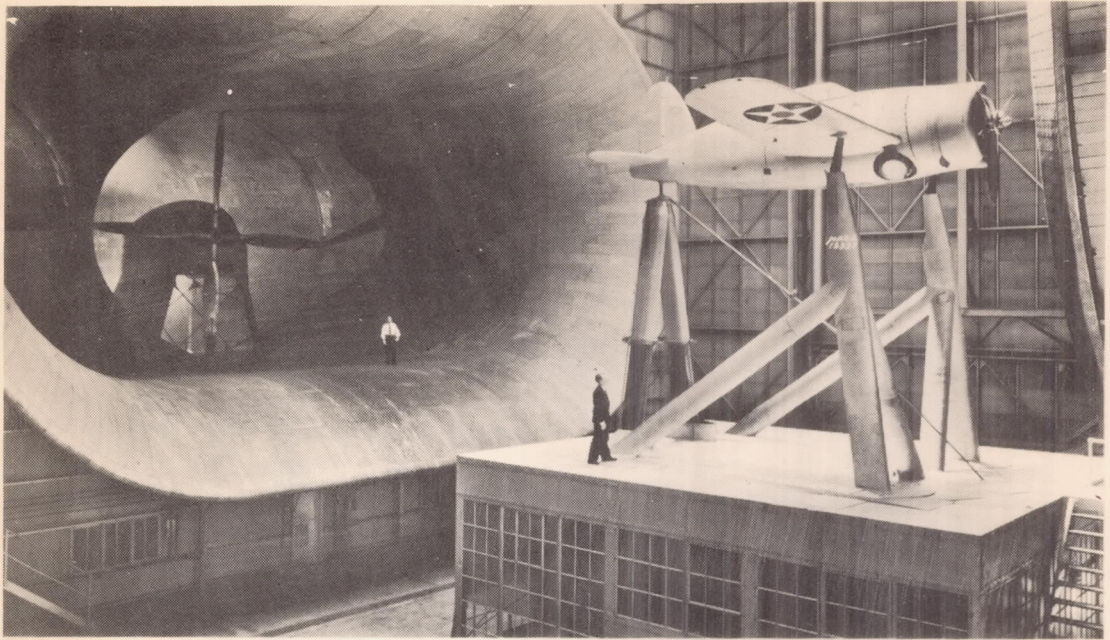
(a) Airplane 1.
