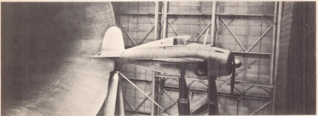
(b) Airplane 2.
