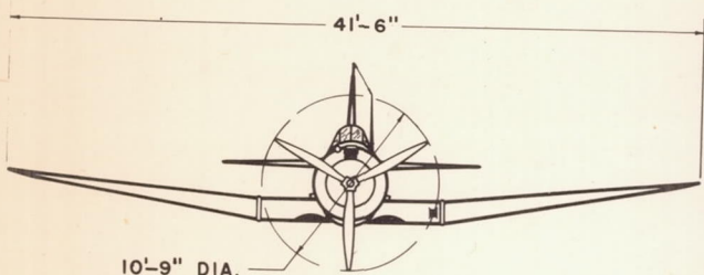
AIRPLANE 5
