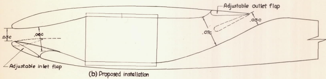
Figure 8.-Prestone radiator installation on airplane 9.
