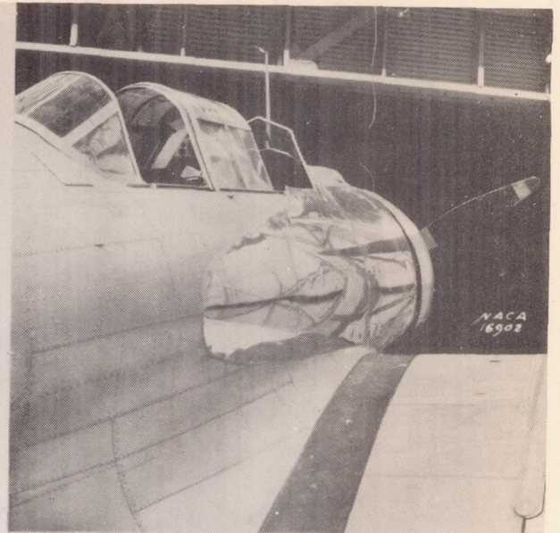
Repaired.
