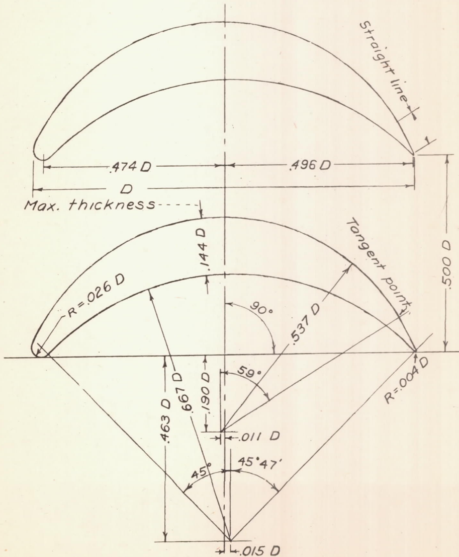
Figure 5.- Design of an efficient 90^\circ turning vane.
