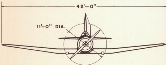
AIRPLANE 4
