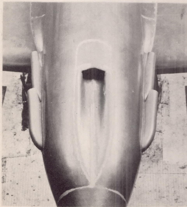
(c) Airplane 11 .
