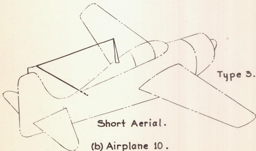
Figure 35.-Aerial installations.
