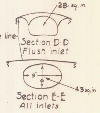
Figure 21.- continued. Carburetor air-intakes.
