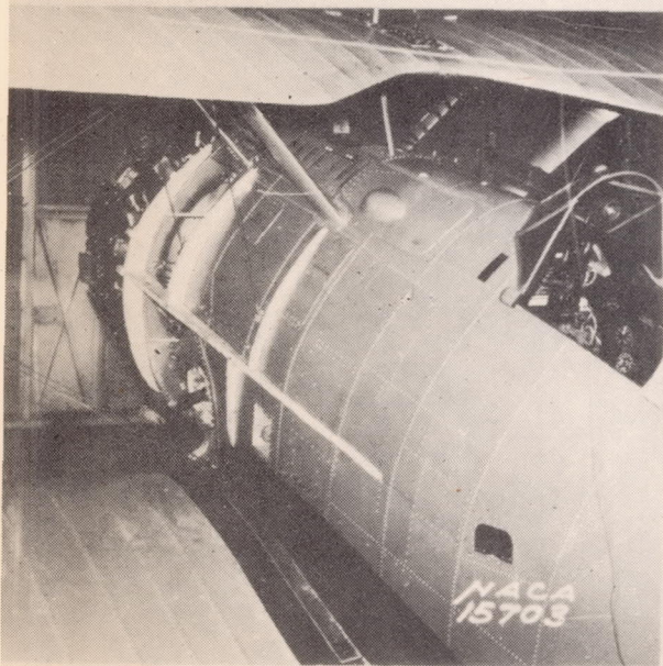
Original condition.
