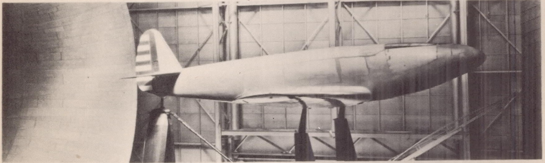
(i) Airplane 9 in smooth condition.
