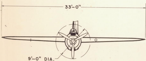
AIRPLANE 6
