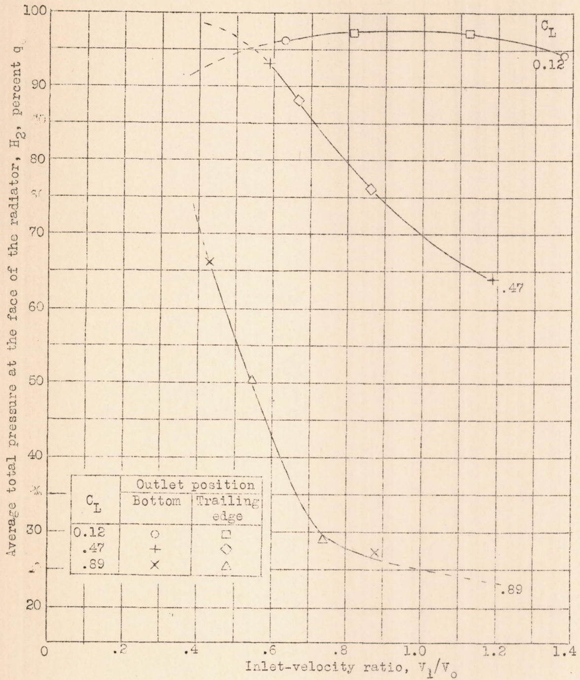
Figure 6.- Effect of inlet-velocity ratio on the average total pressure at the face of a radiator behind inlet 4. Propeller removed; airspeed, 63 miles per hour.
