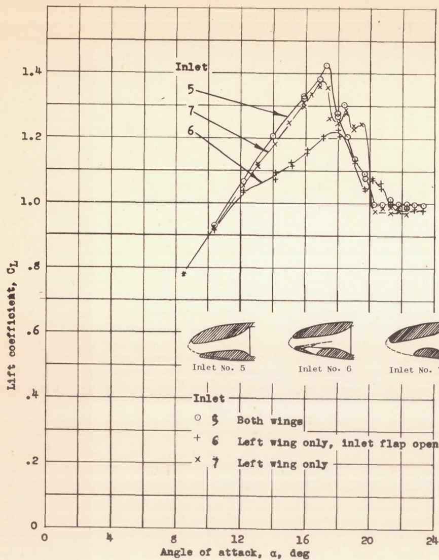
Figure 25. - Effect of lip position, leading-edge radius, and diffuser inclination on the maximum lift coefficient of the complete model. Propeller removed; landing flaps neutral; bottom outlet; outlet flaps closed; \Delta P/q_2 , 5.8.
