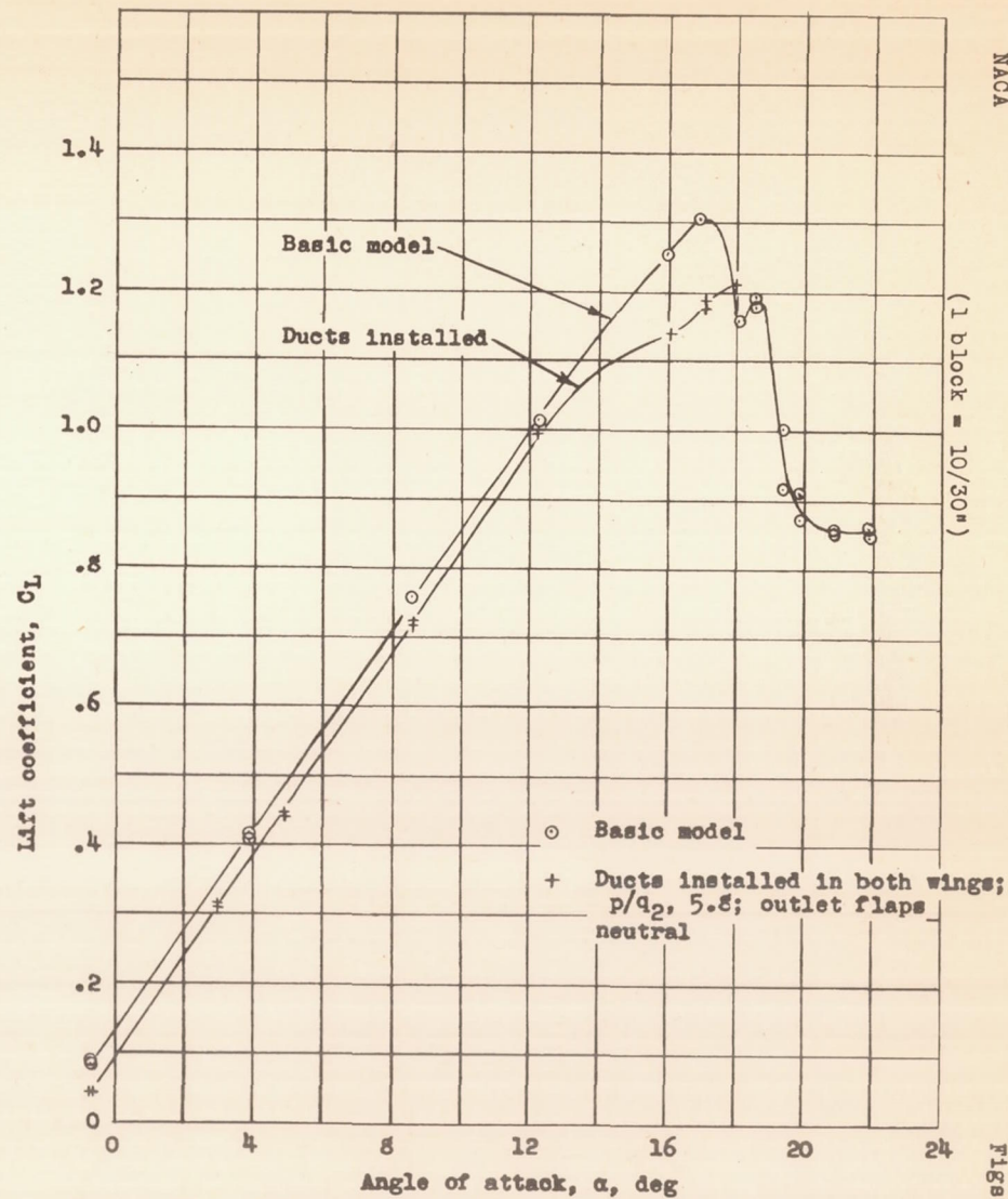
Figure 26. - Effect of inlet 4 and trailing-edge outlet on maximum lift coefficient of the model with tail surfaces removed. Landing flaps neutral; propeller removed.
