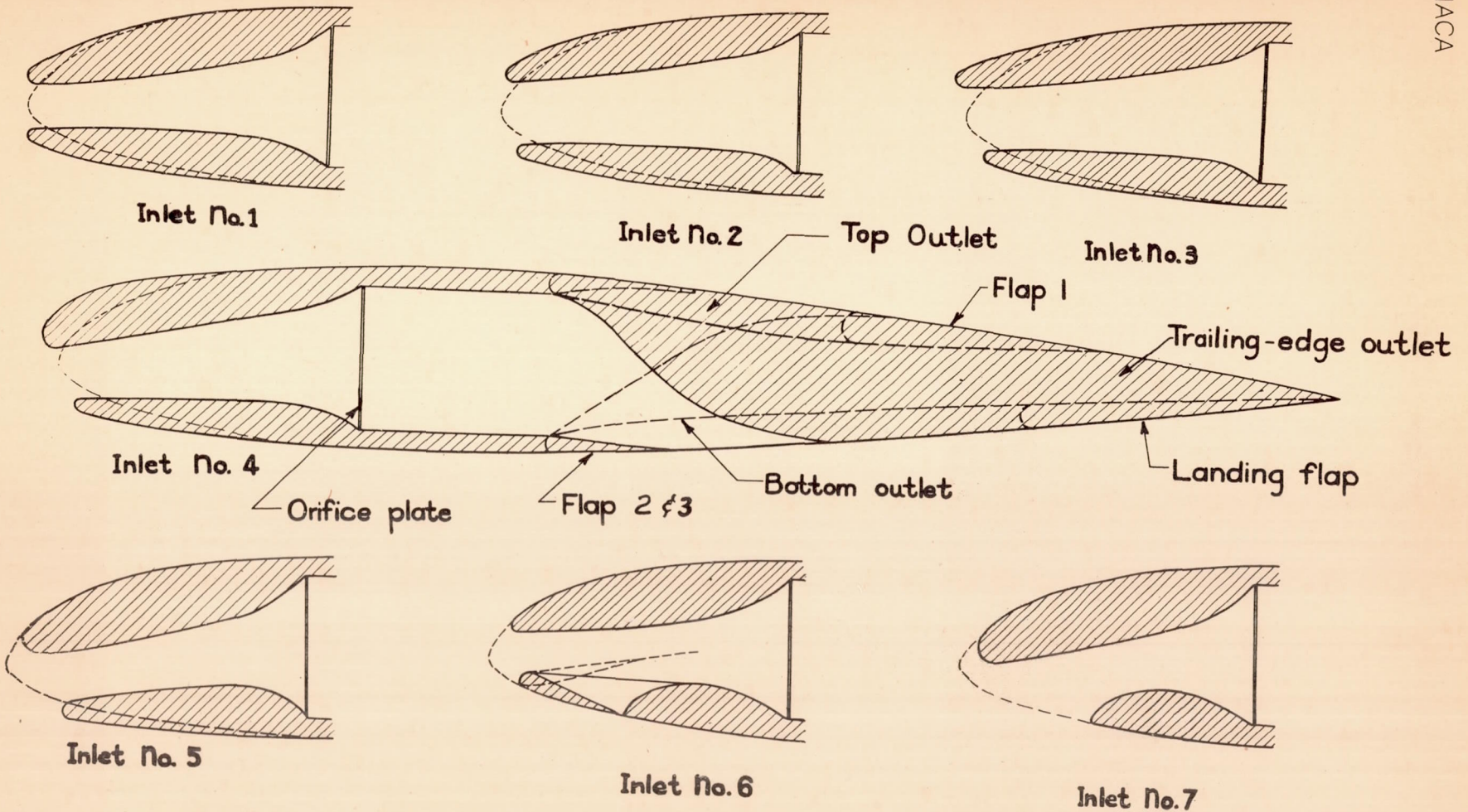
Figure 3.-Inlet and diffuser profiles.
