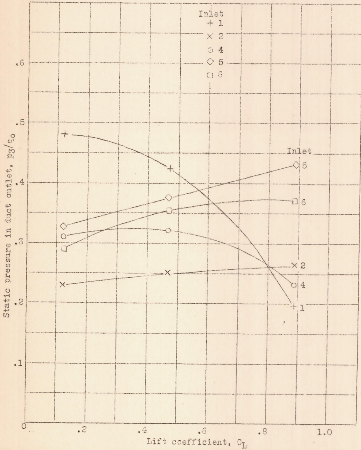
Figure 22.- Effect of inlet design of the static pressure at an outlet in the lower surface of a wing as a function of lift coefficient. Propeller removed.
