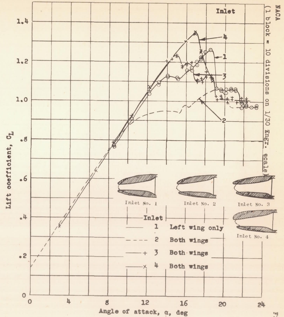
Figure 24. - Effect of inlet size and upper-lip position on the maximum lift coefficient of the complete model. Propeller removed; landing flaps neutral; bottom outlet; outlet flaps closed; \Delta p/q_2 , 5.8.
