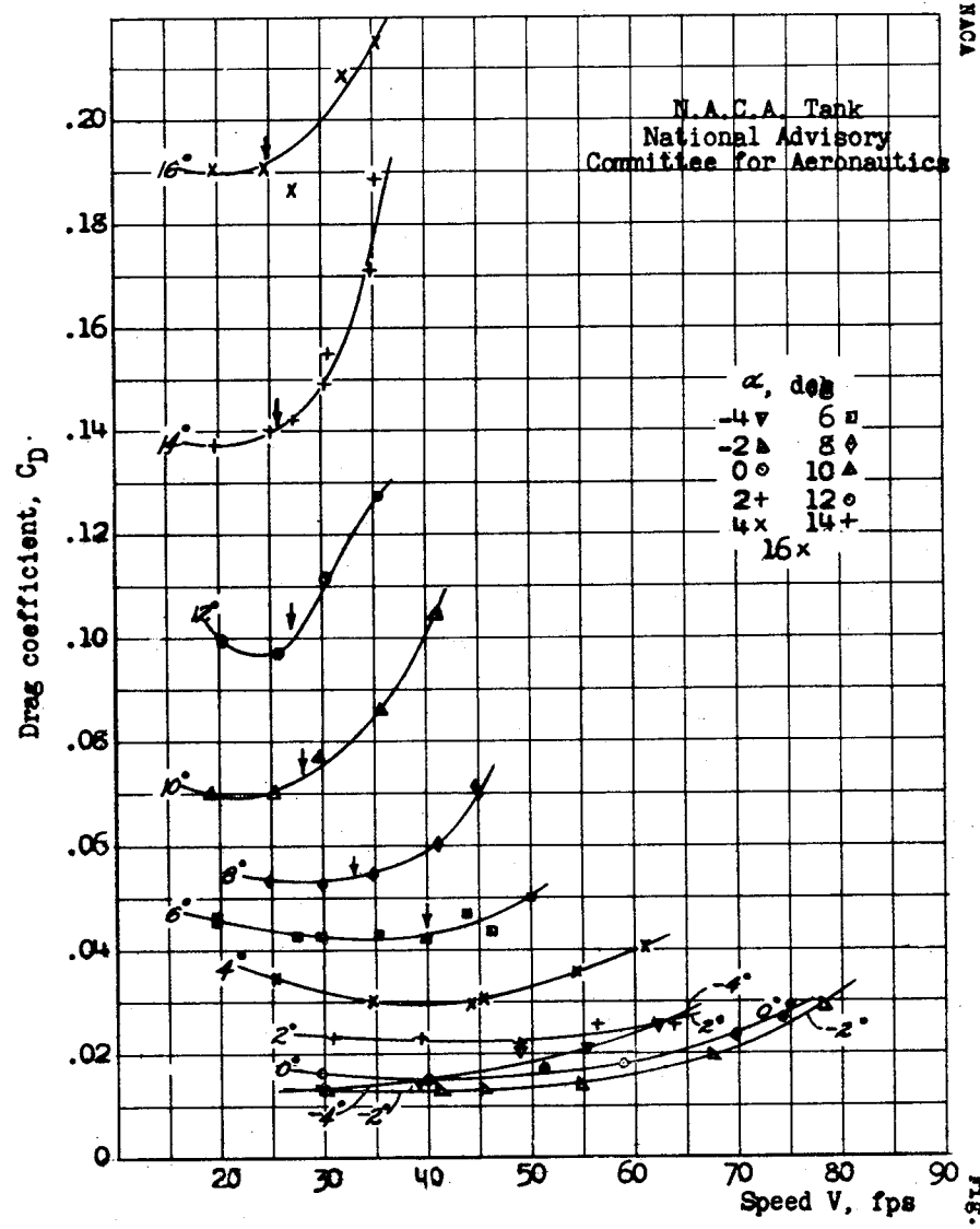
Fig.15 .- NACA 16-509 section hydrofoil. 30° dihedral. Depth, 16.3 inches to \epsilon/4 at tips.
