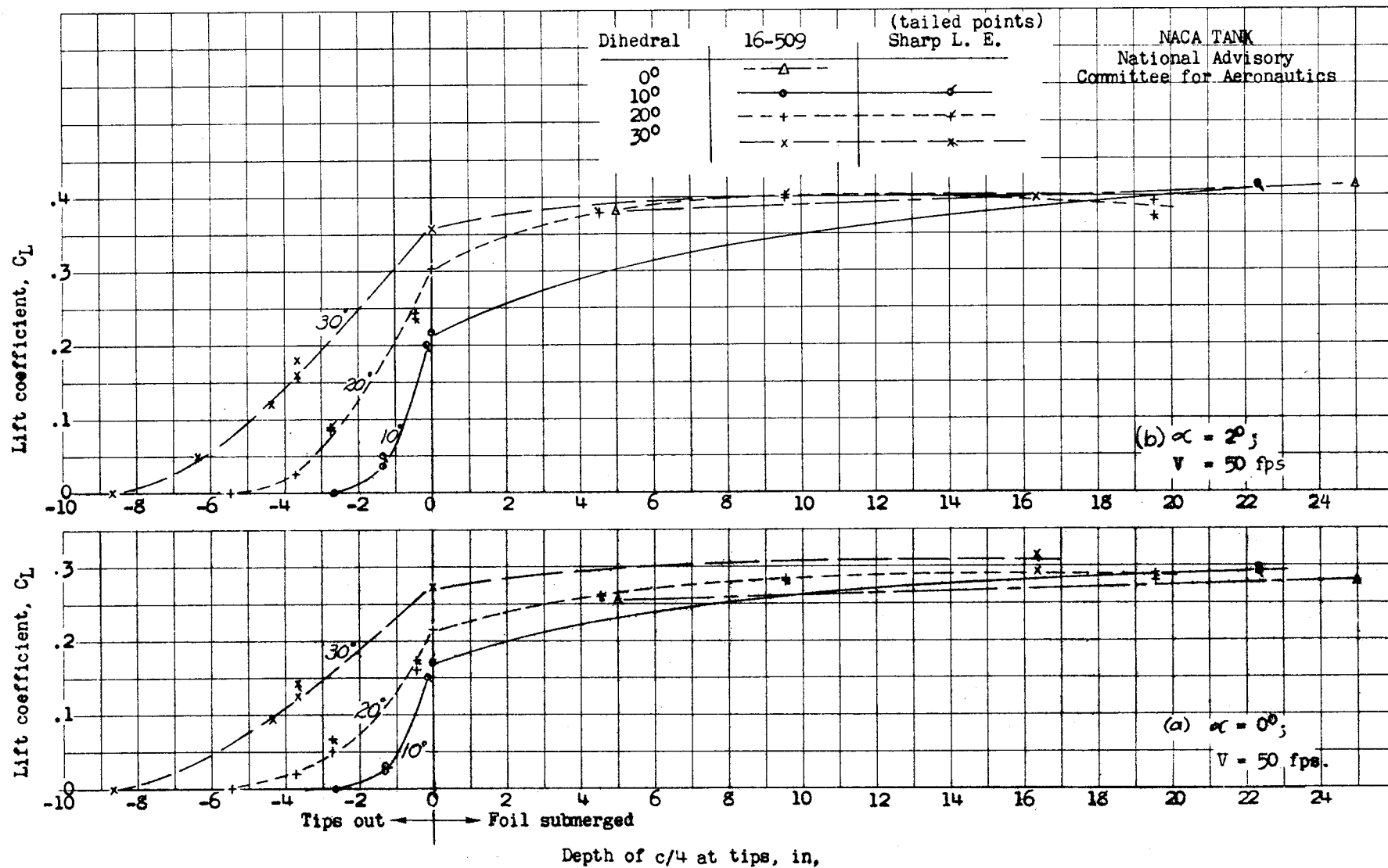
Fig. 16a,b.—Effect of depth on lift coefficient.
