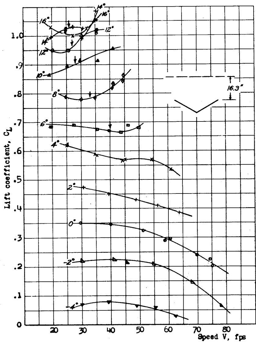
Fig.15 .- NACA 16-509 section hydrofoil. 30° dihedral. Depth, 16.3 inches to \epsilon/4 at tips.
