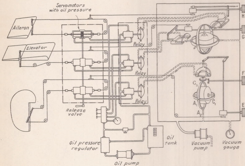
Figure 3.- Assembly sketch of Sperry stabilizer. H, climbing knob; G, banking knob. (For other references see text).
