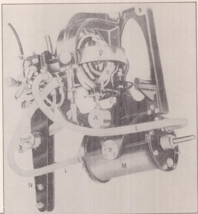
Figure 7.- Smith aileron control.
