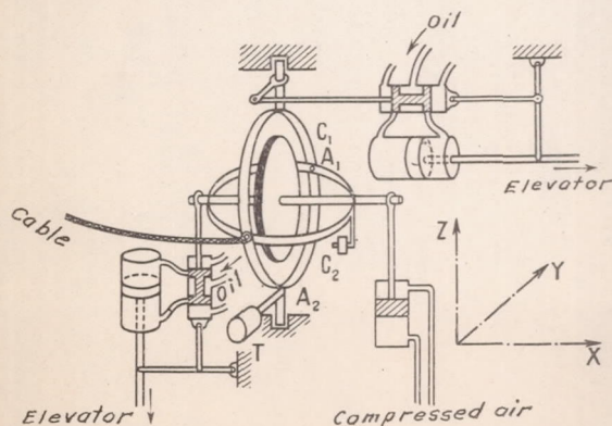
Figure 4.- Smith rudder and elevator control.
