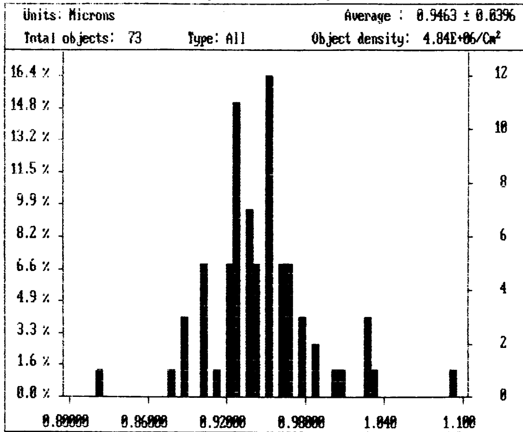
Figure 7. Percent of various size beads produced, illustrating monodispersity beads size 0.95 μ (on average)
