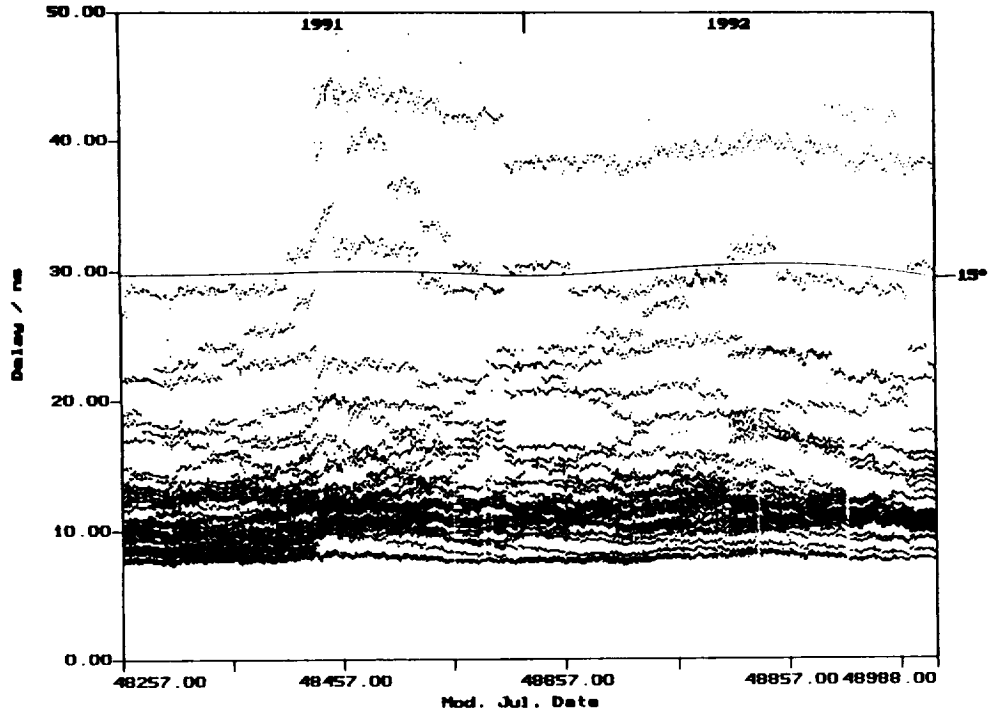
Fig. 12 Hopfield model: Tropospheric delay for each satellite track .
