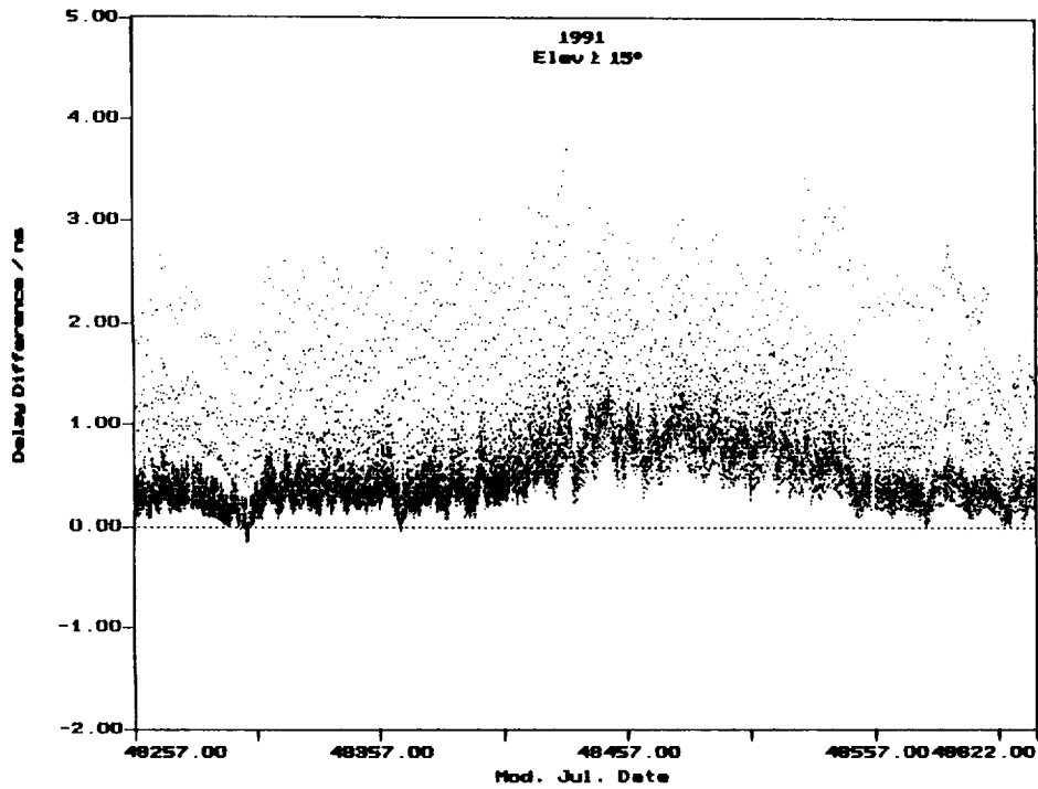
Fig. 18 Delay difference between the Hopfield model and the STI model (each satellite track).
