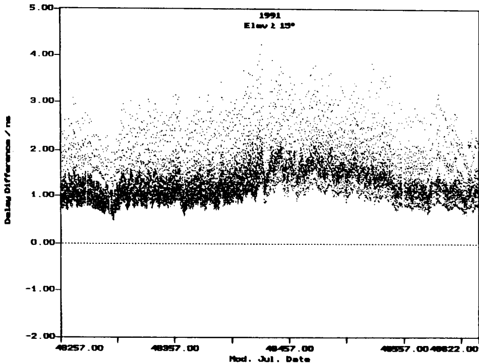
Fig. 17 Delay difference between the Hopfield model and the NBS model (each satellite track).
