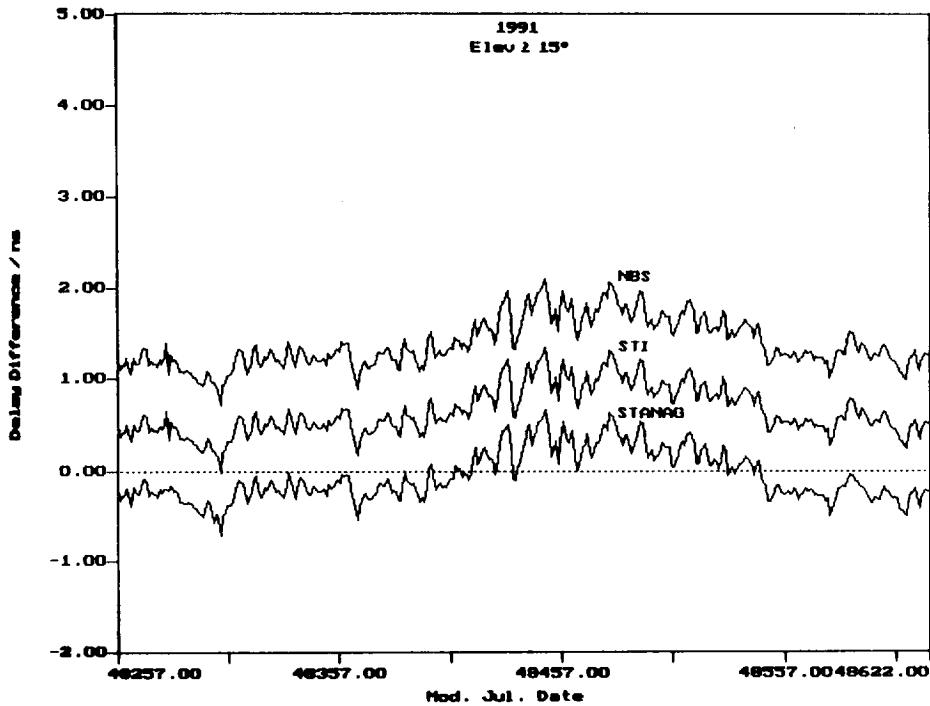
Fig. 21 Delay differences between the Hopfield model and the NBS, STI and STANAG models (one day mean).
