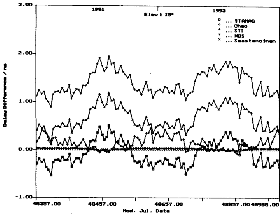
Fig. 14 Delay differences between the Hopfield model and the other models (seven day mean).
