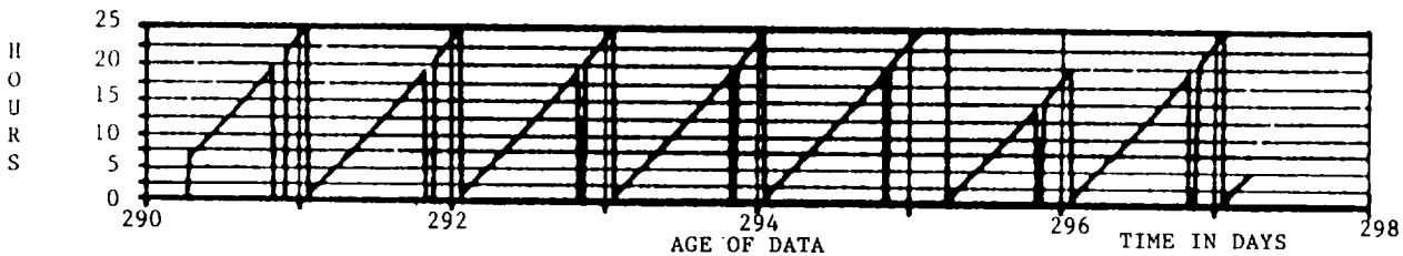
FIGURE 7: RMS-ERD FOR NAVSTAR 25
