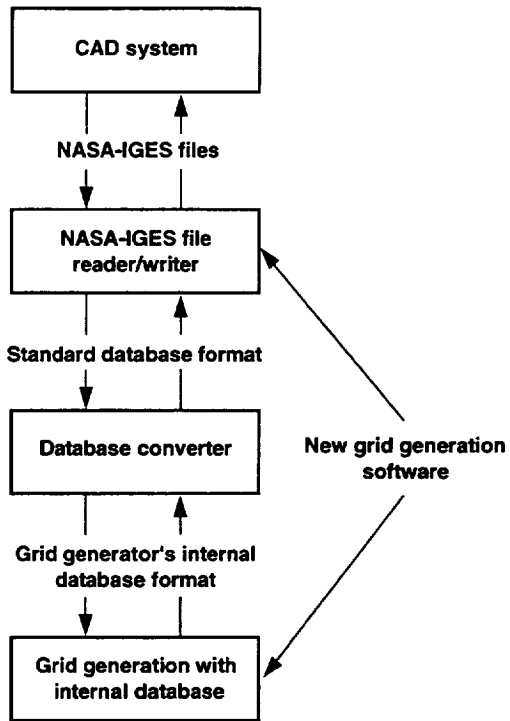
Figure 2. Grid generation with NASA-IGES file reader-writer.
