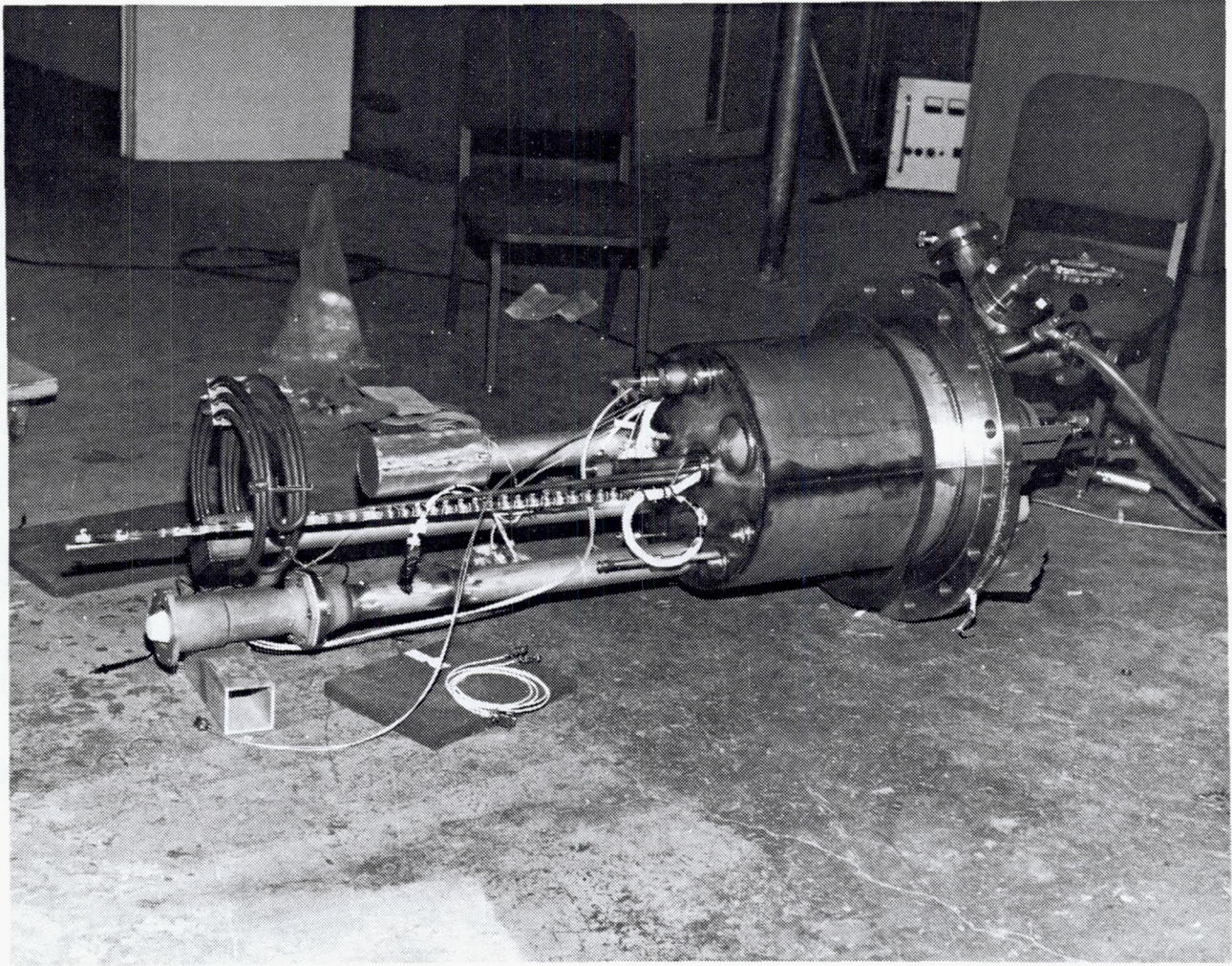
Figure 3-11. Test Tank Manhole Cover Equipment
