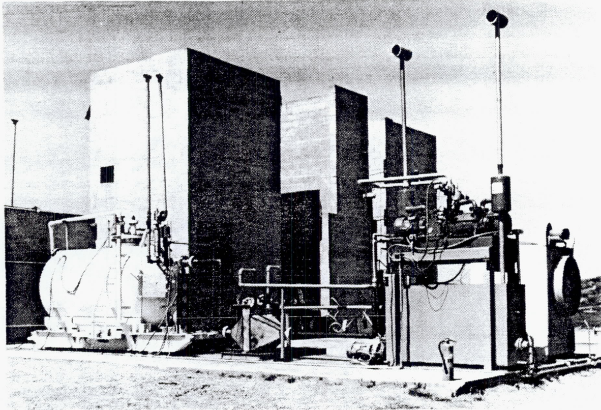
Figure 4-1. MDA 1.9 m 3 (500-Gallon) Slush Hydrogen Test Tank
