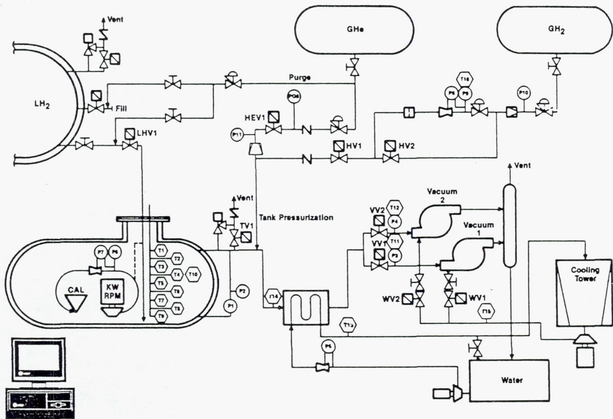
Figure 4-2. MDA Slush Hydrogen Test Facility Schematic
