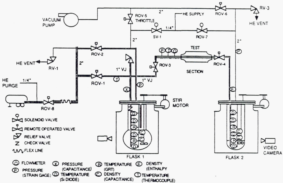
Figure 4-18. Sub-Scale Test Facility Schematic
