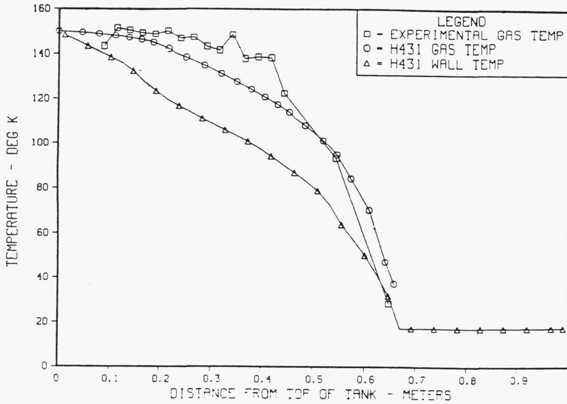
Figure 4-13. H431 Temperature Prediction Comparison for Test 2.0-6
