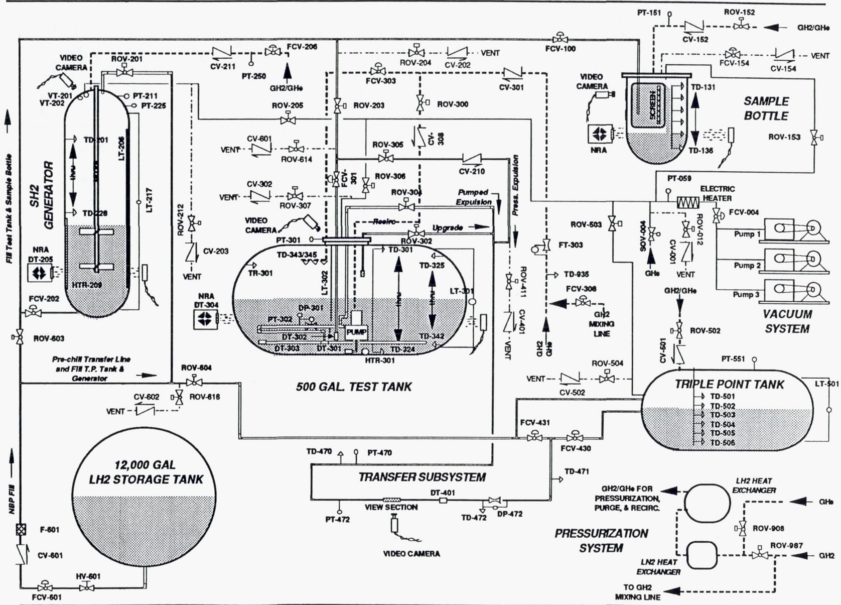
Figure 3-1. Slush Technology Facility (STF) Schematic
