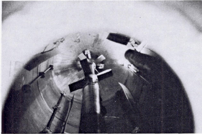
Figure 3-6. Mixer Installed in the Slush Generator
