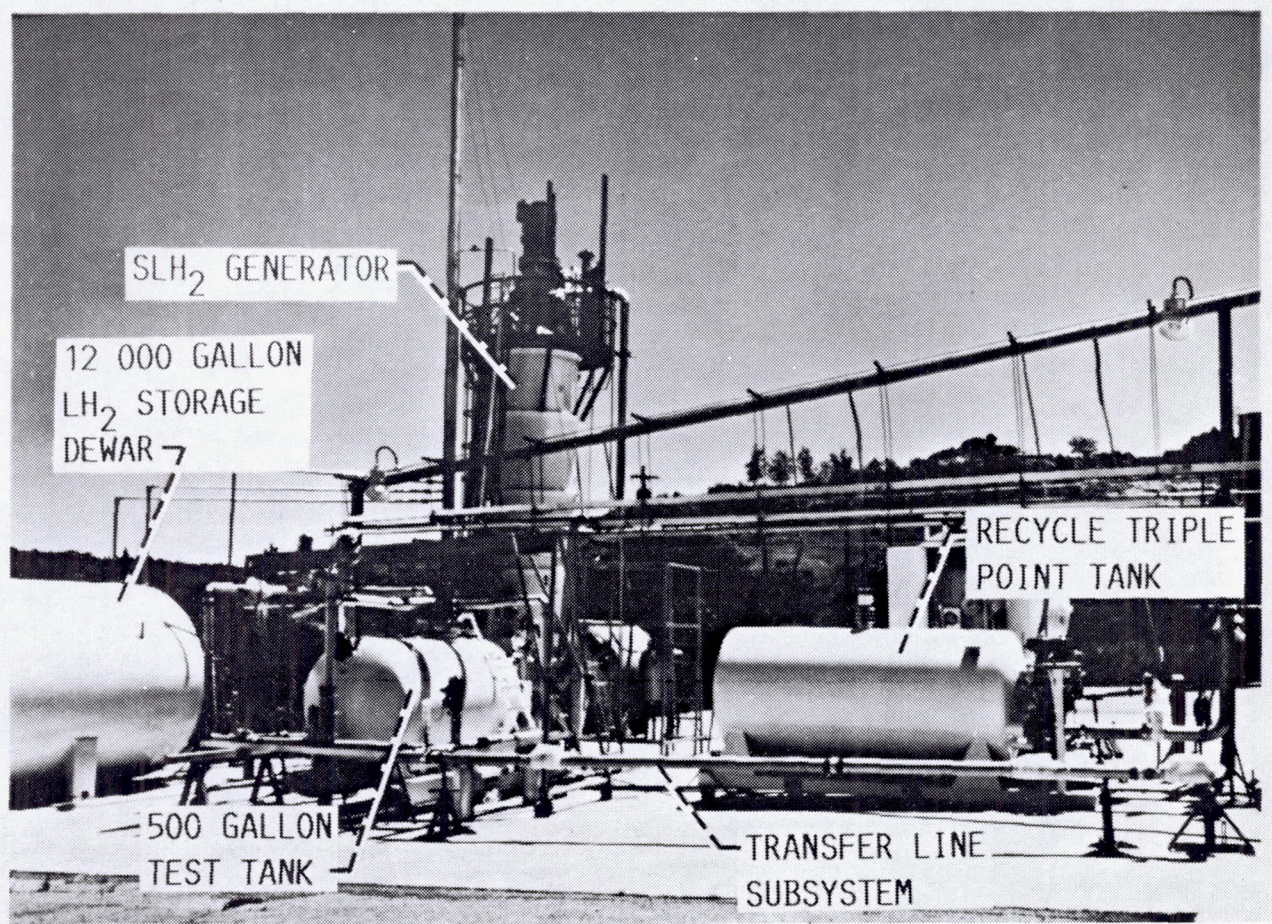
Figure 5-1. Overall View of the STF
