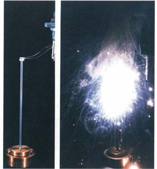
A flammability test at WSTF: the titanium rod in the left image is ignited and burned in an oxygen-enriched environment and scientists study combustion characteristics. WSTF conducts tests like this to help system designers select the most burn resistant metal alloys for use in oxygen systems.
