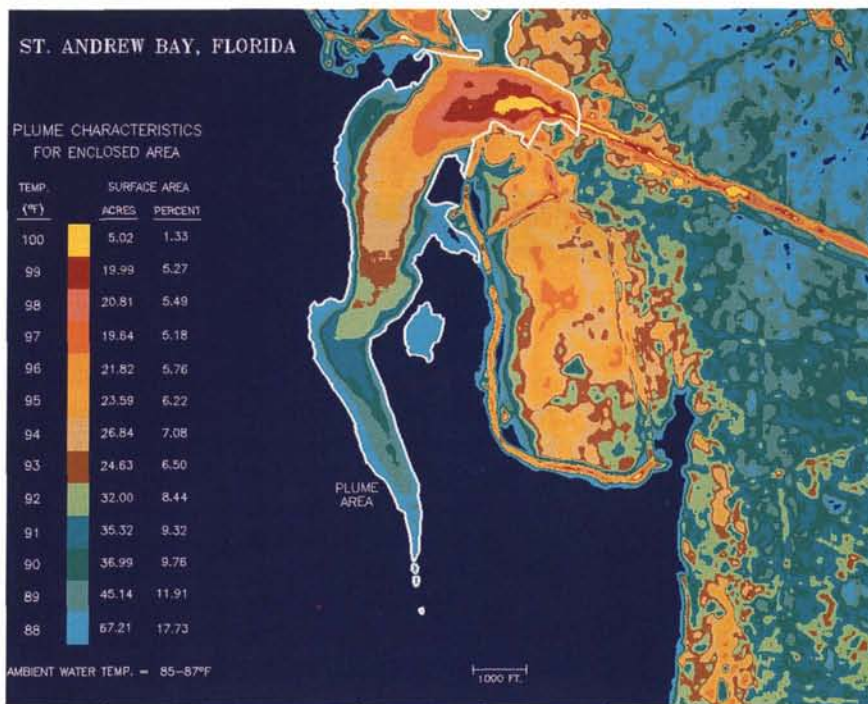
This image shows the actual temperatures of heated water being discharged into a Florida bay from a generating plant. It was part of a broader study of the power plant's impact on plant and animal life in the bay, conducted in a NASA program to help private firms capitalize on the potential of commercial remote sensing.
