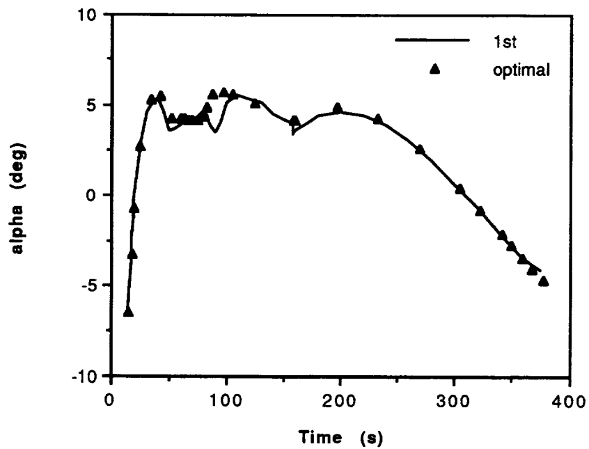
Figure 5.15. Closed Loop Angle of Attack Profile Under Wind and \alpha q Constraint.
