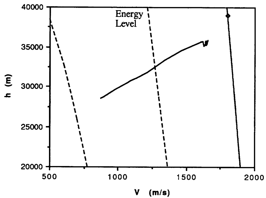
Figure 3.3. Reduced Solution Using Estimated Flight-path Angle.
