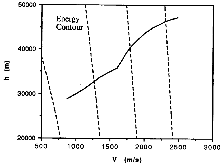
Figure 3.1. Reduced Solution with \gamma = 0 .
