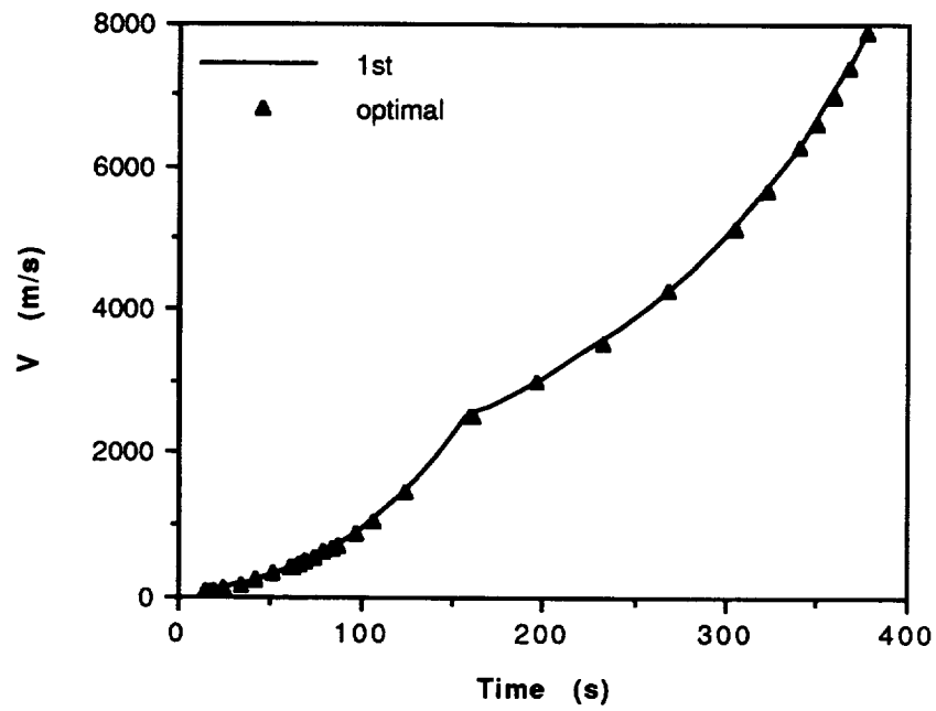
Figure 5.12. Closed Loop Velocity Profile Under Wind and \alpha_q Constraint.
