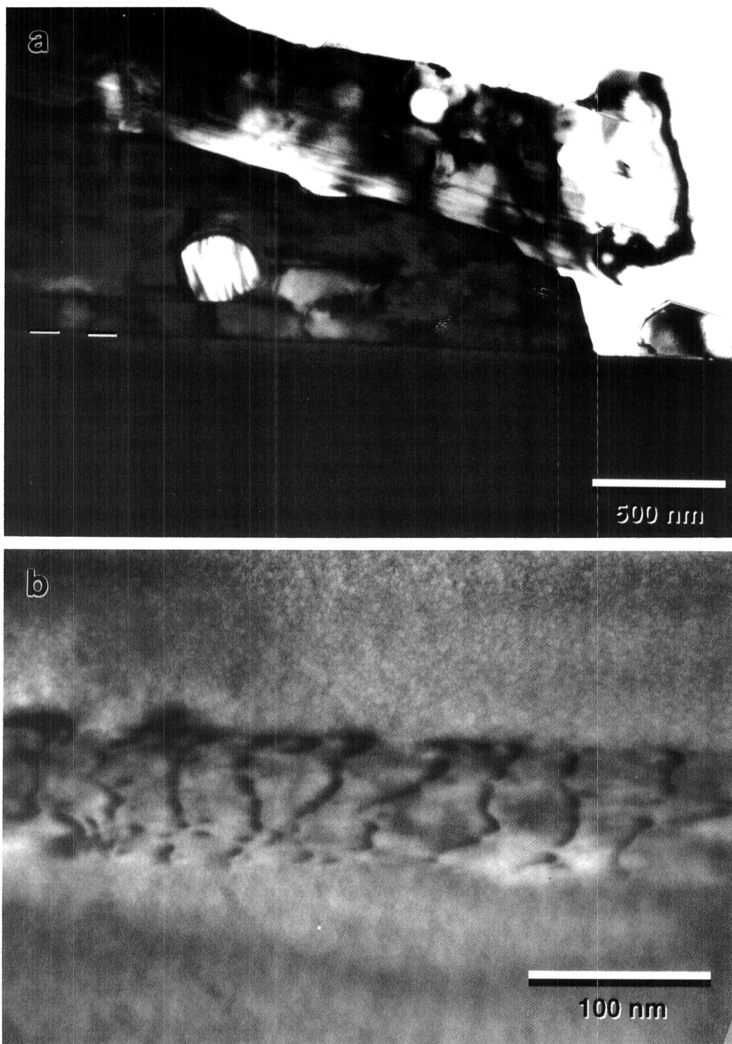
Fig. 5. TEM photomicrograph of (a) typical area of epitaxially grown (Tl,Bi)-1223 film and (b) dislocations in film at \text{LaAlO}_3 interface.
