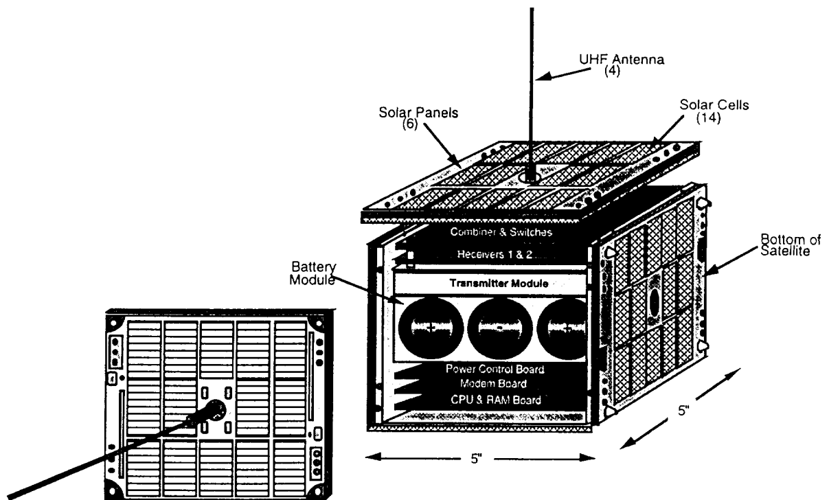
Figure 2. Nanosat Configuration
