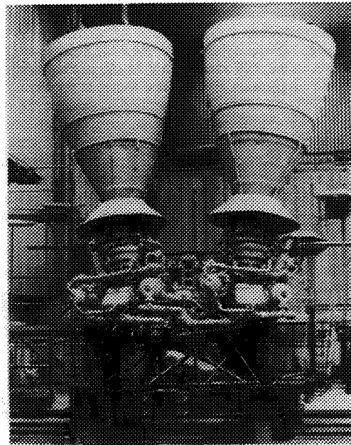
Fig. 7 RD-701 dual-fuel engine mock-up.
