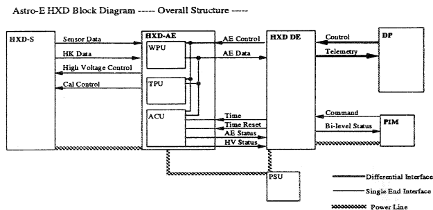
Figure 11: Block diagram of the HXD electronics
