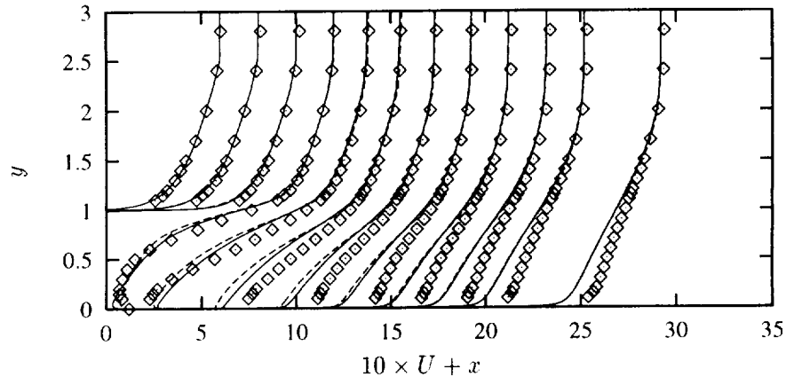
FIGURE 1. DS Velocity profiles. \diamond experiments, — model version (1), --- model version (2).
