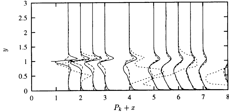
FIGURE 14. DS T d profiles. Symbols as in Fig. 12.
