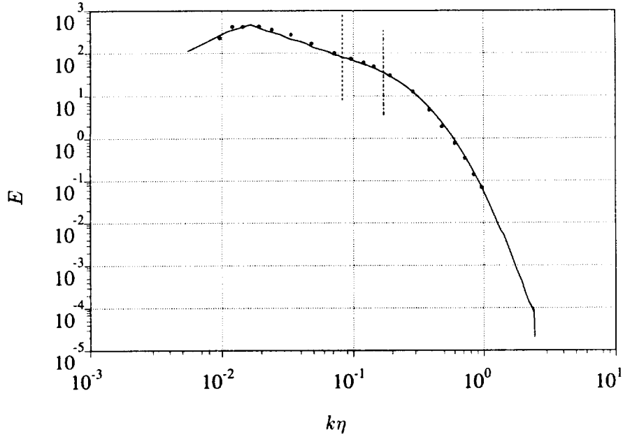
FIGURE 2. Spectrum of the 512^3 DNS ( Re_\lambda = 63.5 ). Also shown are the cuts used to produce the 64^3 and 32^3 synthetic LES fields. ● : Comte-Bellot and Corrsin experimental data at Re_\lambda = 65.1 . k normalized by Kolmogorov scale \eta .
