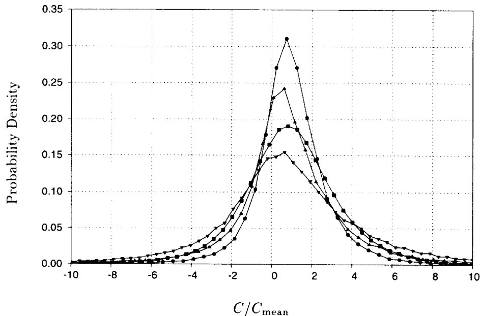
FIGURE 6. Normalized pdf for Model 1 with scaling (a) in the velocity-pressure formulation; 128^3 \rightarrow 32^3 ( \nabla ), 128^3 \rightarrow 16^3 ( \ast ), 512^3 \rightarrow 64^3 ( \blacksquare ), 512^3 \rightarrow 32^3 ( \bullet ) with sharp cutoff.
