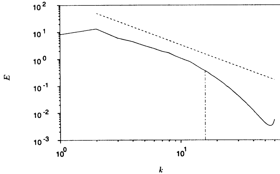
FIGURE 1. Spectrum of the 128^3 DNS ( Re_\lambda = 95.8 ). Also shown is the cut used to produce the 32^3 synthetic LES field. —, E(k) ; ----, K^{-5/3} .
