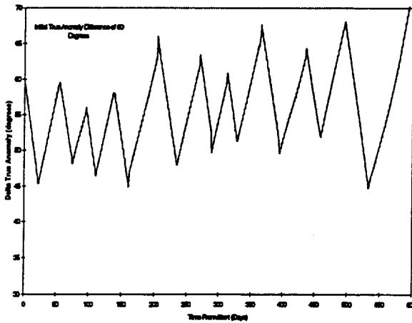
Figure 1 - Constellation Drift of S/C with Different Groundtracks
