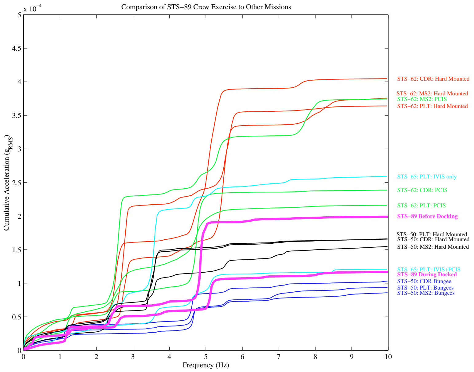
Figure 5. Cumulative RMS Acceleration versus Frequency for Exercise Comparison
