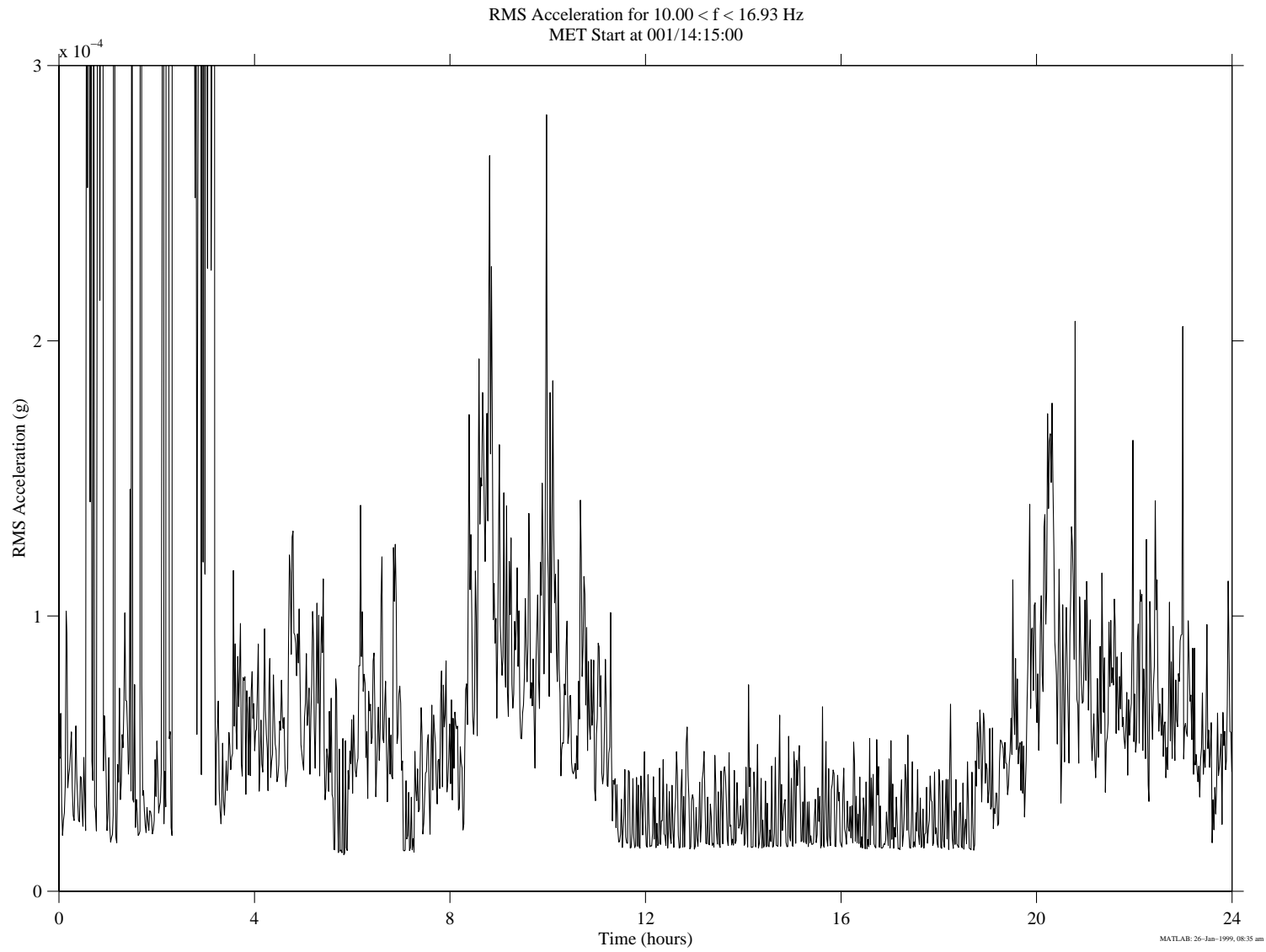
Figure 2. RMS Acceleration Versus Time ( 10 < f < 16.93 Hz), Orbiter SAMS TSH A
