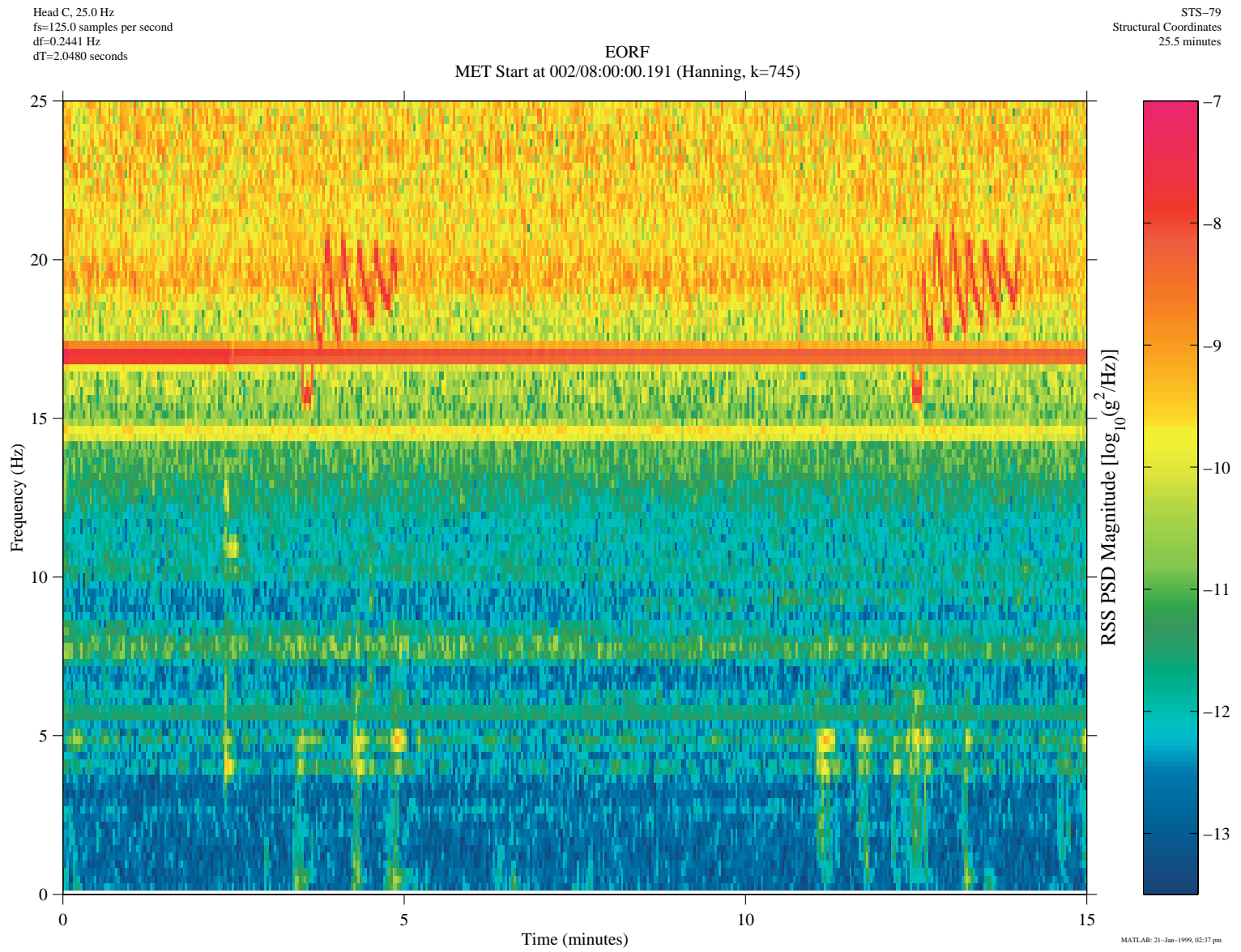
Figure 8. Spectrogram Featuring EORF Signature, STS-79 SAMS TSH C
