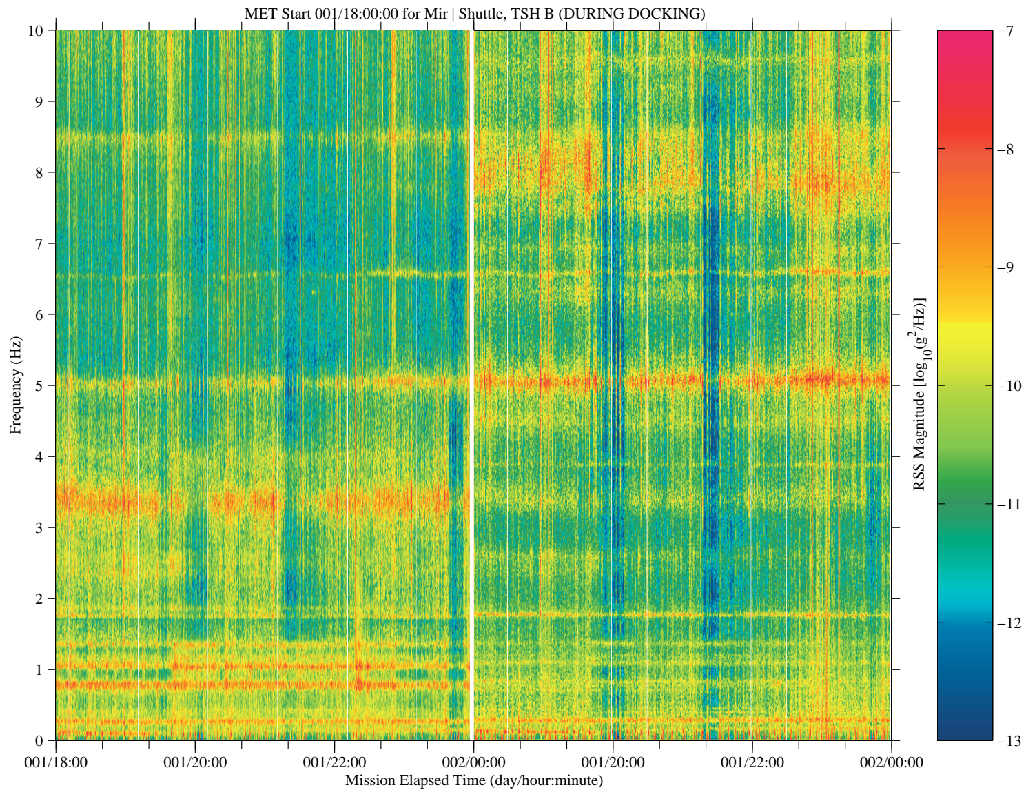
Figure 27. Spectrogram Overlay During Docked Operations
