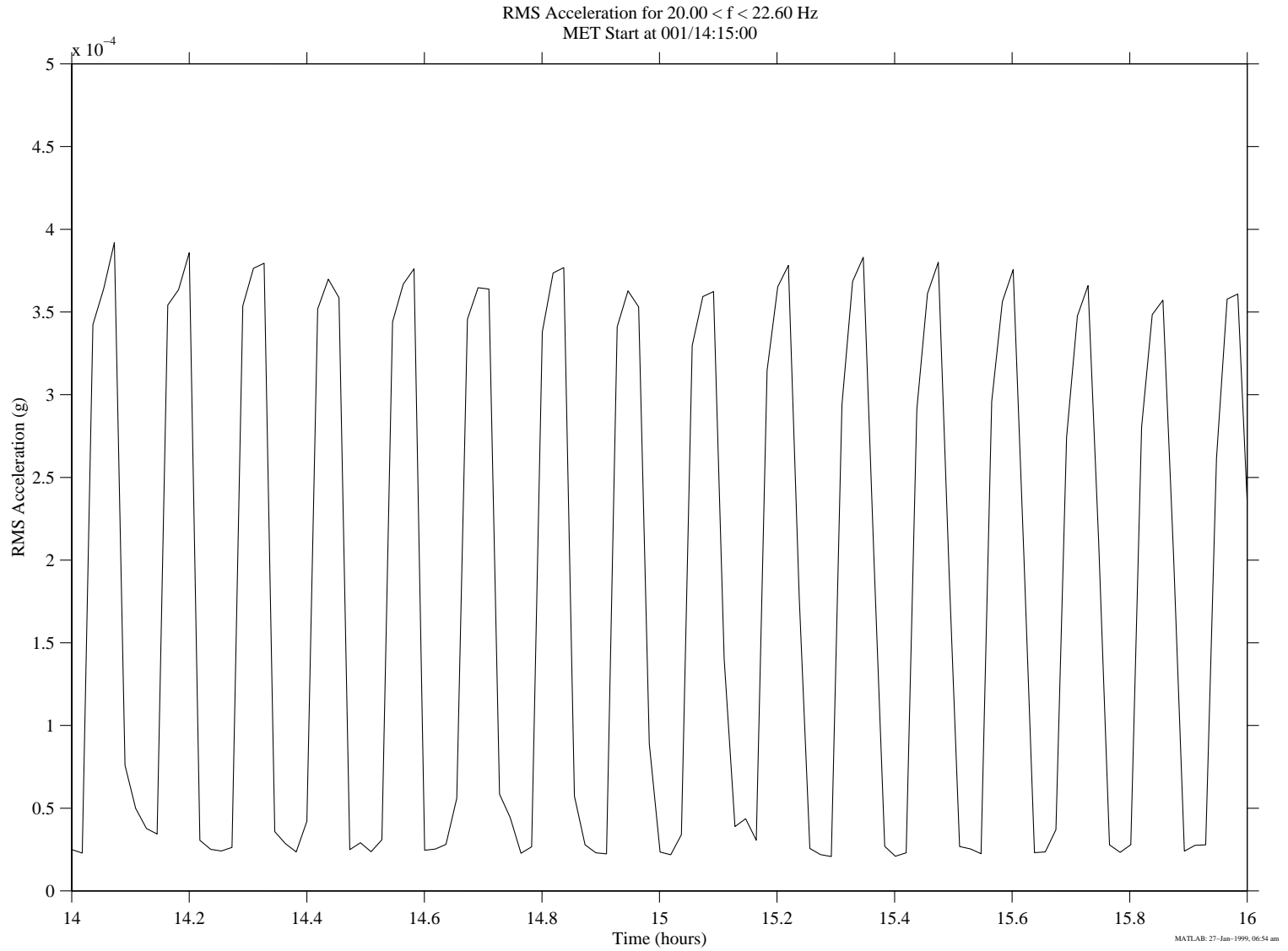
Figure 10. RMS Acceleration Versus Time Zoom ( 20 < f < 22.6 Hz), Orbiter SAMS TSH A
