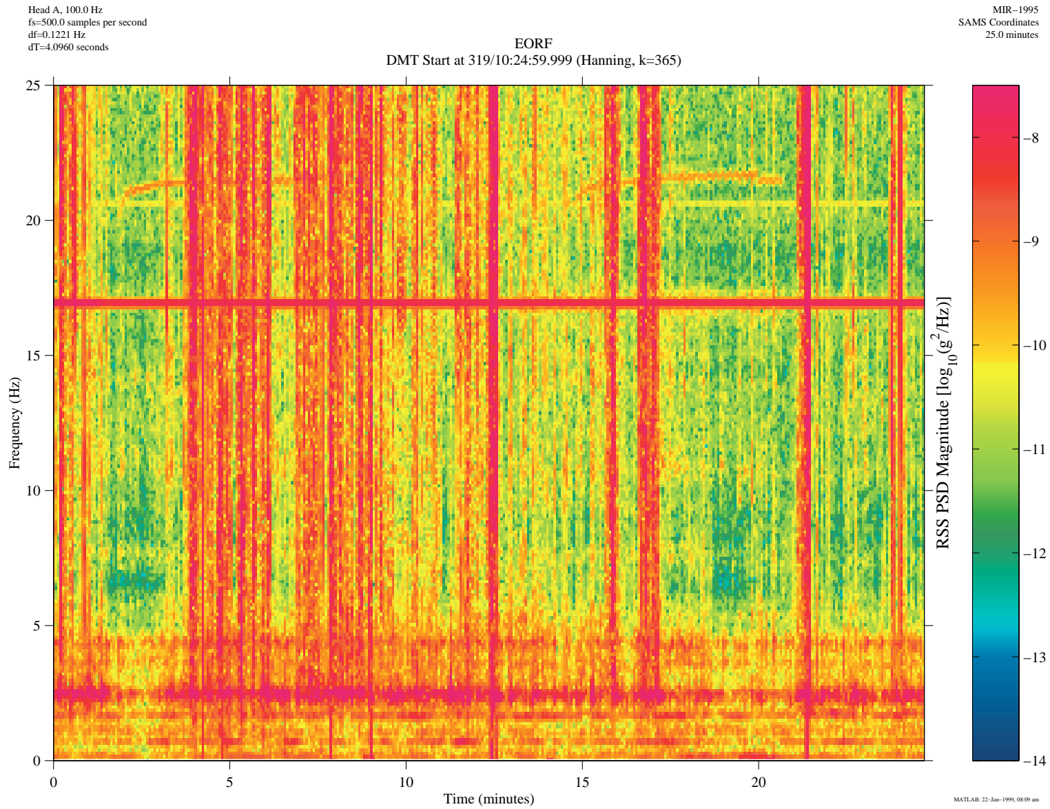
Figure 6. Spectrogram Featuring EORF Signature, Mir SAMS TSH A (1995)
