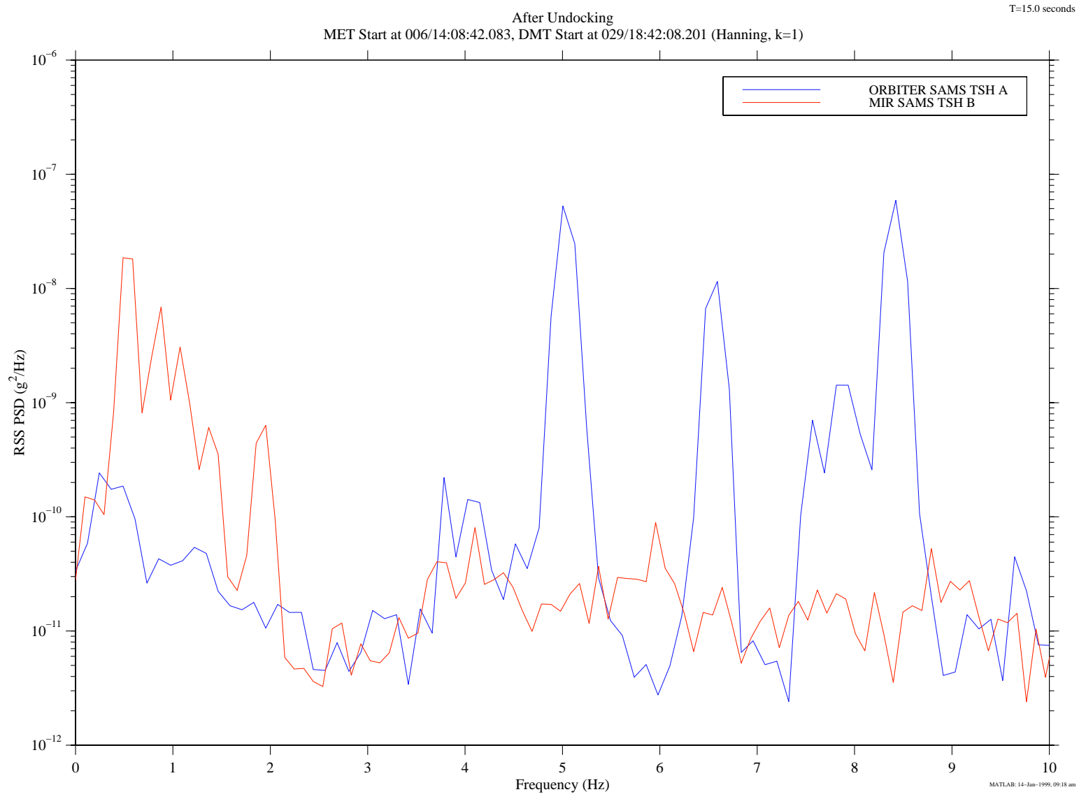
Figure 22. Power Spectral Densities After Undocking
