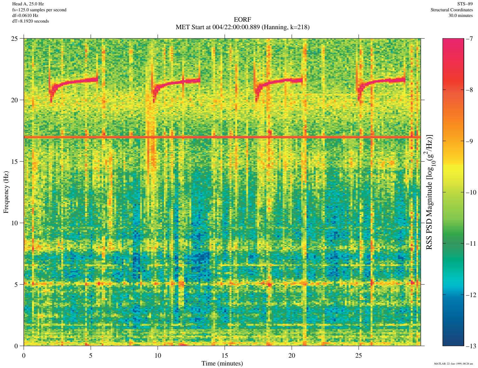
Figure 7. Spectrogram Featuring EORF Signature, STS-89 SAMS TSH A
