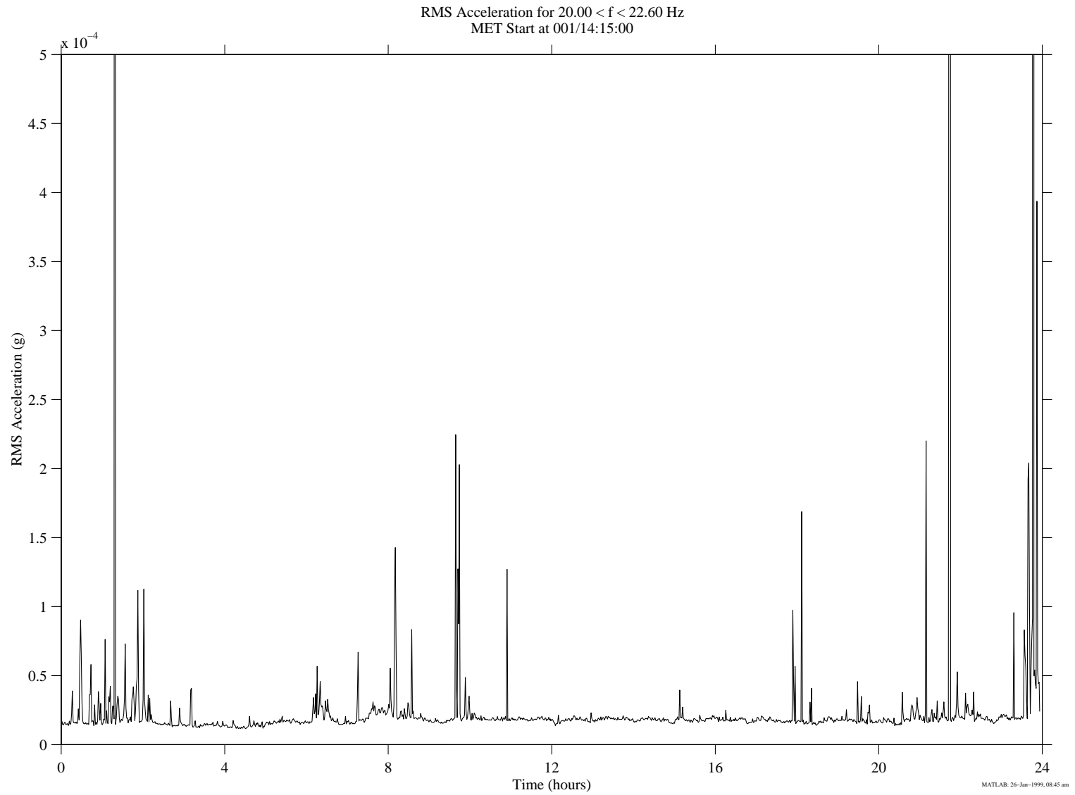
Figure 12. RMS Acceleration Versus Time ( 20 < f < 22.6 Hz), Mir SAMS TSH A
