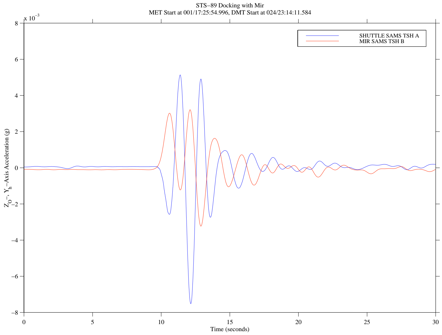
Figure 13. Acceleration Versus Time, STS-89 Docking with Mir
