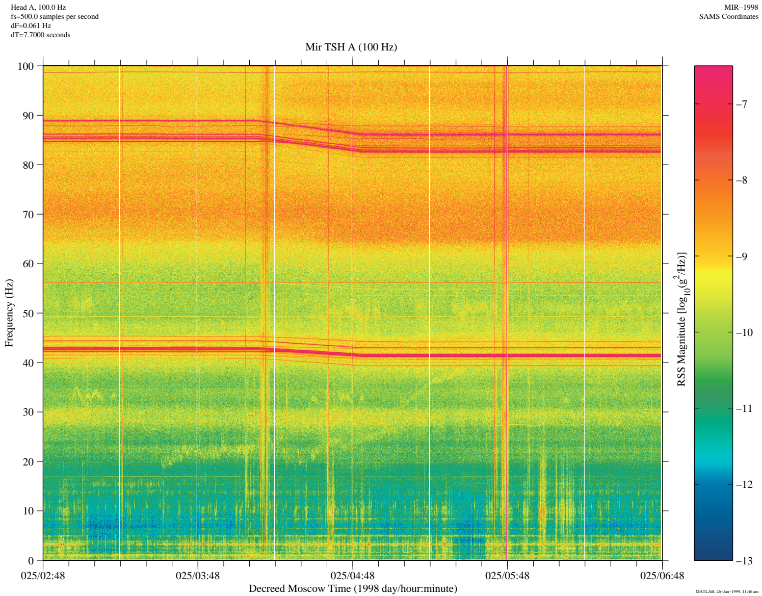
Figure 4. Spectrogram Featuring Mir Life-Support Equipment, Mir SAMS TSH A
