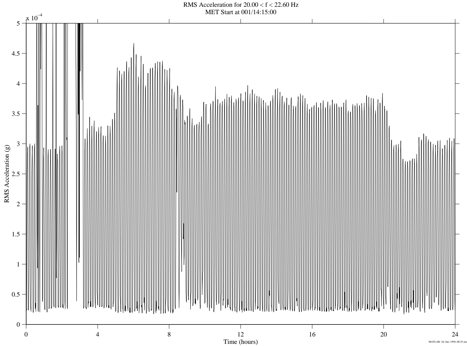
Figure 9. RMS Acceleration Versus Time ( 20 < f < 22.6 Hz), Orbiter SAMS TSH A
