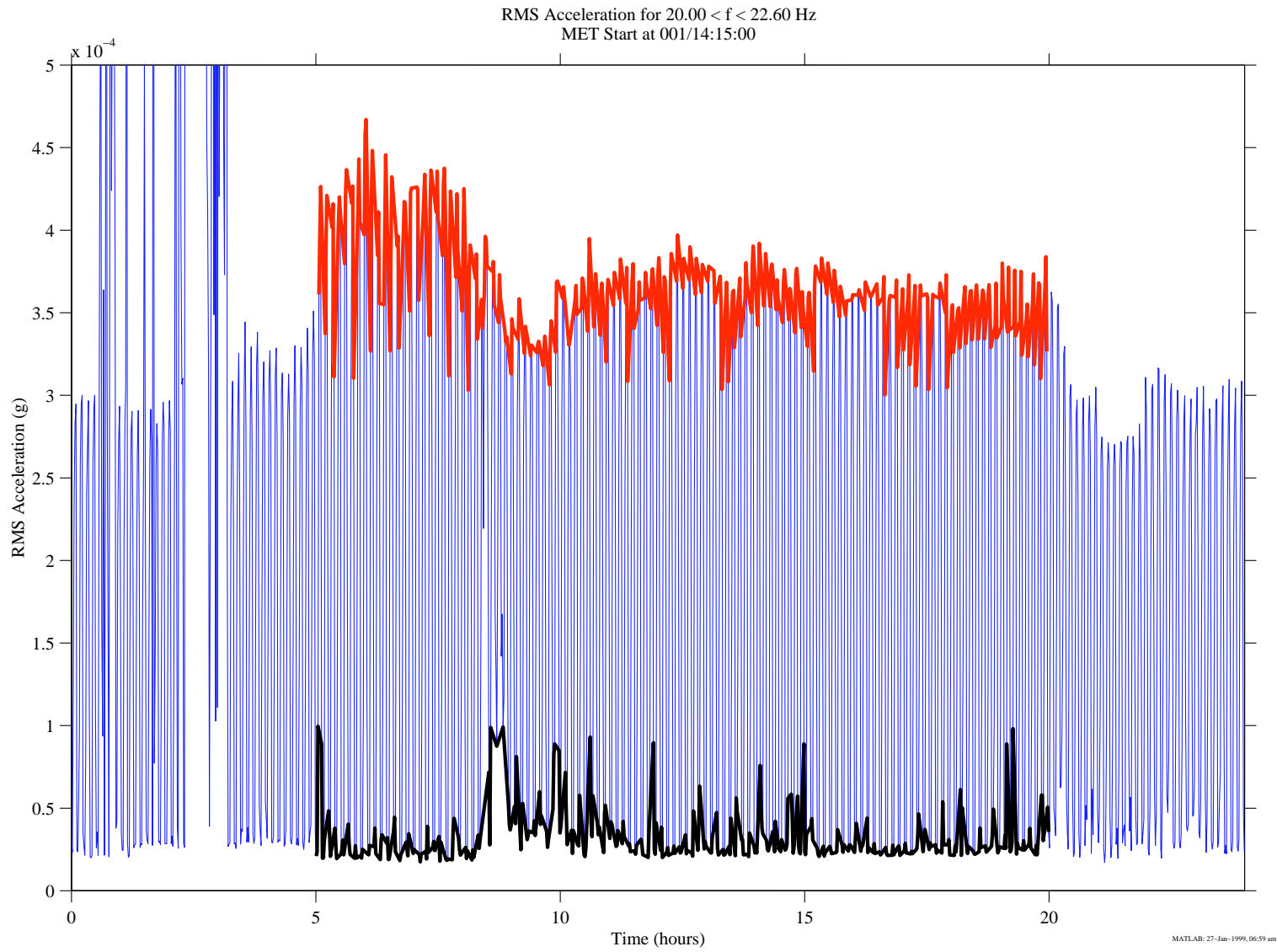
Figure 11. RMS Acceleration Versus Time for EORF Disturbance, Orbiter SAMS TSH A
