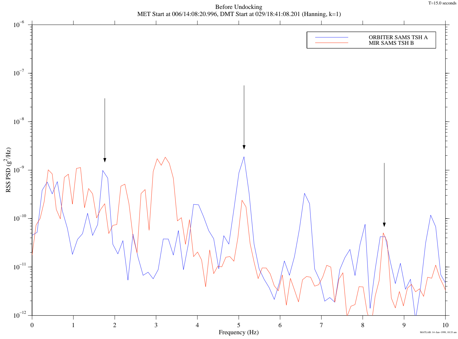
Figure 21. Power Spectral Densities Before Undocking
