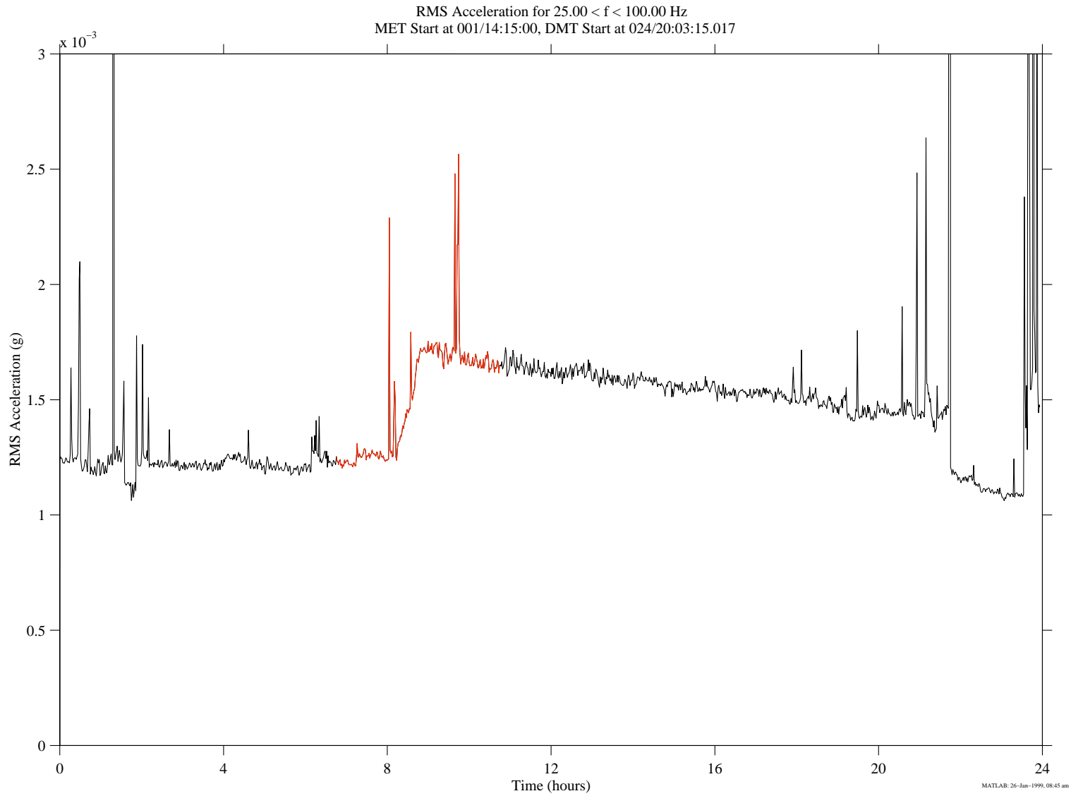
Figure 3. RMS Acceleration Versus Time (25 < f < 100 Hz), Mir SAMS TSH A
