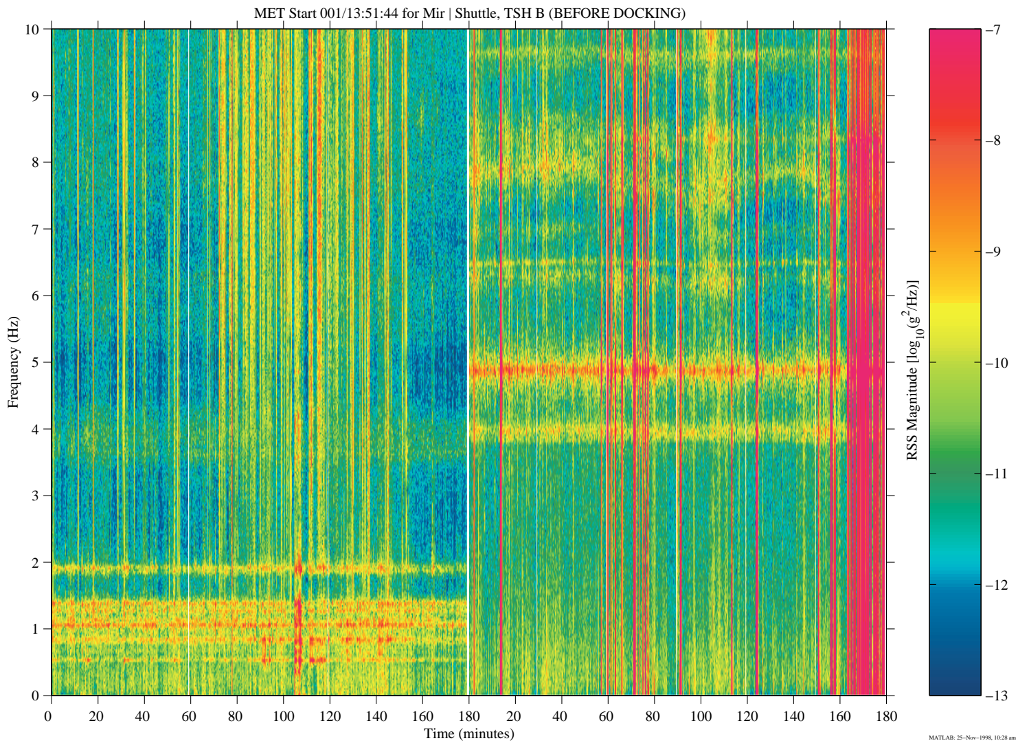
Figure 25. Spectrogram Overlay Before Docking
