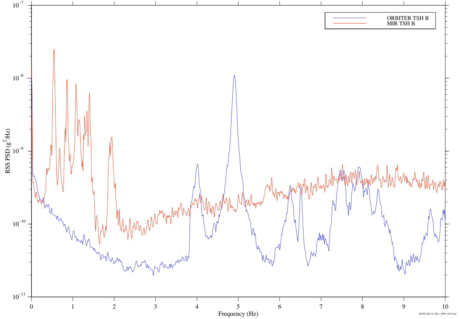
Figure 26. Power Spectral Densities Before Docking
