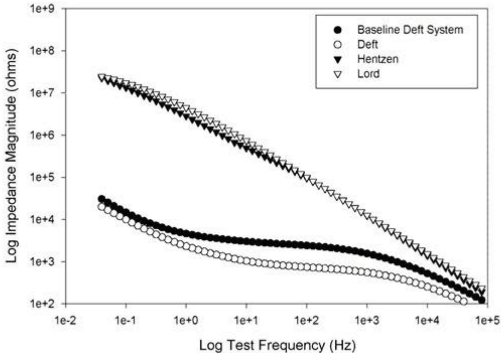
Figure 1. Magnitude for Chemidize 727 With Primer Candidates 672 Hour Exposure EIS Results for Total Coating System With Chemidize 727A Pretreatment Normalized by coating thickness
