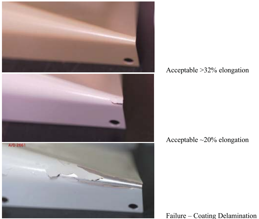
Figure 2. Mandrel Bend Coating Failure
