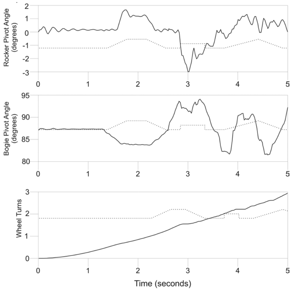
Figure 2. Simulated telemetry showing rocker and bogie pivot angles as function of time during the rolling experiment with MER-like vehicle. The number of wheel turns for the rear wheel is shown on the bottom panel. The topography encountered beneath the center of the rover is shown as a dotted line for the top two panels. For the bottom panel, the topography is shown beneath the center of the rear wheel. The compressed topographic profile with the increasing time is due to rover acceleration. Note that this simulation is the first step toward making a fully MER-like model with powered and steerable wheels. For the simulation shown, the wheel resisting torques were lowered relative to MER conditions to allow rolling on an 8 degree slope.
