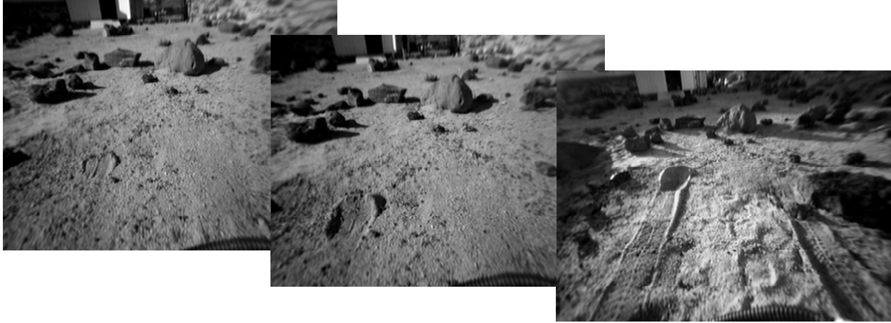
Figure 3. FIDO created a trench in loose sand with front left drive wheel by holding 5 wheels fixed and rotating the front wheel in reverse by ~6 wheel revs. Rover approached site and trenched, backed off and imaged trench, approached site again and trenched, backed off and imaged trench, approached site again and trenched twice (motor stalled on second trench attempt), backed off and imaged trench. Final trench was 7-8 cm deep.
