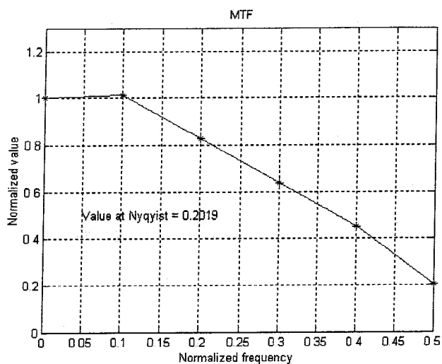
Figure 8d. MTF plot
