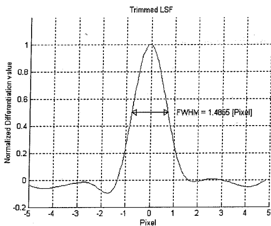
Figure 6c. LSF for Lot 1 – Green Band, Scene 1
