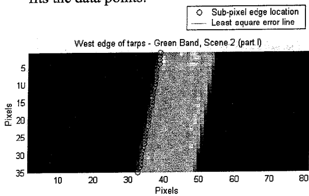
Figure 9a. Tarp west edge - Green Band, Scene 2
