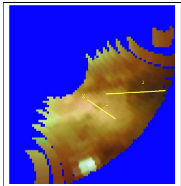
Figure 2. Orthographic projection of VIMS color mosaic at three wavelengths. Points 1 and 2 are the location of circular regions investigated with photometric profiles. We conclude that the photometric properties are not consistent with depressions but they may be palimpsests or penpalimpsests remaining from past impacts.
