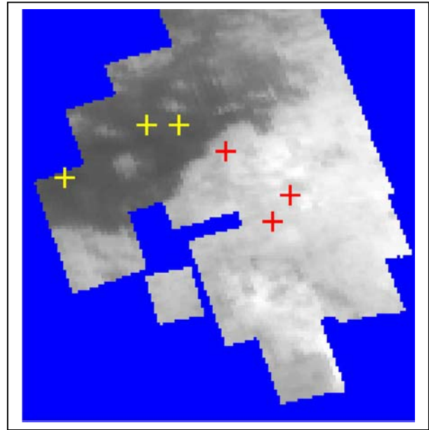
Figure 1. Orthographic projection of VIMS mosaic at 2.02 microns. Location of preliminary photometric control points used in this study. These were used to make the preliminary determination that Titan's regolith is backscattering.
