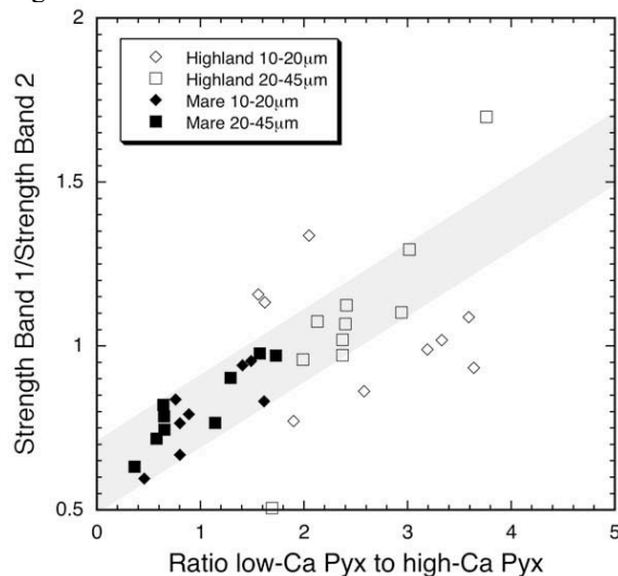
Figure 2. Ratio of low-Ca to high-Ca pyroxene compared to the ratio of a) the band strength of band 1 vs. band 2 and b) the band strength of band 5 vs. band 6.
