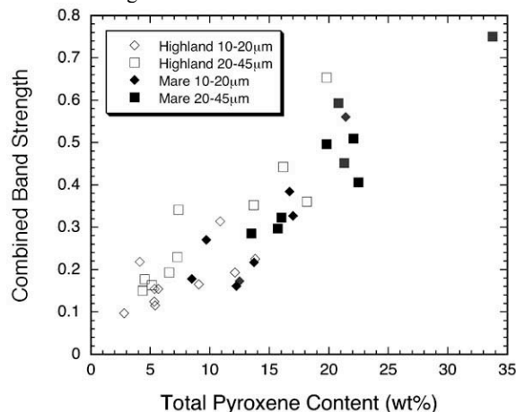
Figure 3. Combined strength of the bands near 1\mu\text{m} compared to the measured pyroxene abundance in the soils.
