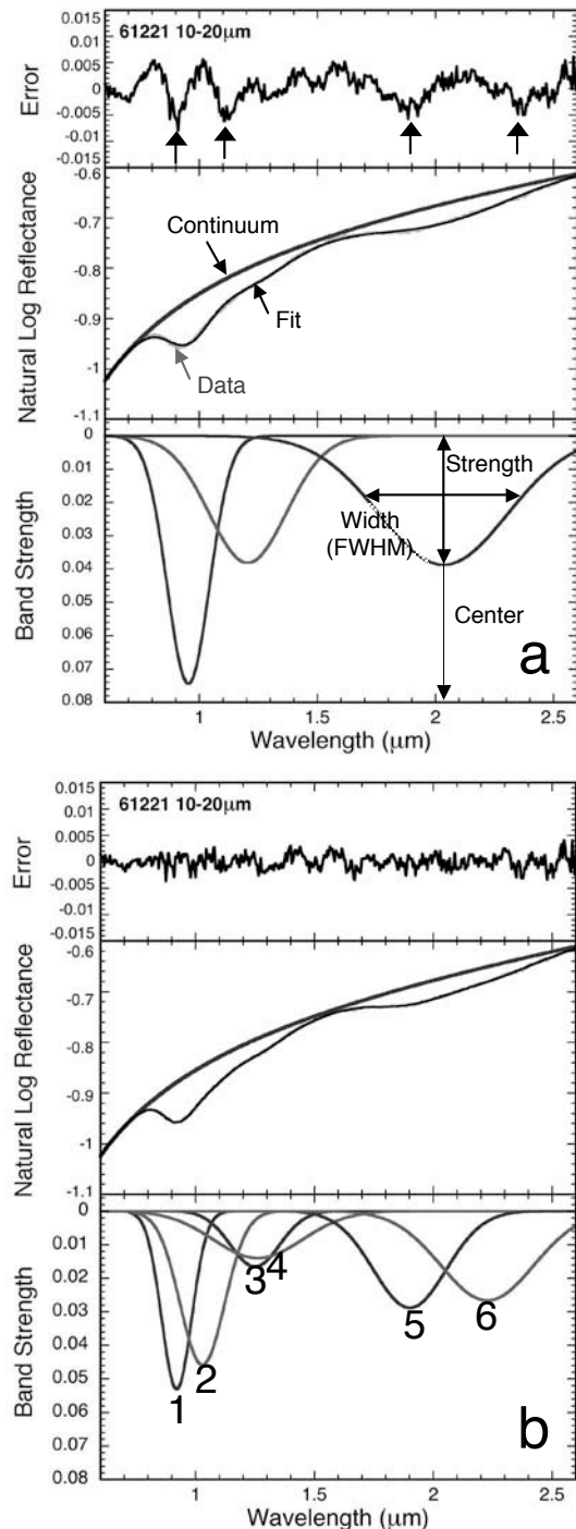
Figure 1. MGM deconvolution results for a representative lunar soil, the 10-20 \mu m fraction of 61221: a=3-band fit, b=6-band fit. The residual in a exhibits systematic errors (arrows) indicating additional bands are required.
