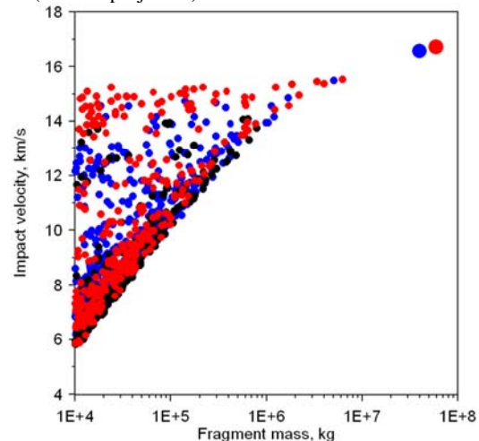
Figure 1: Distribution of final velocity versus mass for fragments larger than 10 4 kg. Variants with one dominant fragment and final velocity of 16 km/s ("strong" projectile) are shown in red and blue. Variants with small fragments and final velocity less than 14 km/s ("weak" projectile) are shown in black.
