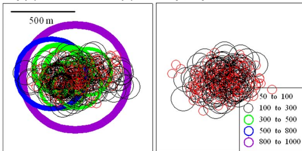
Figure 3: Final. distribution of craters generated by impacting fragments on the surface for two the two main variants (“strong” projectile on the left and “weak” projectile on the right) of figure 2.
