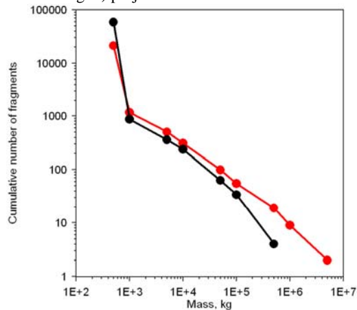
Figure 2: Cumulative number of fragments for the “strong” (red and blue in Fig. 1) and “weak” (black in Fig. 1) projectile cases.
