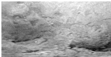
Figure 2. Dark curving lines: river channels in the S. Polar region?
