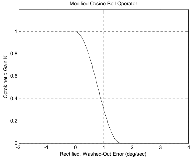
Figure 5.4. Modified Cosine Bell Operator for Optokinetic Gain.
