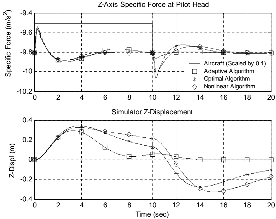
Figure 6.13. Algorithm Responses to Vertical Pulse of 3 m/s 2 Magnitude, 10-Second Duration.
