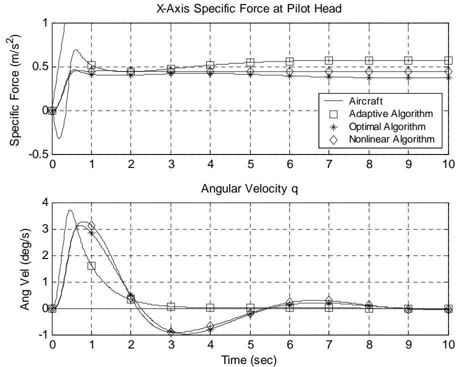
Figure 6.14. Algorithm Responses to Surge Ramp to Step of 1 \text{ m/s}^2 Magnitude, 3 \text{ m/s}^2/\text{s} Slope.
