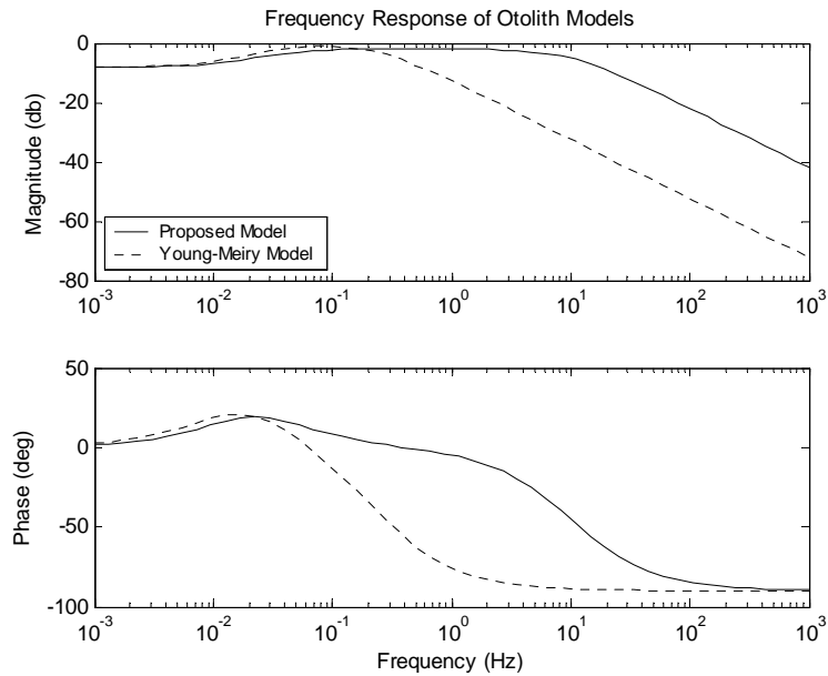
Figure 3.7. Frequency Response of Proposed and Young-Meirly Otolith Models.
