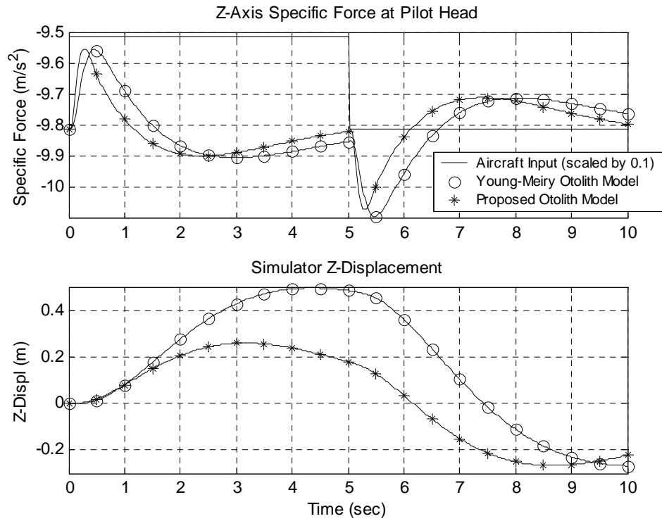
Figure 4.7. Specific Force Responses with Young-Meirly and Proposed Vertical Filters.
