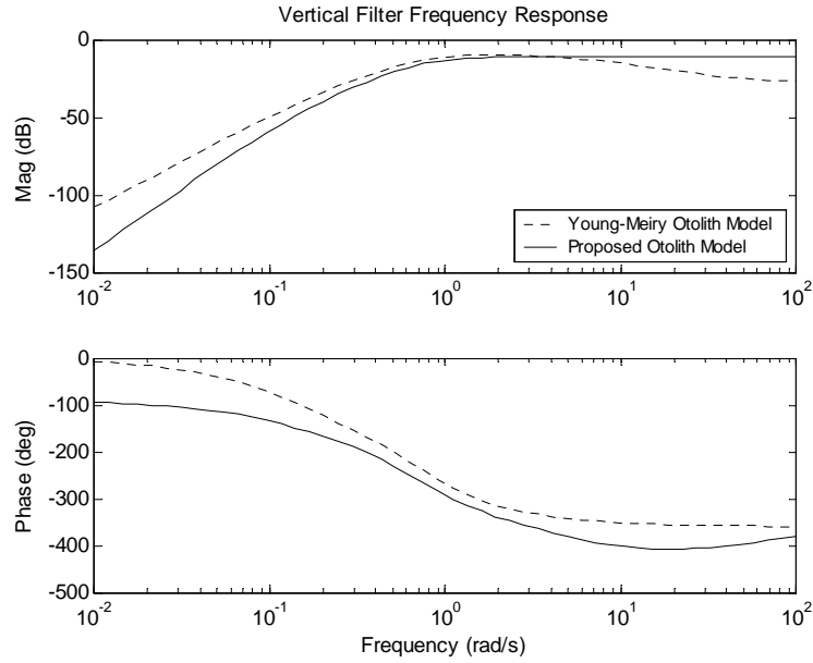
Figure 4.6. Vertical Filter Frequency Responses with Young-Meirly and Proposed Otolith Models.
