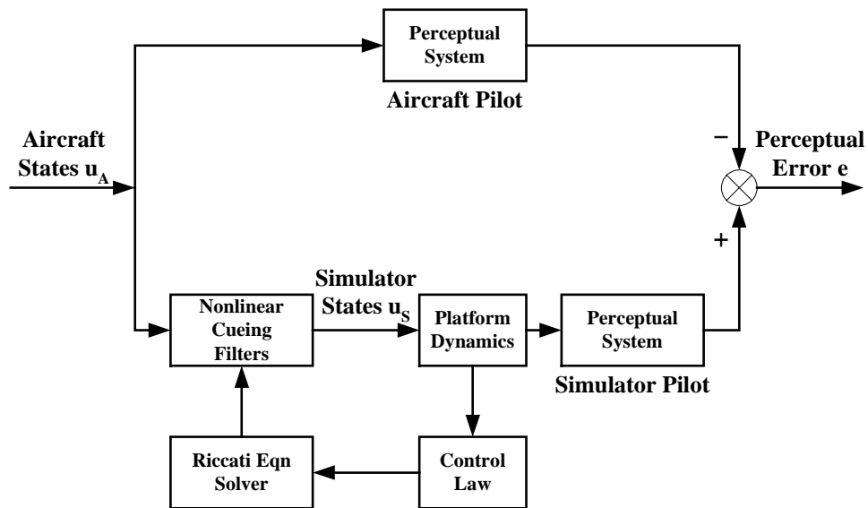
Figure 6.1. Proposed Solution for Nonlinear Motion Cueing Algorithm.
