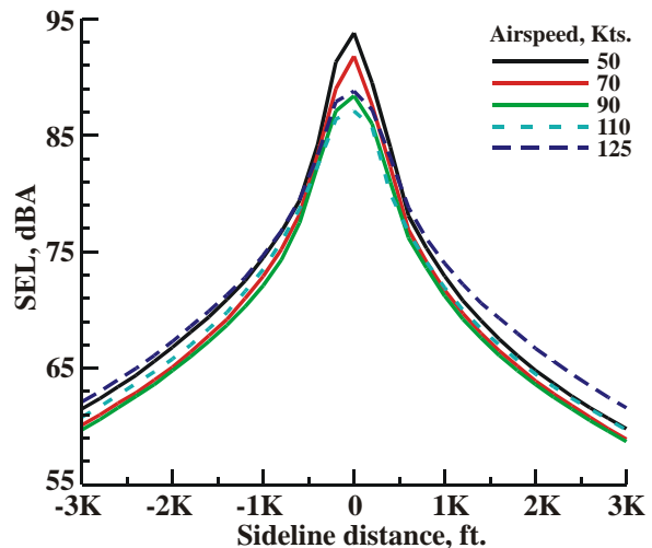
Figure 13. Variation of SEL with sideline distance for airspeeds of 50 to 125 knots; MD600N.
