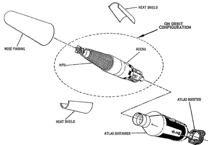
Figure 1. – Configuration of the SNAPSHOT/Agenda D payload and the three pieces of operational debris left on orbit (nose fairing and 2-piece heat shield).
