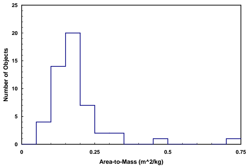
Figure 4. – Area-to-mass histogram of cataloged SNAPSHOT debris.
