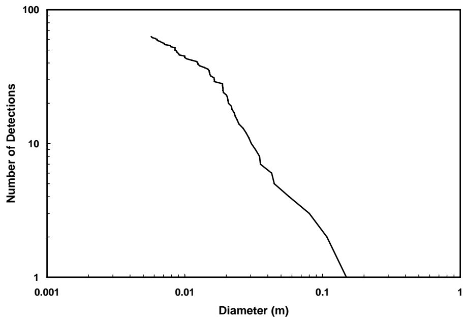
Figure 7. – Size distribution of Haystack detections determined to be SNAPSHOT debris.
