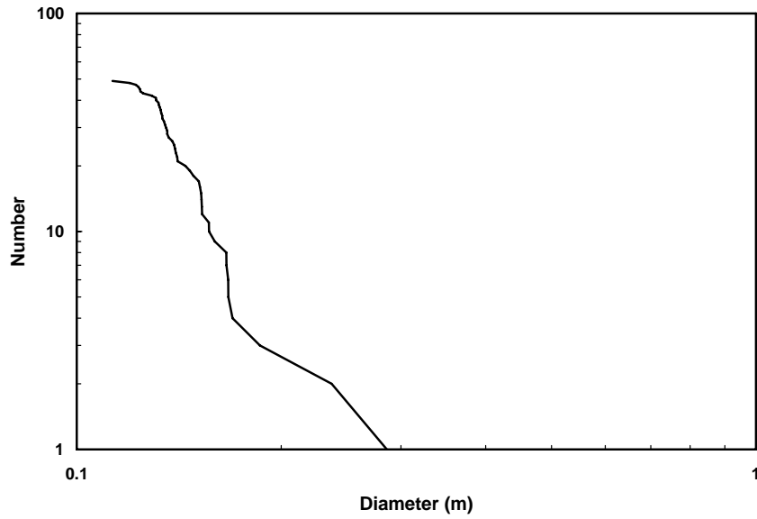
Figure 3. – Size distribution of cataloged SNAPSHOT debris. Size is estimated using the NASA Size Estimation Model.
