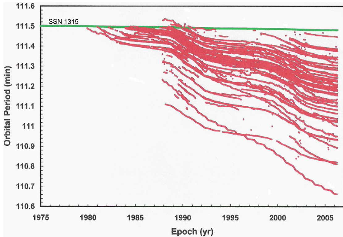
Figure 2. – Orbit period for SNAPSHOT (SSN1315) and associated cataloged debris.
