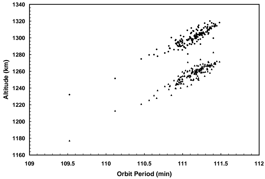
Figure 5. – Gabbard diagram of all SNAPSHOT debris tracked in May 2006 including both cataloged and analyst objects.
