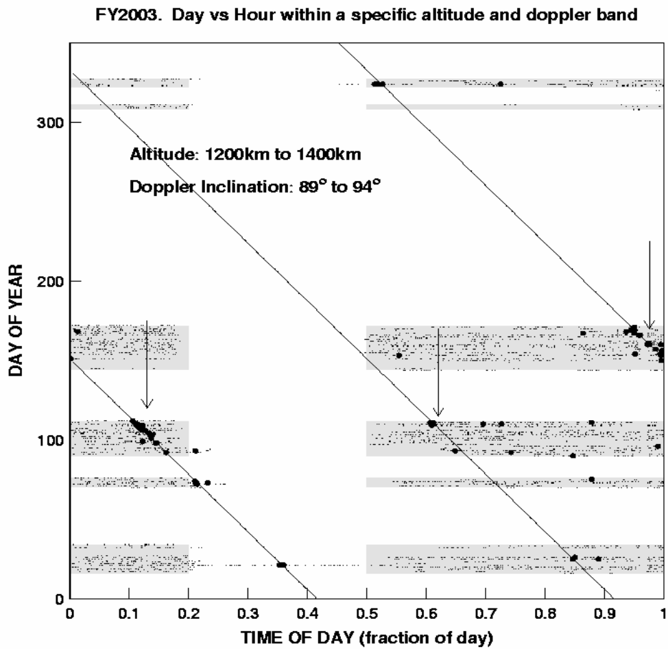
Figure 6. – Diagram showing time of day of all detections (small dots) and detections 1200-1400 km and inclinations 89°-94°. The diagonal lines show the time of orbit plane passage of SNAPSHOT.
