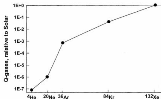
Figure 2. Elemental abundance of Q-gases relative to solar abundance of 132 Xe, as a function of mass. Adapted from Hohenberg et al. [6].
