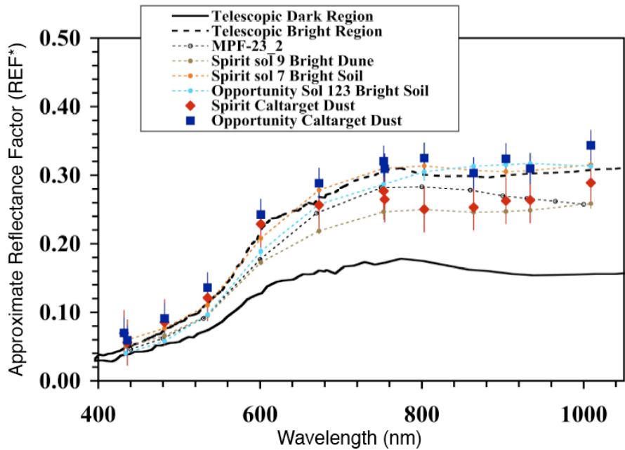
Figure 13.9. Model-derived visible to near-IR spectra of airfall dust on the Pancam calibration targets compared to Martian dust spectra from other sources (telescopic: Mustard and Bell, 1994; Mars Pathfinder bright soil MPF-23_2: Bell et al. , 2000; MER bright soils: Bell et al. , 2004a,b). Modeling and analysis described in detail in Kinch et al. , 2006.
