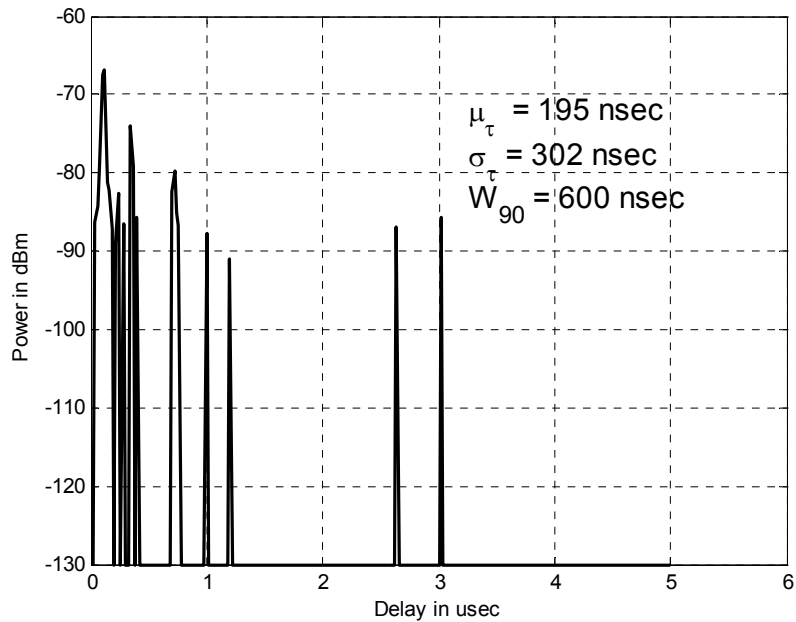
Figure 4.26. Example PDP for JFK, NLOS-S region.
