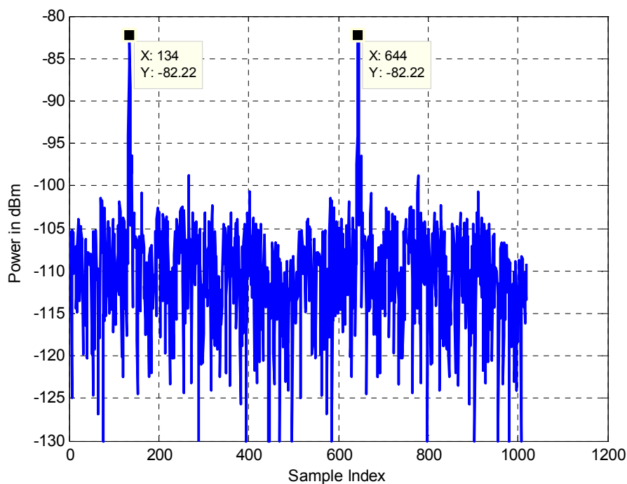
Figure 5.3. Example PowerRecord for 50 Mcps after using Chameleon.
