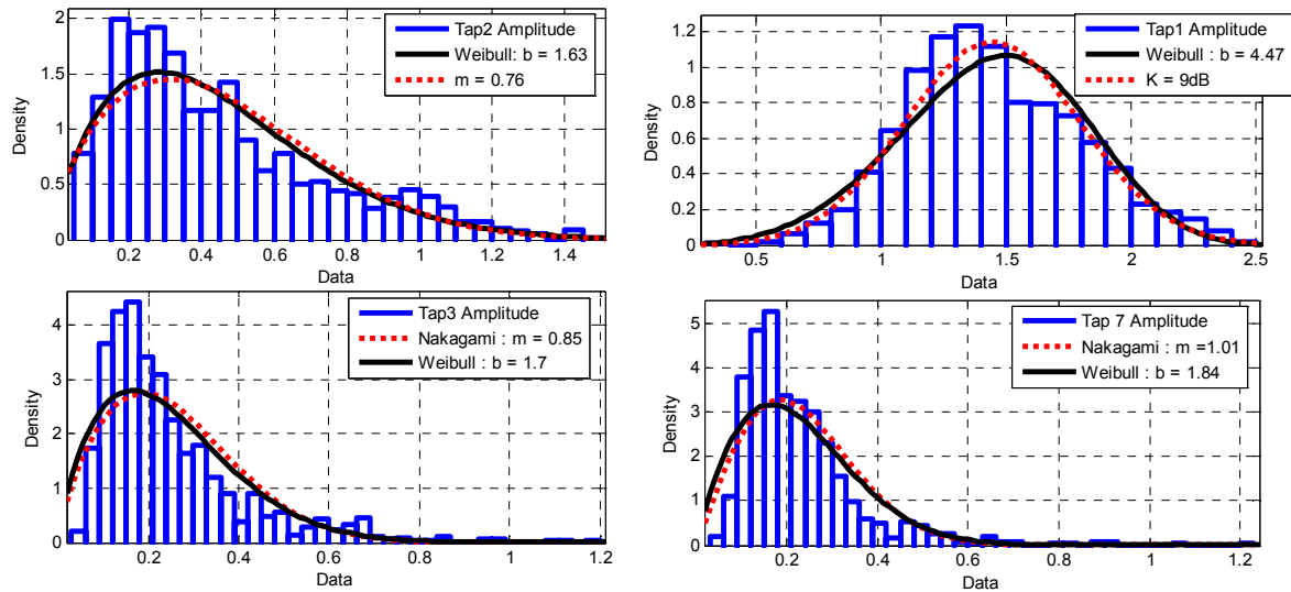
Figure 6.11. Amplitude statistics of taps 1, 2, 3, and 7 for AFS channel [MIA, NLOS-S, 50].
