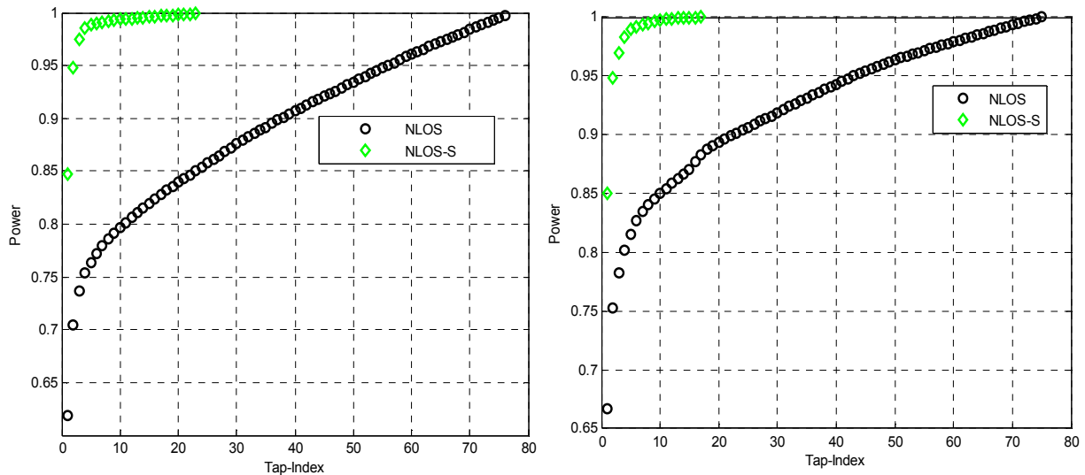
Figure 6.5. Cumulative energy for (a) [MIA 50], and (b) [JFK 50].
