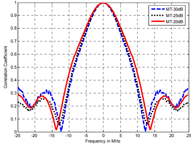
Figure 5.7. Example FCEs for CLE data applying different values of MT .
