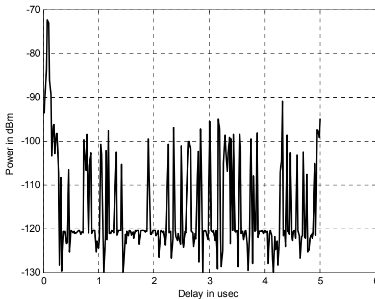
Figure C8. Power-delay profile, in LOS setting at Cleveland airport.
