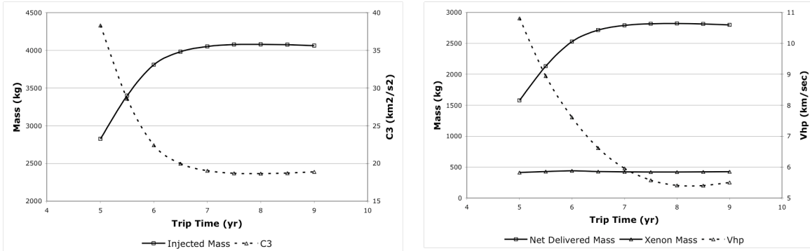
Figure 3. ELV Injection and SEP Module Performance, NEXT 2+1 System, 20 kW Solar Array, Atlas 551 and EGA at 1000 km altitude
