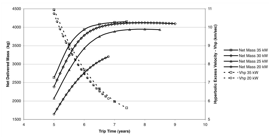
Figure 9. Delivered mass and V_{hp} results at varying array power levels for a NEXT 3+1 configuration, launch on Delta 4050H and an EGA at 1000 km altitude
