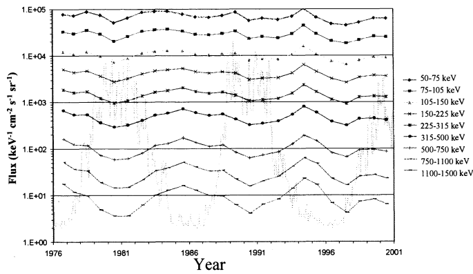
Fig. 32. Electron fluxes at geostationary orbit as a function of the solar cycle.
