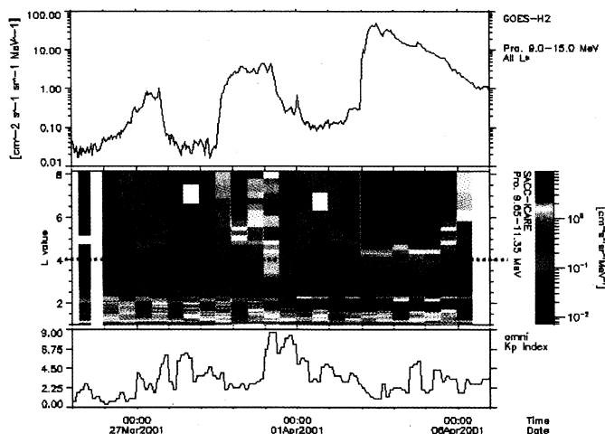
Fig. 39. Top panel: Solar protons observed by GOES-8 at GEO, middle panel: 9.65-11.35 MeV protons measured at LEO onboard SAC-C and bottom panel: Kp index.
