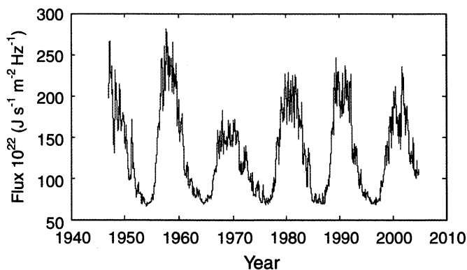
Fig. 2. Measured values of solar 10.7 cm radio flux.
