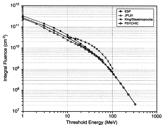
Fig. 16. Comparison of different models of cumulative solar proton event fluence during solar maximum for a 2-year period and the 90% confidence level [45].
