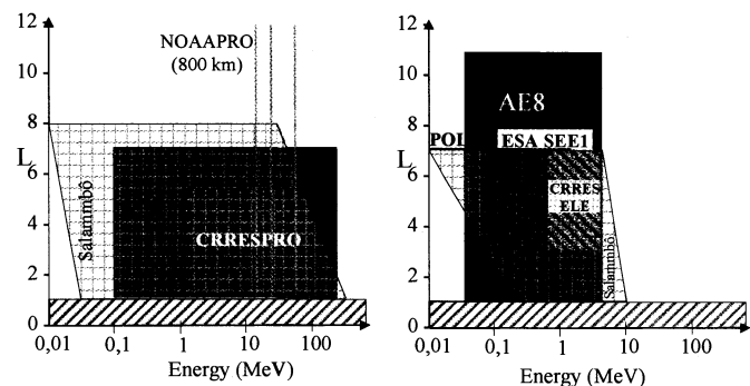
Fig. 43. Validity domain of the radiation belt models
