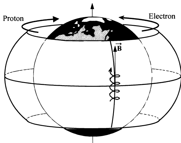
Fig. 26. Composition of a charged particle's three periodic movements: gyration, bounce and drift. The particle then follows a torus surface called a drift shell.
