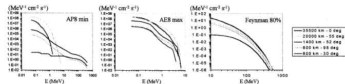
Fig. 45. Omnidirectional differential flux spectrums for trapped protons (AP8 min) on the left, for trapped electrons (AE8 max) in the center and for solar protons (Feynman 80 %) on the right.
