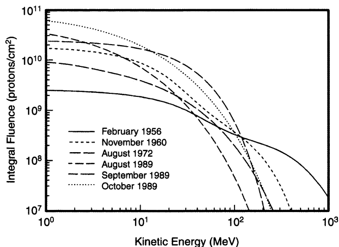
Fig. 17. Some of the most severe solar proton event energy spectra in solar cycles 19-22 [47].
