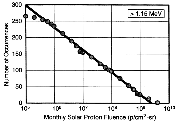
Fig. 12. Integral distribution of monthly solar proton fluences > 1.15 MeV, from 1973 to 2001 [23].
