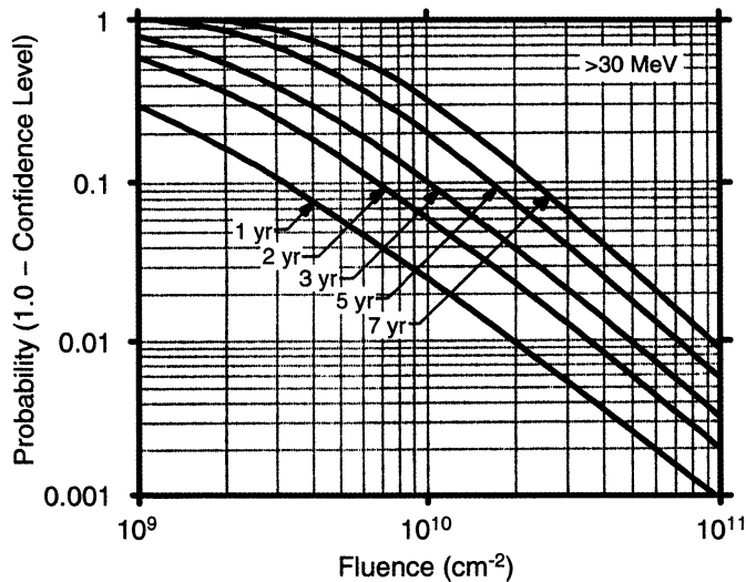
Fig. 14. JPL91 solar proton fluence model for > 30 MeV protons. The misprint of x-axis units has been corrected from the original reference [39].
