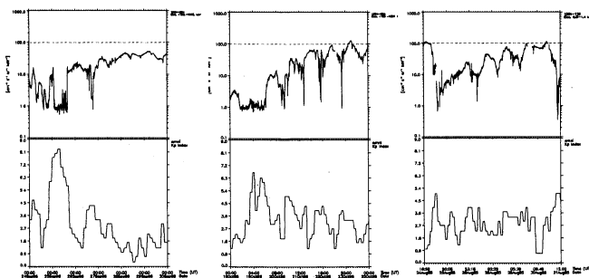
Fig. 36. Comparison of the consequences of three magnetic storms on the fluxes of 1.1-1.5 MeV electrons in geostationary orbit for three different levels of activity
