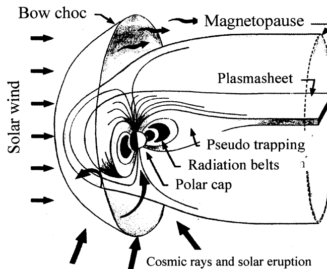
Fig. 23. The Earth's magnetosphere
