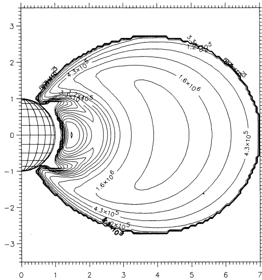
Fig. 28. Electron radiation belt.
