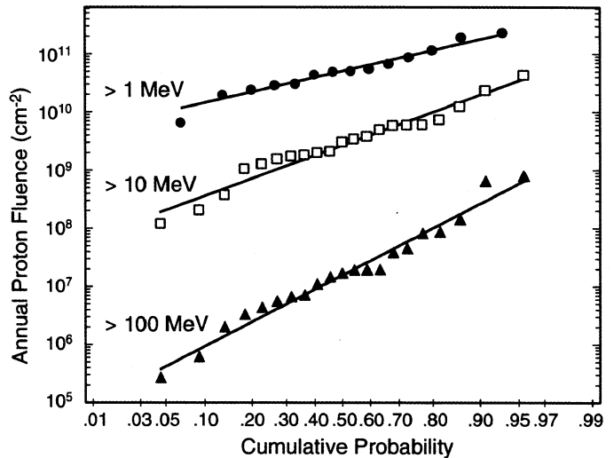
Fig. 15. Cumulative annual solar proton event fluences during solar maximum periods for 3 solar cycles plotted on lognormal probability paper. The straight lines are results for the ESP model [42].
