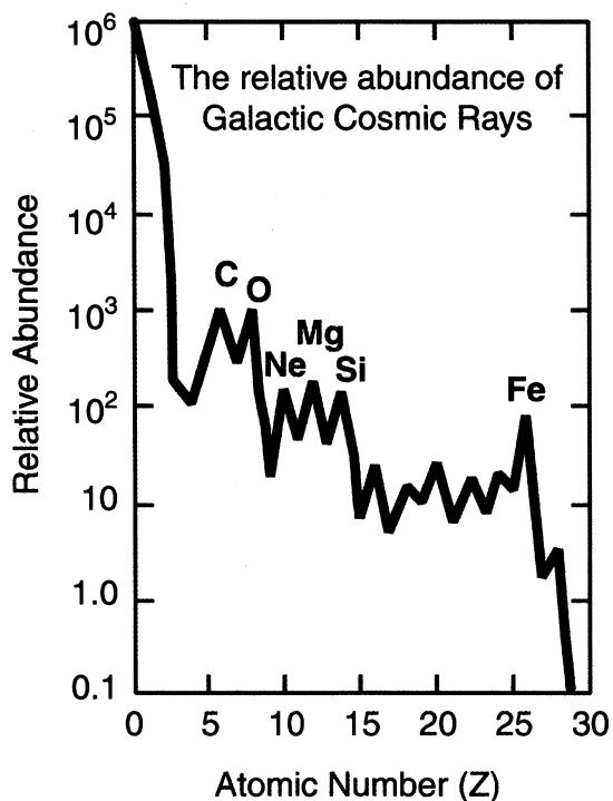
Fig. 4. Abundances of GCR up through Z = 28 .
