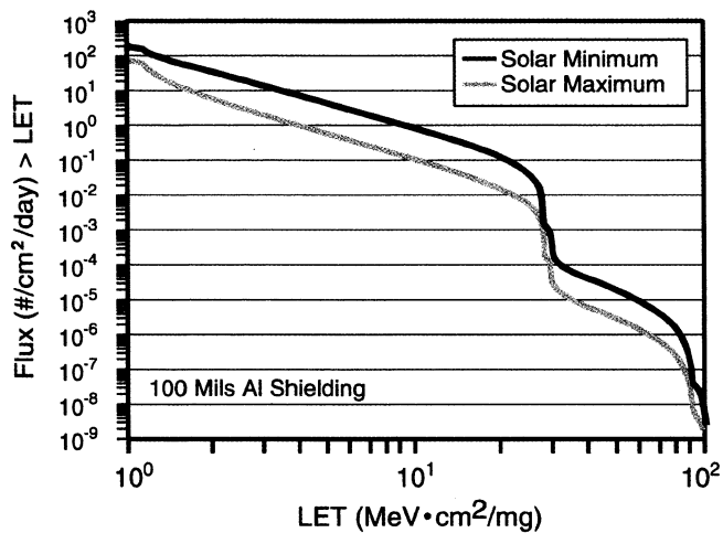
Fig. 6. Integral LET spectra for GCR during solar maximum and solar minimum.
