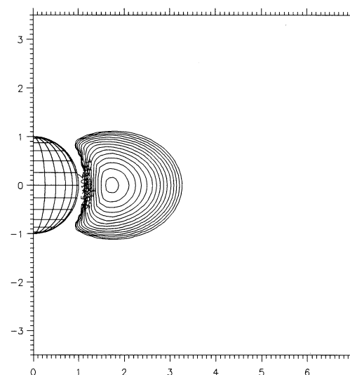
Fig. 27. Proton radiation belt.
