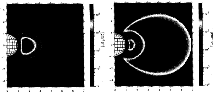
Fig. 41. Omnidirectional integrated fluxes of protons with an energy level higher than 10 MeV (left) and of electrons with an energy level higher than 1 MeV (right).
