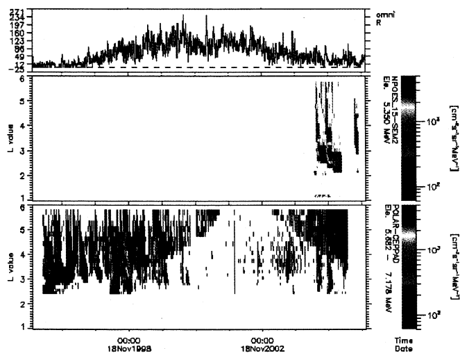
Fig. 38. Top panel: Sunspot number, middle panel: 5.35 MeV electrons measured at LEO onboard NPOES-15 and bottom panel: 5.6-7.1 MeV electrons measured at HEO onboard Polar.
