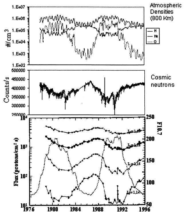
Fig. 31. Changes in the proton fluxes at low altitudes (bottom), in the cosmic radiation (middle) and atmospheric densities (top) as a function of the solar cycle.
