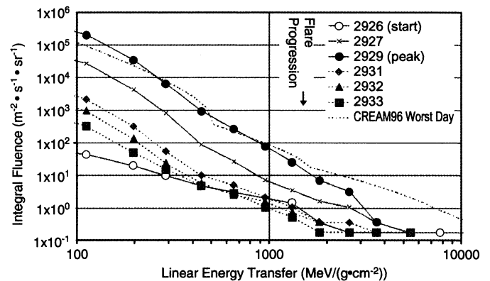
Fig. 21. Comparison of a solar heavy ion event that occurred in November 2001 with the CREME96 “worst day” model. The progression of daily intensities is indicated with the peak intensity occurring on day 2929 of the mission [71].
