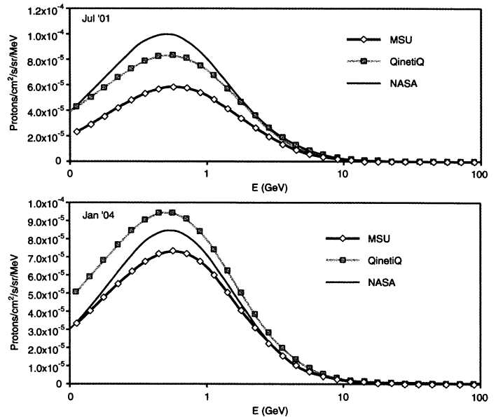
Fig. 7. GCR proton energy spectra predicted by the MSU, Badhwar and O'Neill, and QARM models for two different dates [18].
