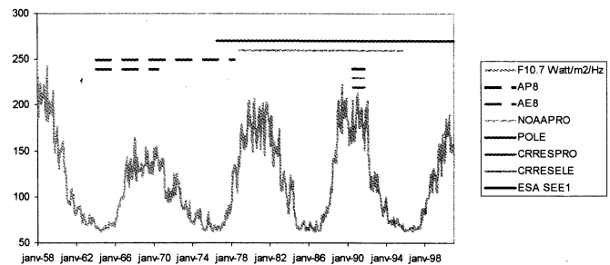
Fig. 42. Coverage of the measurements used to create the various models of radiation belts.
