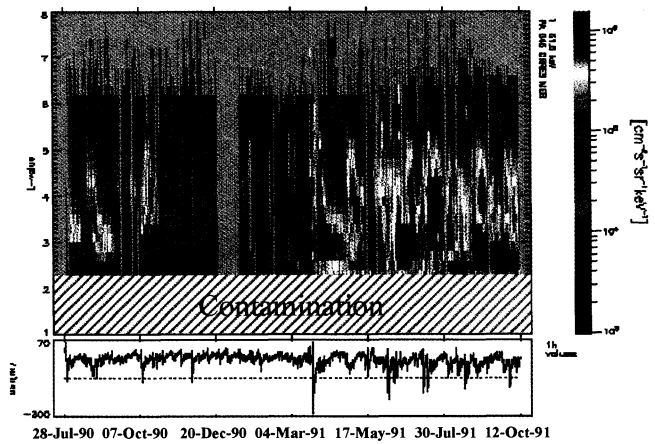
Fig. 33. Flux of 62 keV protons measured by the MEB detector on CRRES for 14 months.
