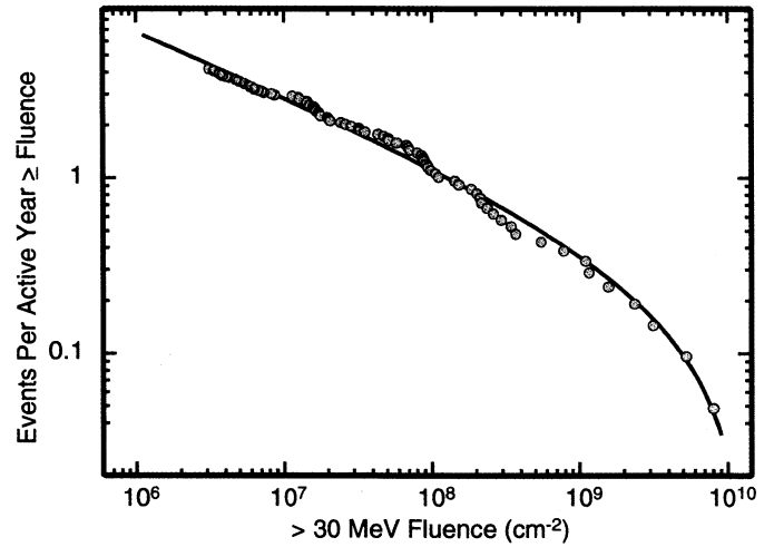
Fig. 13. Comparison of the maximum entropy theory result for the distribution to 3 solar cycles of data during solar maximum [37].
