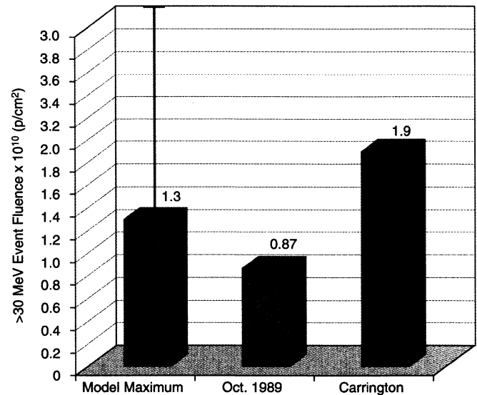
Fig. 19. Comparison of the > 30 MeV solar proton event fluences of the October 1989 event, the 1859 Carrington event as determined from ice core analysis [63], and the model upper limit parameter plus one standard deviation shown by the error bar [37].
