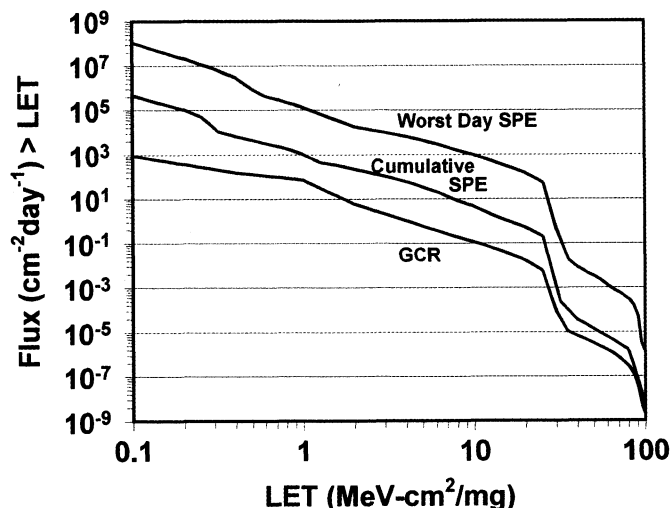
Fig. 22. LET spectra obtained from CREME96 [14] for the “worst day” solar particle event (top curve) and GCR during solar maximum (bottom curve), compared to the cumulative solar particle event flux at the 90% confidence level [65]. All results assume 100 mils of aluminum shielding.
