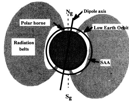
Fig. 29. Environment in low orbit
