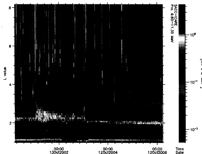
Fig. 40. 9.65-11.35 MeV protons measured at LEO onboard SAC-C.
