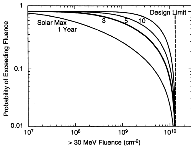
Fig. 19. Probability model for worst-case event fluences expected during the indicated time periods during solar maximum [37].
